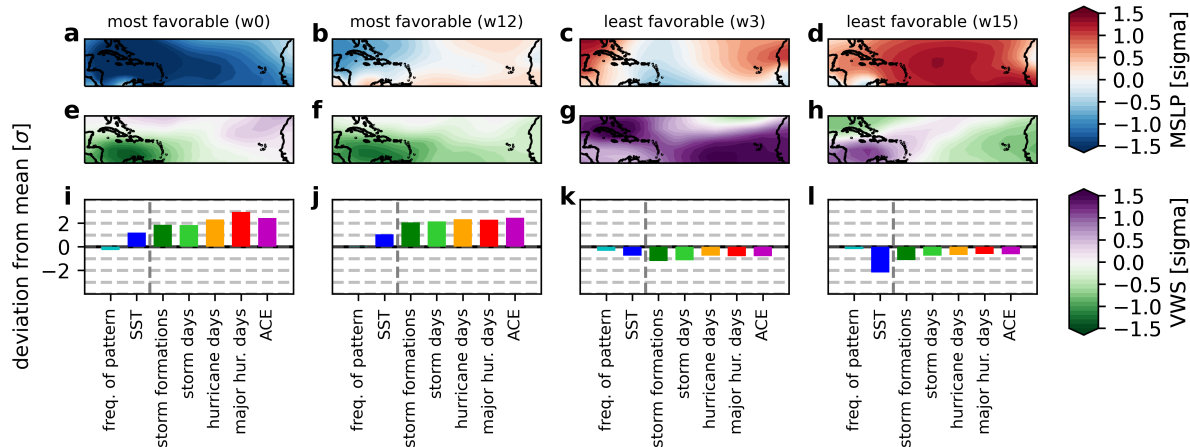
Figure 1. Tropical cyclone activity during selected weather patterns. Mean sea level pressure anomalies (a-d) and vertical wind shear anomalies (e-h) for four selected weather patterns w0, w12, w3 and w15. The last row (i-l) shows relative deviations from the average of all weather patterns expressed in standard deviations for the following statistics: frequency of the weather pattern, SST in the MDR, number of storm formations during the weather pattern, storm days, hurricane days, major hurricane days and average ACE generated during days with this weather pattern. A value of 2 indicates, that the statistic is 2 standard deviations higher during this weather pattern than for the average over all weather patterns. All 20 weather patterns are shown in figures S1, S2, S3
