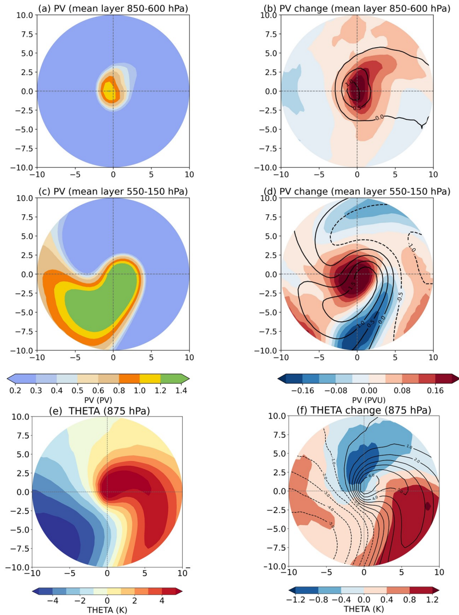
Figure 9. Present-day composites for extreme cyclones of PV averaged over a) the lower troposphere (850-600 hPa), c) the upper troposphere (550-150 hPa) and potential temperature at 875 hPa (lower boundary) for winter in the North Atlantic region. Future changes of the lower tropospheric PV, upper tropospheric PV and potential temperature are shown in b, d, and f respectively. The present-day mean of each field is overlaid as black contour lines in b, d and f. The composites are shown at the time of maximum intensity (time=0).
