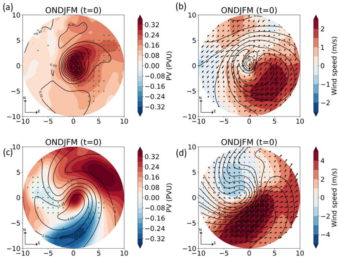
Figure 8. Future change in composites for extreme cyclones of a) PV at 700 hPa, b) wind speed at 850 hPa, c) PV at 250 hPa and d) wind speed at 250 hPa for winter in the North Atlantic region. The present-day mean of each field is overlaid as black contour lines. Green dots denote regions of ensemble agreement on the sign of change, i.e., more than 80% of the ensemble members indicate a future change of the same sign. The composites are shown at the time of maximum intensity (time=0). Extreme cyclones are defined as the 1% strongest systems in terms of maximum RV850.
