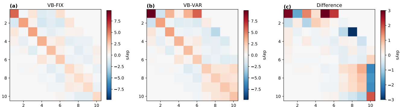
Figure B1. Response matrices \hat{L} calculated from the barotropic setups using Eq. (B5) but for practical purposes with an upper integration limit of 40 days (a) VB-FIX (b) and VB-VAR. These are the \hat{L} matrices used to make the predictions in Fig. 6, shown here in their respective EOF bases. (c) Difference between (a) and (b) in the EOF basis of the OFF control experiment, highlighting the impact of interannual VB variability.
