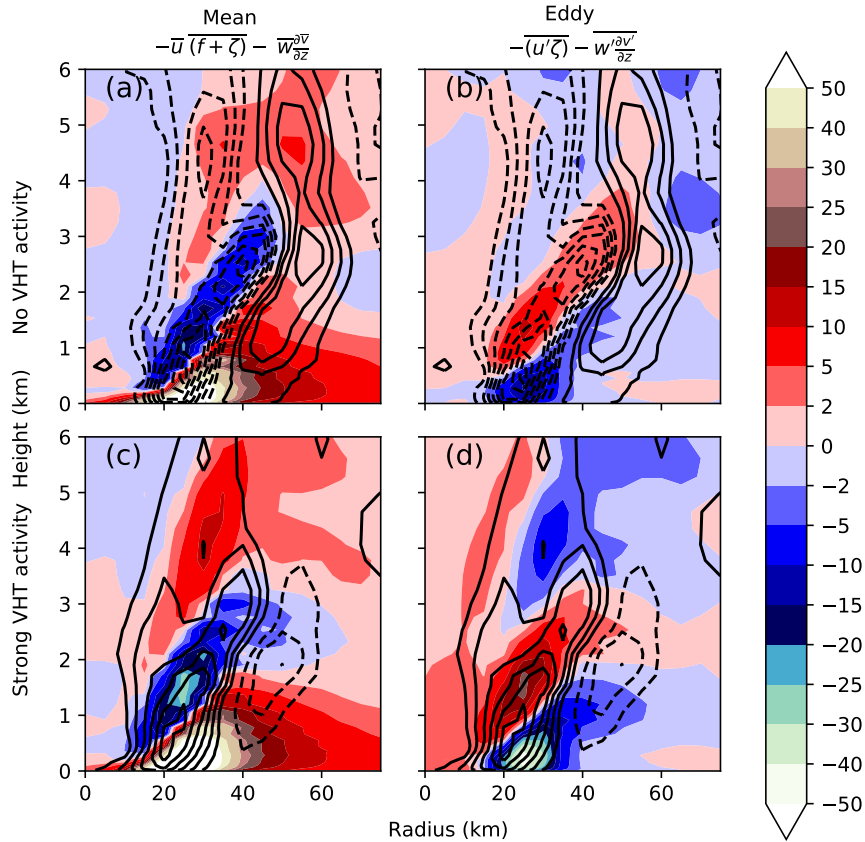
Figure 11. As with Fig. 10 but this time composites of no VHT activity (top row) and strong VHT activity (at least one VHT-like structure with ascent shading perturbation vertical velocity above 2 \text{ m s}^{-1} and perturbation relative vorticity contours above 10^3 \text{ s}^{-1} at all three levels as in Fig. 9; bottom row). Composites are created by averaging any times in the W1 and S1 combined period with no distinction between weakening and strengthening periods (45.5 hours to 57.5 hours) that either have no VHT activity (top row) or strong VHT activity (bottom row).
