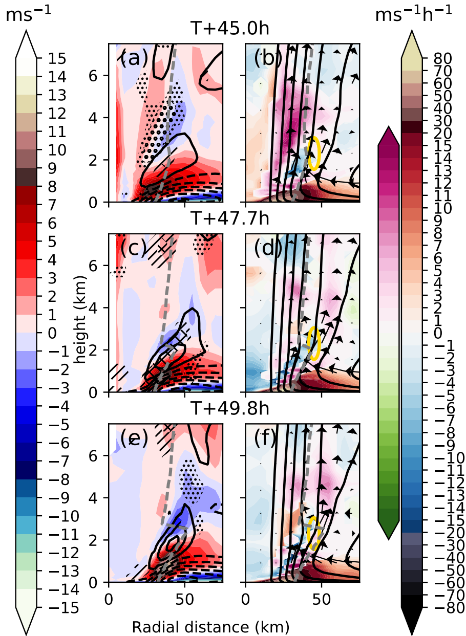
Figure 15. Left column shows, as a function of height and radius: the gradient wind (shading, \text{ms}^{-1} left colourbar), the radial wind in intervals of 4 \text{ms}^{-1} with dashed lines indicating negative values, the tendency in tangential wind as small dots showing +2 \text{ms}^{-1}\text{h}^{-1} \text{ms}^{-1}\text{h}^{-1} , large dots showing +4 \text{ms}^{-1}\text{h}^{-1} \text{ms}^{-1}\text{h}^{-1} , line hatches showing -2 \text{ms}^{-1}\text{h}^{-1} \text{ms}^{-1}\text{h}^{-1} and cross hatches showing -4 \text{ms}^{-1}\text{h}^{-1} \text{ms}^{-1}\text{h}^{-1} . Right column shows angular momentum (lines in units of 5 \times 10^{-5} \text{m}^2 \text{s}^{-1} ) and the secondary circulation as arrows in the plane of the cross section (with the boundary layer strong inflow omitted for clarity). The shading shows the contribution of the sum of the radial and vertical advection of angular momentum to the tangential wind budget. The colour scale used indicates which is the dominant term. If radial advection dominates over vertical advection then the blue/red shading is used and if vertical advection is dominant over radial advection then the green/purple scheme is used. For example green shading implies that the radial and vertical advection of angular momentum causes a negative tangential wind tendency and that the vertical term dominates. Also shown is RMW as the dashed grey line. The times shown in (a,b) are T+45 h, (c,d) T+47.4 h, and (e,f) T+49.8 h (the first three panels in Fig. 9). A region of interest is denoted
