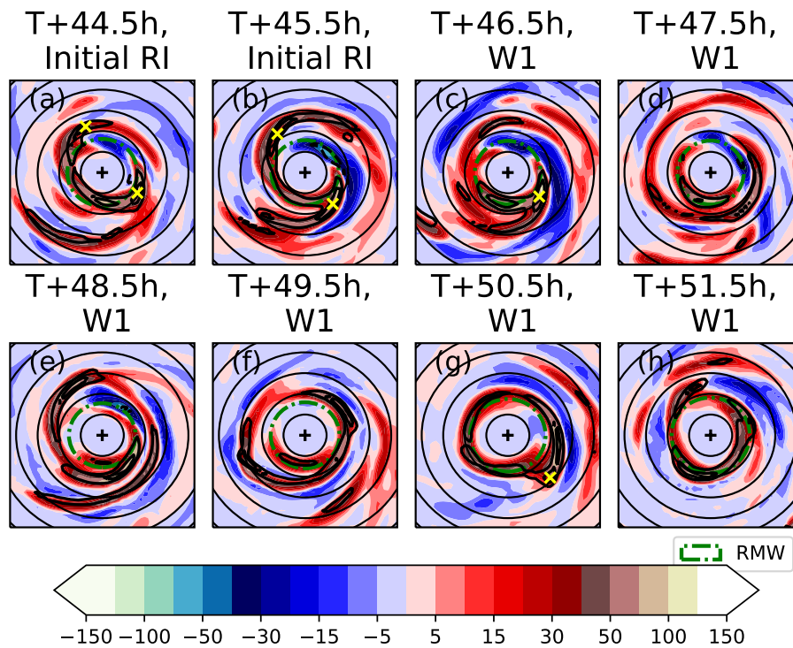
Figure 13. Diabatic heating ( \text{K h}^{-1} shading) for height 4963 m before and during the first weakening phase W1. Vertical velocity contours in intervals of 2 \text{ m s}^{-1} . Yellow crosses indicate the location of the maximum local perturbation vertical velocity at the same level for any VHT-like structures as determined by criteria adapted from Smith and Eastin (2010).
