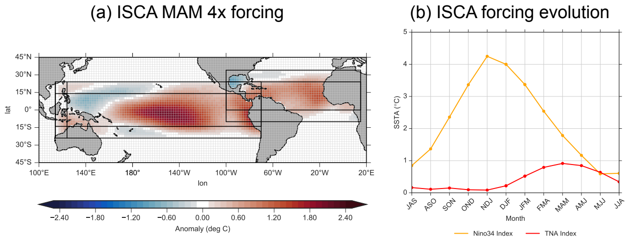
Figure 1. Forcing areas and seasonal evolution used to force ISCA. (a) depicts March-May (MAM) SST forcing for the AP runs (combined Pacific and Atlantic forcing). Black outlines indicate areas where regression was used, with outside rectangles indicating transition areas of linear decrease (see S1 for percentages). (b) shows the seasonal evolution of Niño3.4 (orange) and TNA (red) indices using a 3-month running mean.
