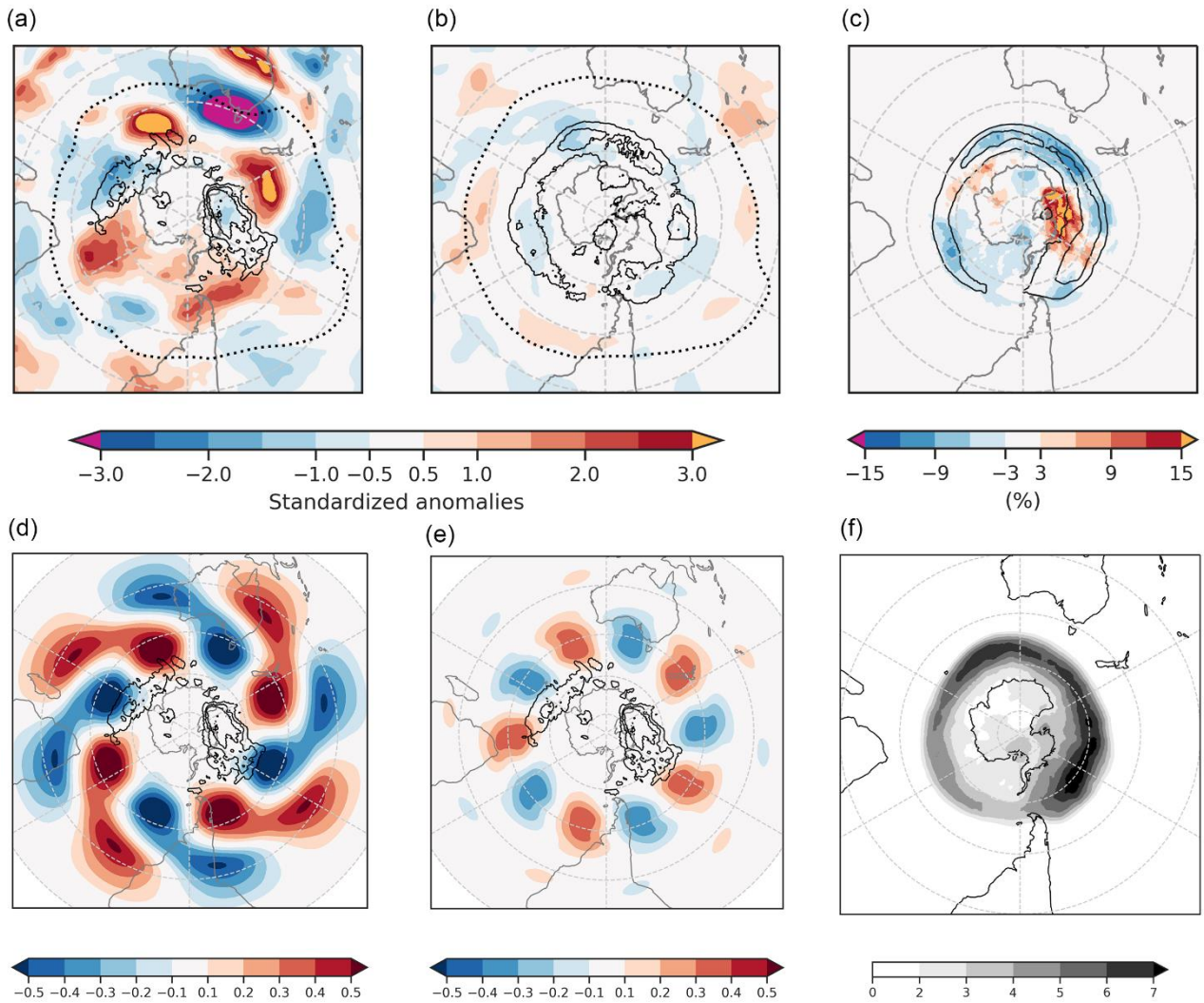
315 Figure 8: Standardized PV anomalies on the 350 K isentropic with respect to the DJF climatology (1979–2018) for (a) High R_{SEA} days and SEA heatwave days (HD), (b) High R_{SEA} days and non-SEA HD. Dotted black lines show 2 PVU contour in the mean PV fields for (a) and (b), and black contours show mean blocking frequency contours at 5, 10, 15 % for the same. (c) Shows the difference in blocking frequency between (a) and (b). (d) shows the WN4 component for the mean PV (in PVU) for High R_{SEA} and SEA HD in (a), (e) shows WN5 component for the same, and the black contours in (d) and (e) show the blocking frequency as in (a). (f) shows the climatological mean blocking frequency (%) for DJF, and black contours in (c) show the same at 4, 6 %.
