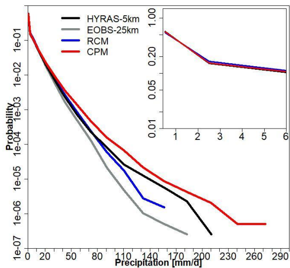
725 Figure 5. Empirical Probability Distribution Functions (PDF) of daily precipitation over SGer in the period 2000-2015 from HYRAS-5km (black), EOBS-25km (grey), RCM (blue), CPM (red). The lowest precipitation rates are shown in the upper-right corner subpanel.
