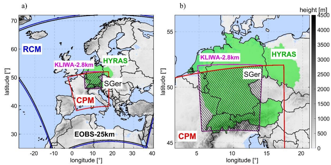
695 Figure 1. a) Simulation, and observation domains for RCM (25km; blue), CPM (3 km; red), KLIWA-2.8km (magenta); HYRAS- 700 5km (green), and EOBS-25km (black). The two investigation domains of this study are Southern Germany (SGer; dashed box), and 705 the CPM domain.
