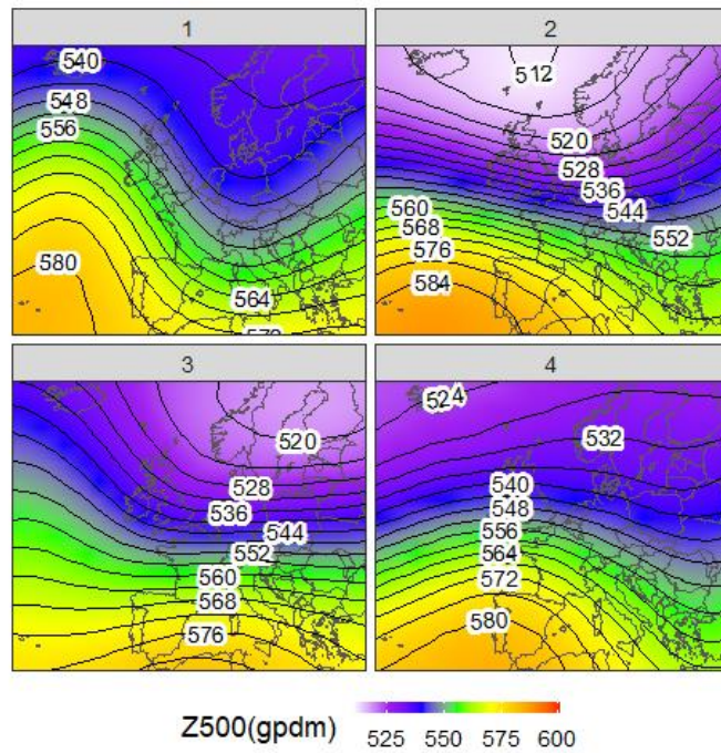
715 Figure 3. Synoptic weather patterns based on Principal Component Analyses for the 98-percentile most severe precipitation cases in winter (SONDJF) of the 1971-2015 period, detected with the PSI. The spatial distributions show 500 hPa geopotential height in geopotential decametres (gpdm) obtained from RCM. The analysis has been performed with the SynoptReg R package (M. Lemus-Canovas et al., 2019).
