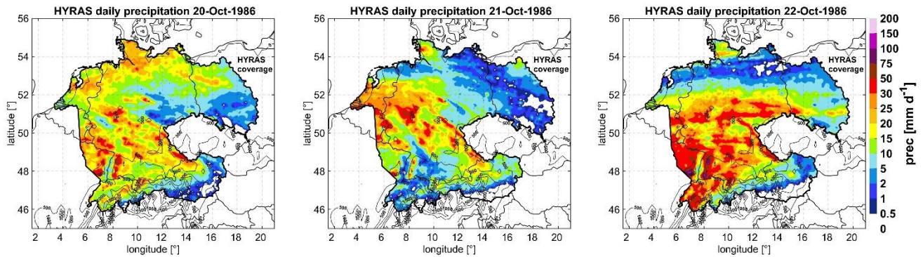
710 Figure 2. (a) Rank correlations between flds and different configurations of the PSI daily values in the period 1971-2015 over SGer obtained with HYRAS-5km. The top three events of the period are shown for each index. (b), (c), and (d) show spatial distributions of daily precipitation measured by HYRAS-km on the 20, 21 and 22 October 1986.
