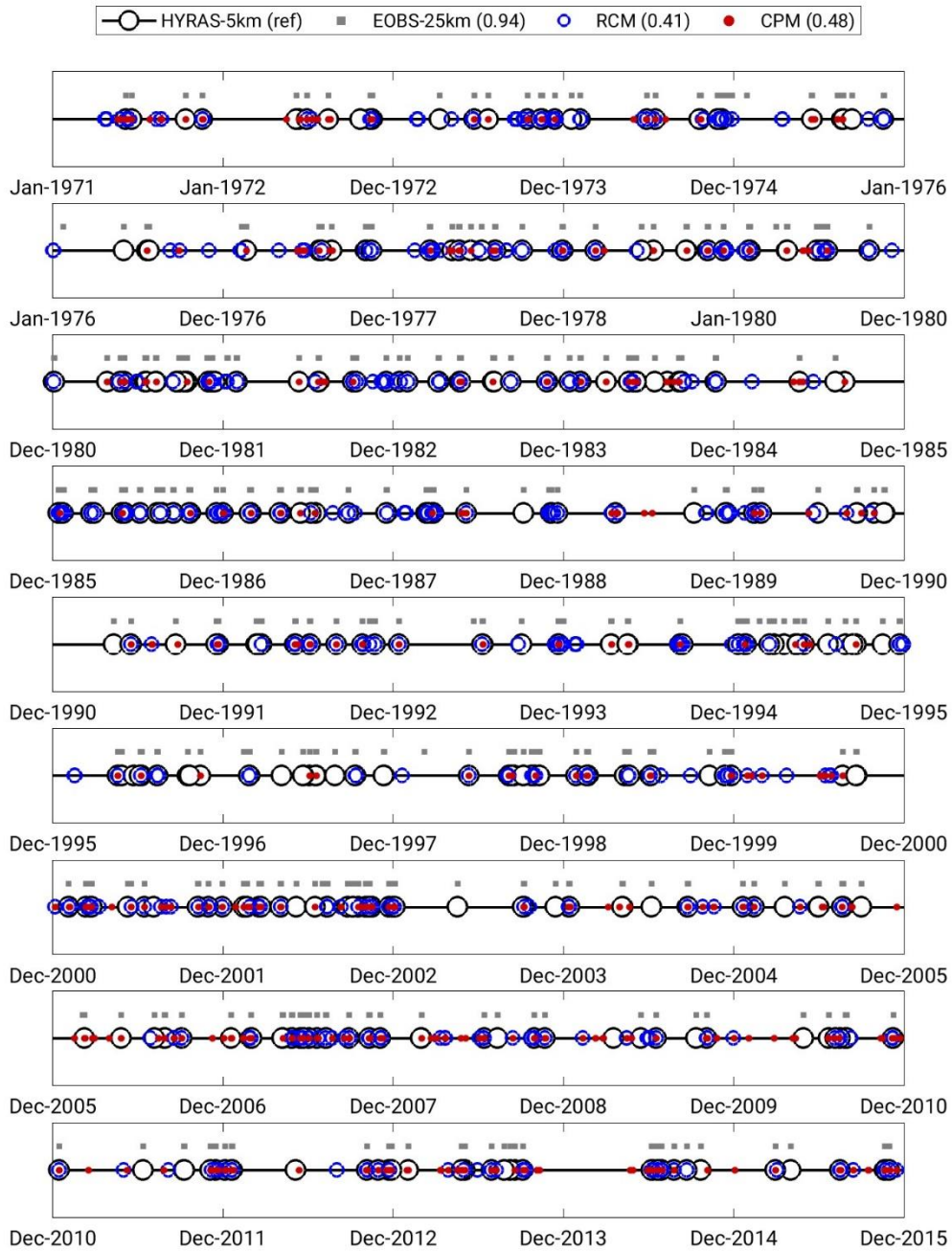
655 Figure 6. Dot diagram of the period 1971-2015, showing the 500 most severe precipitation events, detected using the PSI for HYRAS-5km (black circles), EOBS-25km (grey squares), RCM (blue circles), and CPM (red dots). The CPM data set is extended from Jan-1971 to Dec-1999 using KLIWA-2.8km (Sect. 2.2). The spearman's rank correlation of the data sets is shown in the legend where HYRAS-5km taken as the reference.
