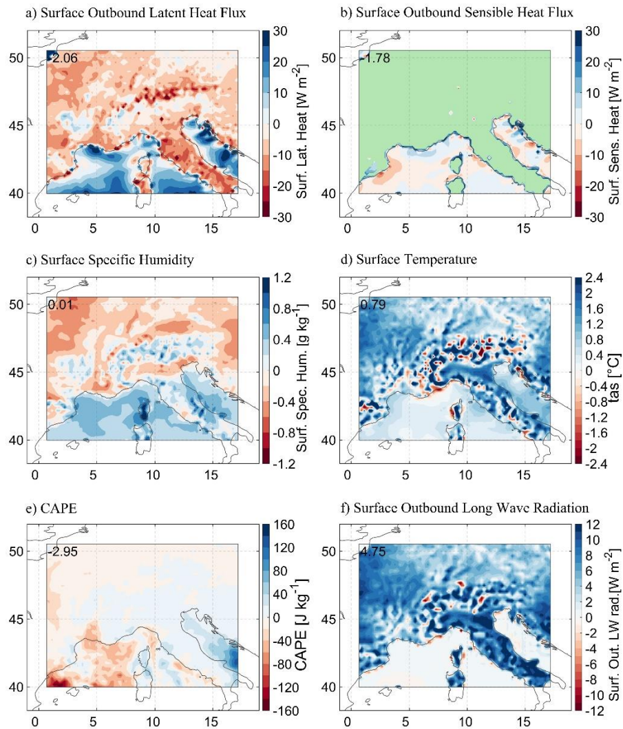
690 Figure 12. Composite precipitation differences between RCM (blue, positive) and CPM (red, negative). All composites correspond to the negative principal components of EOF-3 for winter (SONDJF) events. (a) Surface outbound latent heat flux, (b) Surface outbound Sensible Heat flux, (c) Surface specific humidity, (d) Surface Temperature, (e) CAPE, (f) Surface outbound long wave radiation. Green colours in Latent and Sensible heat fluxes denote inbound directed fluxes and are thus not shown.
