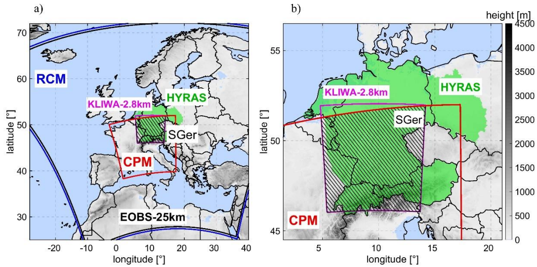
Figure 1. a) Simulation, and observation domains for RCM (25km; blue), CPM (3 km; red), KLIWA-2.8km (magenta); HYRAS-5km (green), and EOBS-25km (black). The two investigation domains of this study are Southern Germany (SGer; dashed box), and the CPM domain.
