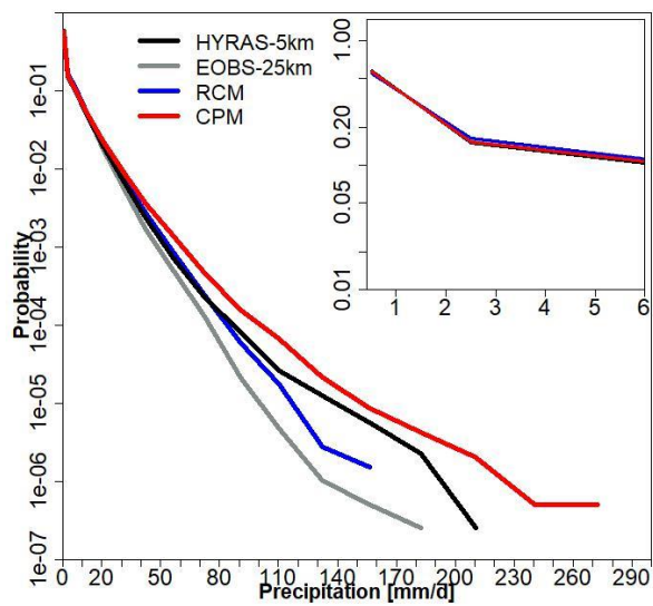
Figure 5. Empirical Probability Distribution Functions (PDF) of daily precipitation over SGer in the period 2000-2015 from HYRAS-5km (black), EOBS-25km (grey), RCM (blue), CPM (red). The lowest precipitation rates are shown in the upper-right corner subpanel.
