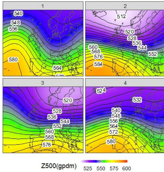
645 Figure 3. Synoptic weather patterns based on Principal Component Analyses for the 98-percentile most severe precipitation cases in winter (SONDJF) of the 1971-2015 period, detected with the PSI. The spatial distributions show 500 hPa geopotential height in geopotential decametres (gpdm) obtained from RCM. The analysis has been performed with the SynoptReg R package (M. Lemus-Canovas et al., 2019).
