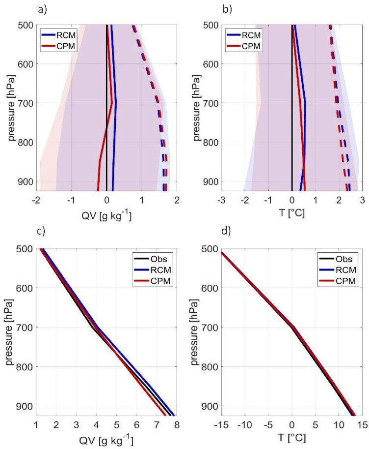
660 Figure 7. (a, b) Mean bias (solid line), standard deviation of the differences (shaded areas) and RMSE (dashed lines). (c, d) Humidity and temperature profiles of RCM, CPM, and the observations. Radiosondes obtained from the UWYO soundings at Nimes (France); Oppin, Meiningen, Idar-Oberstein, Stuttgart, Kümmersbruck and Munich (Germany); Praha (Czech Republic); Milano, S. Pietro, and Pratica di Mare (Italy). The model information is interpolated to the station location.
