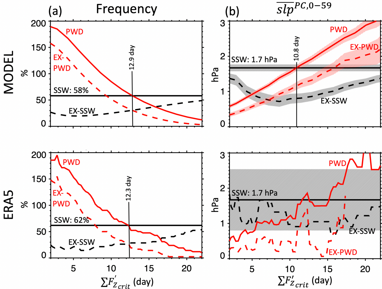
Figure 2: Sensitivity of (a) event frequency (%) and (b) surface response (hPa) to the wave driving \Sigma F'_{Z_{crit}} . Event frequency is given in %, i.e., events per year multiplied by 100. The surface response in (b) is the polar-cap-averaged (60-90°N) sea level pressure (SLP) anomaly averaged from day 0 to 59 after onset ( \overline{slp}^{PC,0-59} ). Thick horizontal line is for SSWs. Shading in (b) shows the 95% confidence intervals. EX-PWDs and EX-SSWs are events that are either only PWDs or only SSWs. The top panels for the model show that (a) at \Sigma F'_{Z_{crit}} = 12.9 day the frequency of PWDs is similar to SSWs, and (b) that at \Sigma F'_{Z_{crit}} = 10.8 day the SLP response to PWDs is similar to SSWs.
