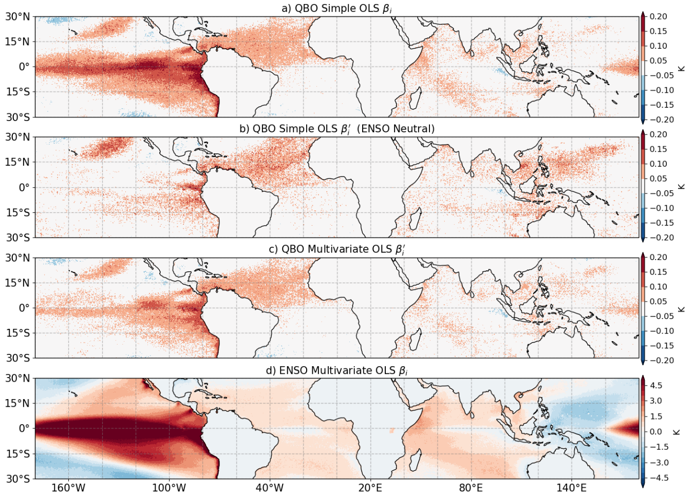
Figure S3. Regression analysis as in Figure 5 of the main manuscript but for sea-surface temperatures (SSTs).
