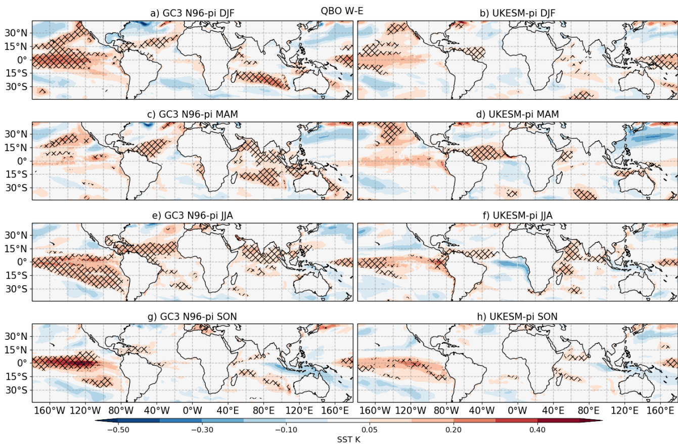
Figure S2. SST composite differences for (left) GC3 N96-pi and (right) UKESM-pi for the seasons of (a-b) DJF, (c-d) MAM, (e-f) JJA and (g-h) SON.
