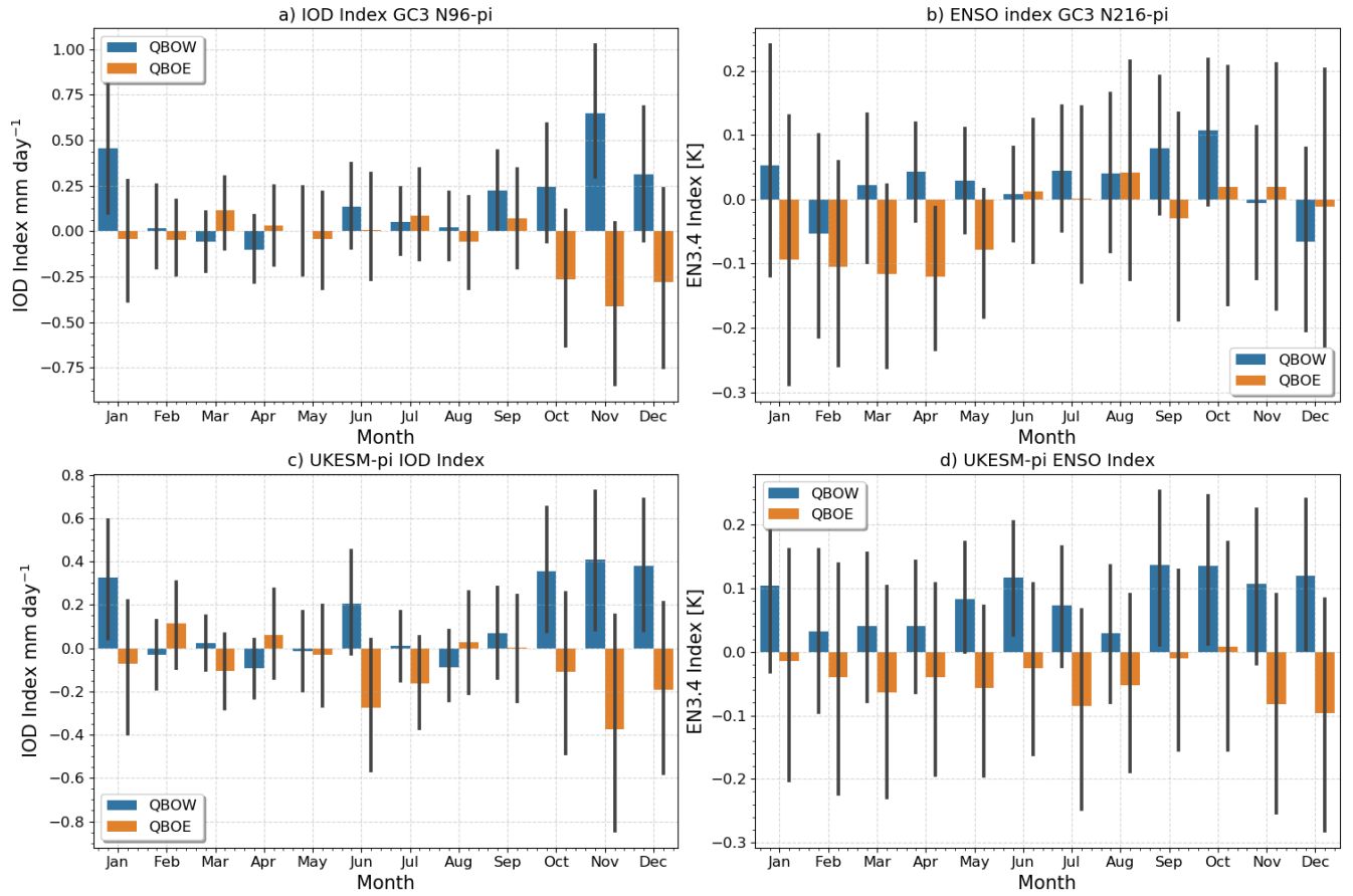
Figure S4. As in Figure 6 of the main manuscript but for (a, b) GC3 N96-pi and (c, d) UKESM-pi.
