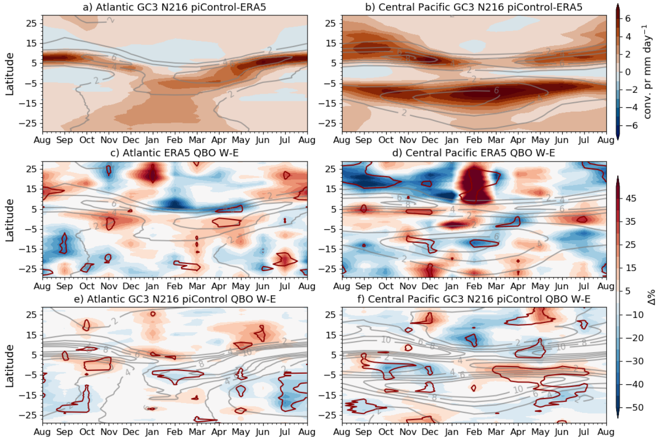
Figure S5. As in Figure 9 of the main manuscript but only for Neutral years only.
