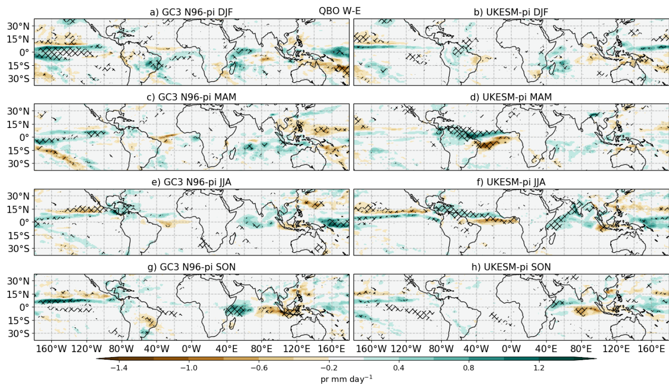
Figure S1. Seasonal mean precipitation differences between QBO W-E phases in (left) GC3 N96-pi and (right) UKESM-pi for (a, b) DJF, (c, d) MAM, (e, f) JJA and (g, h) SON. Hatching denotes statistically significant differences to the 95% confidence level using a bootstrapping with replacement test.
