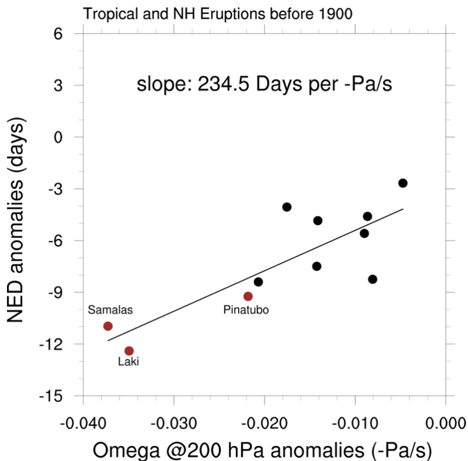
Figure 7 Scatter plot of the JA omega velocity anomalies (-Pa/s) at 200 hPa averaged over the mean ascending region (black boxes in Figure 6) against the corresponding NED anomalies in the CESM-LME. Negative omega velocity anomalies indicate reduced upwelling. Tropical and NH volcanoes before 1900 are used only. Brown circles denote Pinatubo, Samalas and Laki. A linear regression calculates a negative slope of about 2.3 days per 0.01 -Pa/s significant at p < 0.01 based on a two tailed t-test.
