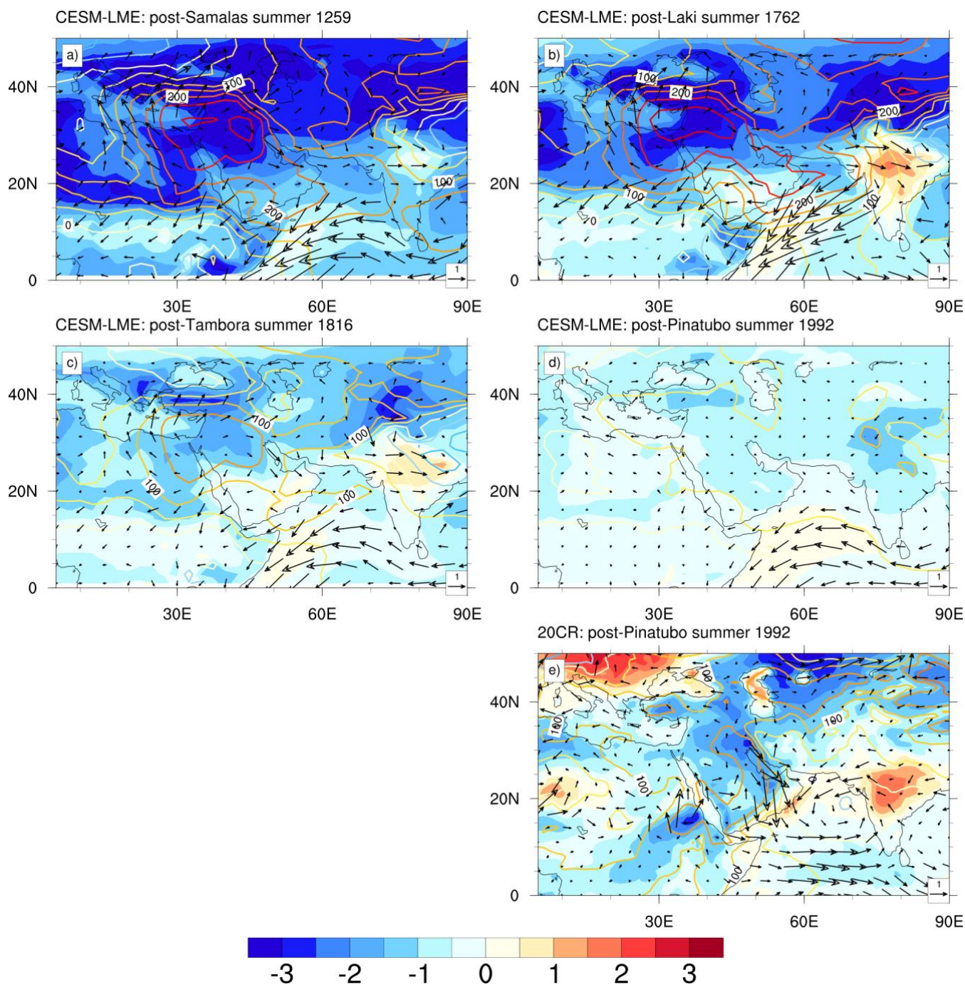
Figure 5 Anomalies of surface temperature (K, shaded), 10m winds (m/s, arrows) and SLP (Pa, contours) in the post-eruption summers (JA) following Samalas, Laki, Tambora and Pinatubo. Years of the maximum NED response according to Figure 3. Panels a-c) from CESM-LME and e) from 20CR. Anomalies relative to the average 5 years before the eruption year (see Table 1). No significance test is overlaid. See Sup. Figure 2 for all eruptions listed in Table 1.
