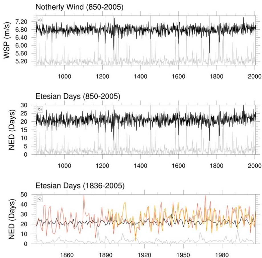
480 Figure 2 Time series of the JA WSP (m/s) and NED (days) over the last millenium (850-2005) for CESM-LME (black), 20CR (red) and L-days (orange). (a) CESM-LME ensemble mean WSP time series. (b) CESM-LME ensemble mean NED time series. (c) NED time series over the common period 1836-2005 for CESM-LME, 20CR and L-days. Note the different range between panels b) and c). The outgoing clear-sky SW radiation at the top of the atmosphere, averaged over the Northern Hemisphere (0-90 °N, grey lines, relative scaling), is used here as proxy of stratospheric aerosol loading, with peaks indicating 485 volcanic eruptions.
