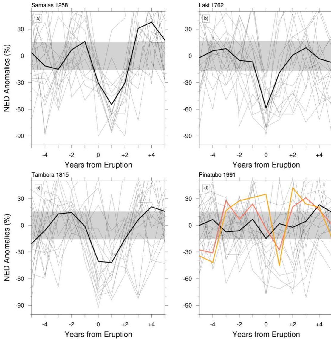
Figure 3 Percentage anomalies of NED for (a) Samalas, (b) Laki, (c) Tambora and (d) Pinatubo eruptions in CESM-LME (black), 20CR (red) and L-days (orange), from 5 pre-eruption to 5 post-eruption years. Zero denotes the year of eruption as listed in Table 1. Thin black lines show percentage NED anomalies for the 17 individual runs of the CESM-LME ensemble. Grey shading measures the \pm 2 standard deviation of pre-eruption (-5 to -1 years) NED in CESM-LME. See Sup. Figure 1 for all eruptions listed in Table 1.
