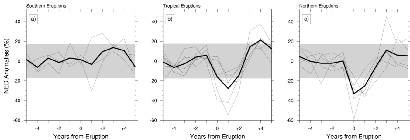
Figure 4 Percentage anomalies of NED in CESM-LME for (a) Southern hemisphere, (b) tropical and (c) Northern hemisphere volcanic eruptions from 850 to 1900 (bold eruption years in Table 1). Zero denotes the year of eruption. Thin black lines show the ensemble mean anomalies for every eruption and the thick black line shows the multi-eruption mean response. Grey shading measures the \pm 2 standard deviation of pre-eruption (-5 to -1 years) NED.
