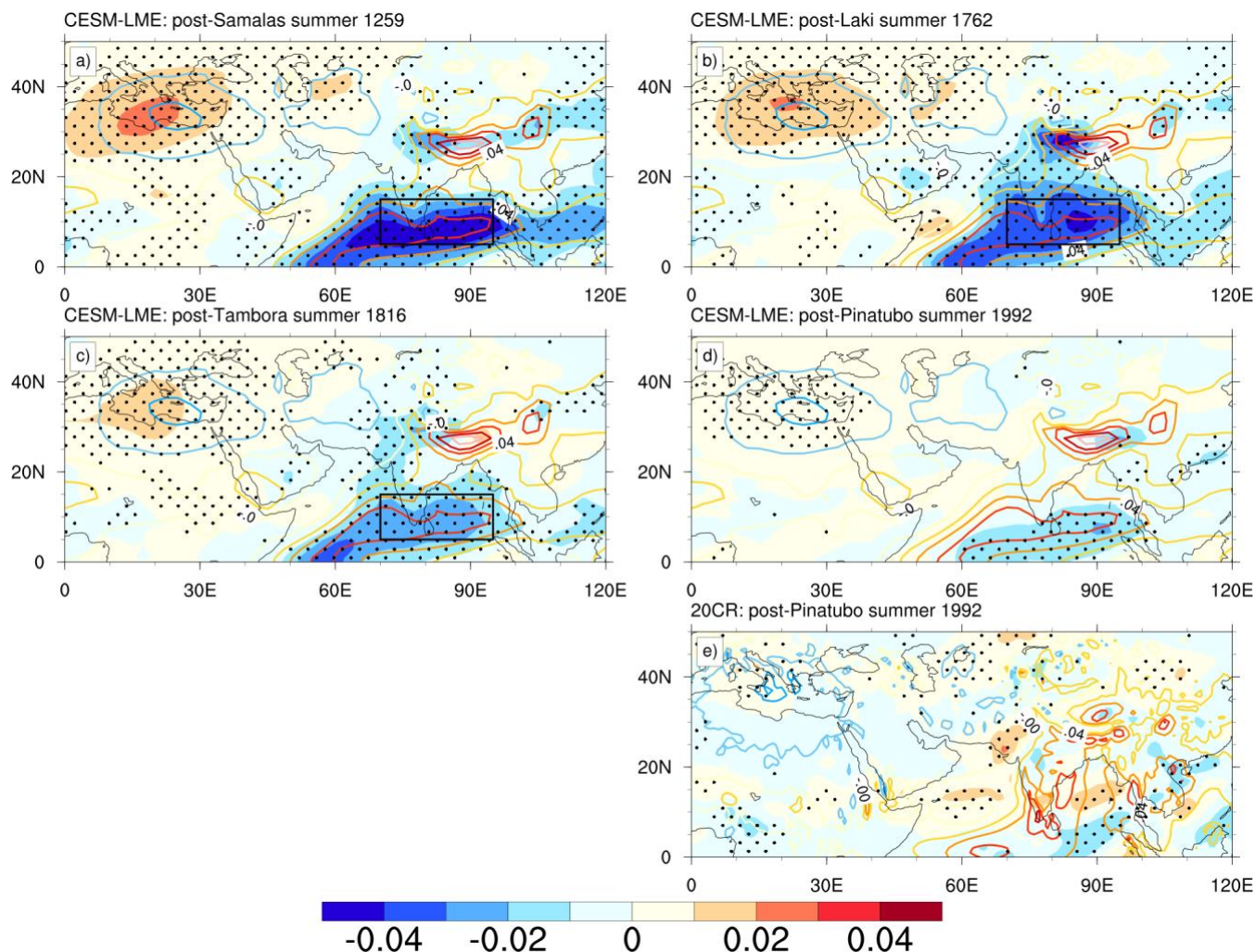
Figure 6 Anomalies of omega velocity ( -\text{Pa/s} , shaded) at 200 hPa in the post-eruption summers (JA) following Samalas, Laki, Tambora and Pinatubo. Years of the maximum NED response according to Figure 3. Climatology of omega velocity ( -\text{Pa/s} ) show regions of upwelling (red positive contours) and downwelling (blue negative contours). Panels a-c) from CESM-LME and e) from 20CR. Positive (negative) anomalies indicate reduced descending (ascending) motions. Anomalies relative to the average 5 years before the eruption year (see Table 1). Regions of p < 0.05 based on a two-tailed t-test are stippled. See Sup. Figure 4 for all eruptions listed in Table 1. Black boxes in panels a-c denote areas used for averaging omega velocity anomalies shown in Figure 7.
