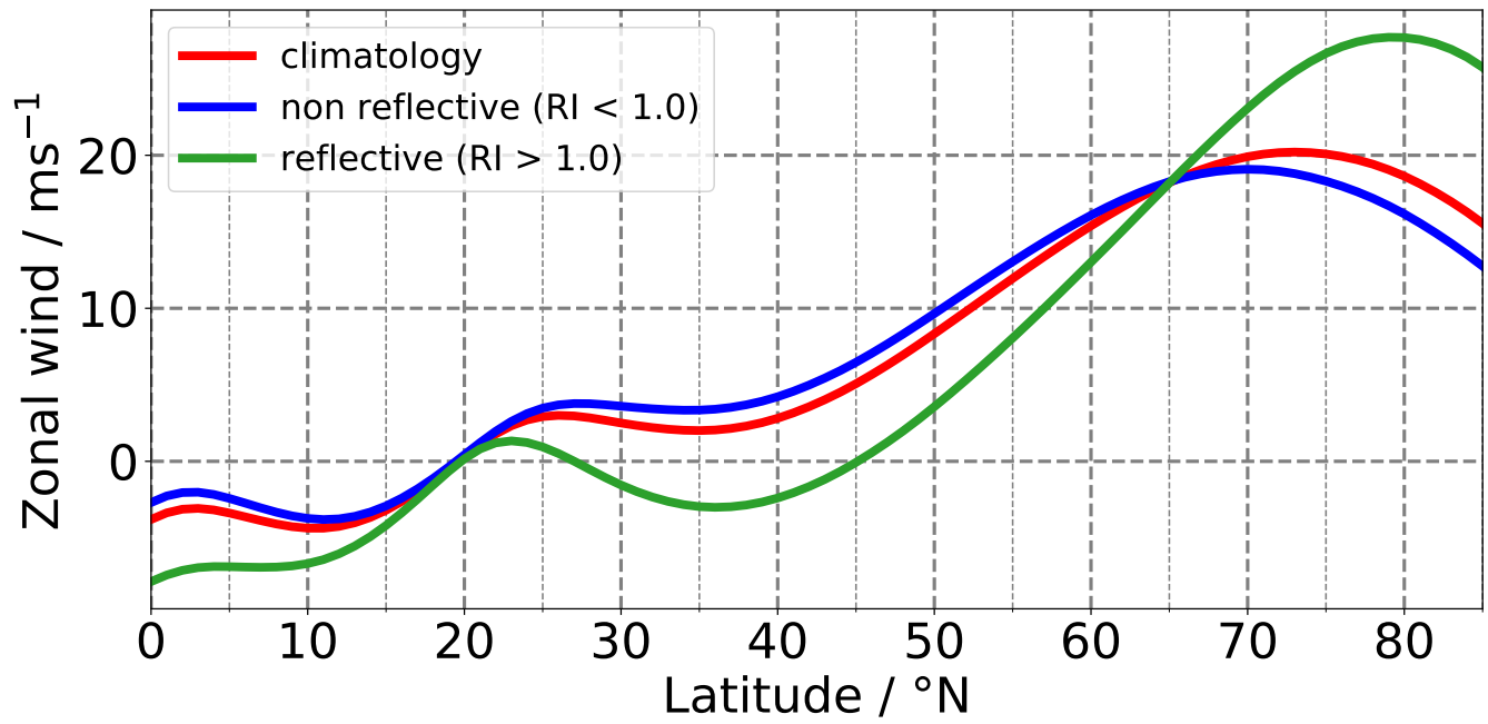
Figure A2. Meridional profiles of the zonal wind averaged over 230–280 ^{\circ}\text{E} (Canadian sector) at 30hPa. Climatology of all winter days (red line), days when \text{RI} > 1 (green line) and days when \text{RI} < 1 (blue line).
