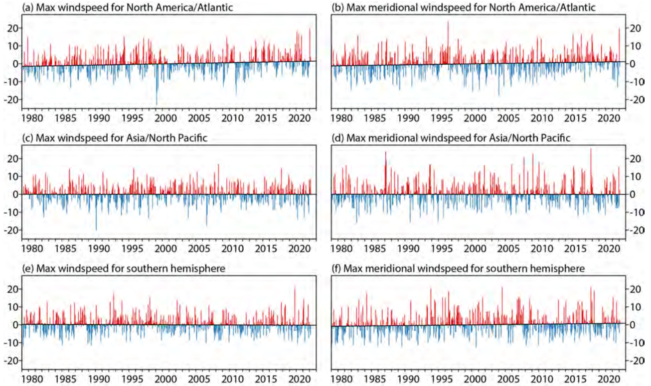
Figure 16: Deviations (ms -1 ) from average values for each month in the period March 1979 to February 2022 in the highest 200 hPa windspeed analysed during the month over regions covering most of (a) North America and the North Atlantic (120° W-20° W; 20° N-90° N), (c) Asia and the North Pacific (60° E-120° W; 20° N-90° N) and (e) the southern hemisphere south of 20° S. Panels (b), (d) and (f) are corresponding time series for the maximum speed of the meridional wind component. Values are plotted according to whether they are above (red) or below (blue) the least-squares-fit linear trend for the period.
