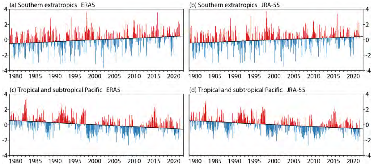
745 Figure 19: Monthly means of 850 hPa zonal winds ( \text{ms}^{-1} ) averaged over the southern extratropics ( 45^\circ \text{ S} - 60^\circ \text{ S} ) for (a) ERA5 and (b) JRA-55, and over central latitudes of the Pacific ( 30^\circ \text{ N} - 30^\circ \text{ S} , 160^\circ \text{ E} - 120^\circ \text{ W} ) for (c) ERA5 and (d) JRA-55. They are shown relative to the average for each month in the period from March 1979 to February 2022, and plotted according to whether they are above (red) or below (blue) the least-squares-fit linear trend for this period.
