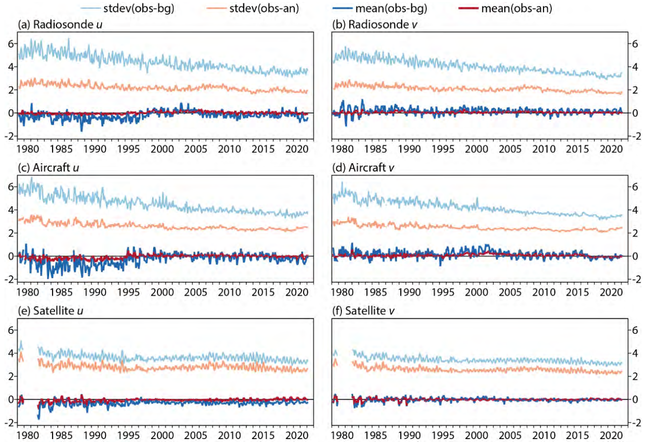
600 Figure 13: Monthly means and standard deviations of observation minus background (dark/light blue) and observation minus analysis (red/orange) departures ( \text{ms}^{-1} ) for the 175 to 225 hPa layer over the region from 10^\circ \text{ S} to 10^\circ \text{ N} and 90^\circ \text{ W} to 150^\circ \text{ E} , from March 1979 to February 2022, for zonal ( u ) and meridional ( v ) wind components from (a, b) radiosondes, (c, d) aircraft and (e, f) satellite imagery.
