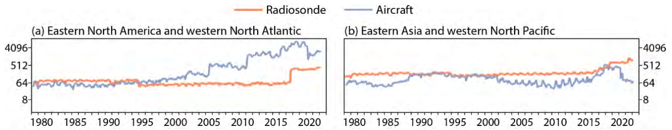
Figure 14: Monthly average number of observations per day for the 175 to 225 hPa layer, from March 1979 to February 2022, for radiosondes (red) over the regions (a) from 35° N to 55° N and 80° W to 50° W and (b) from 25° N to 45° N and 115° E to 145° E and aircraft (blue) over the regions (a) from 35° N to 55° N and 60° W to 30° W and (b) from 25° N to 45° N and 145° E to 175° E.
