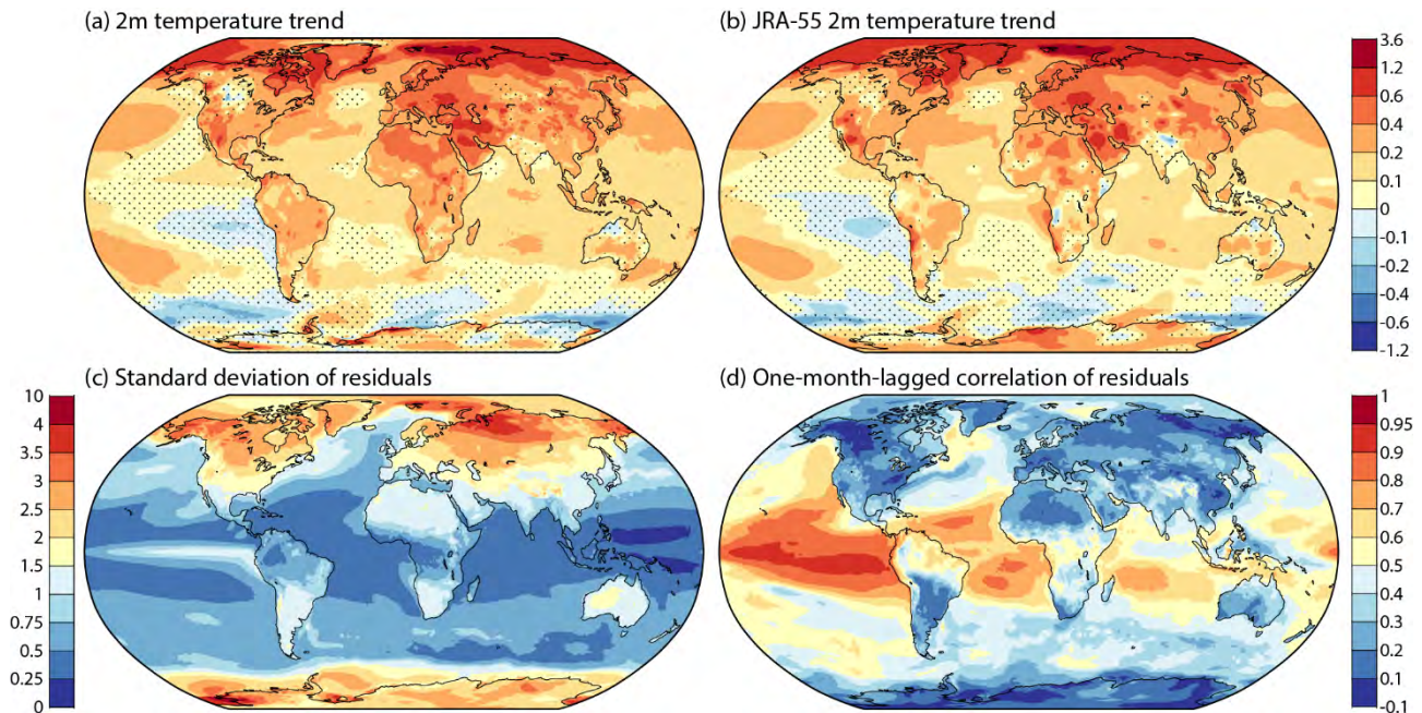
Figure 2: (a) The least squares linear trend (K/decade) in two-metre temperature based on monthly average ERA5 data from March 1979 to February 2022. (b) As (a), but for JRA-55. Dots show where the 95 % confidence intervals are two-signed. (c) The standard deviation of differences between two-metre temperatures and their linear trend (K). (d) The correlation coefficient between successive monthly deviations of two-metre temperature from the linear trend.
