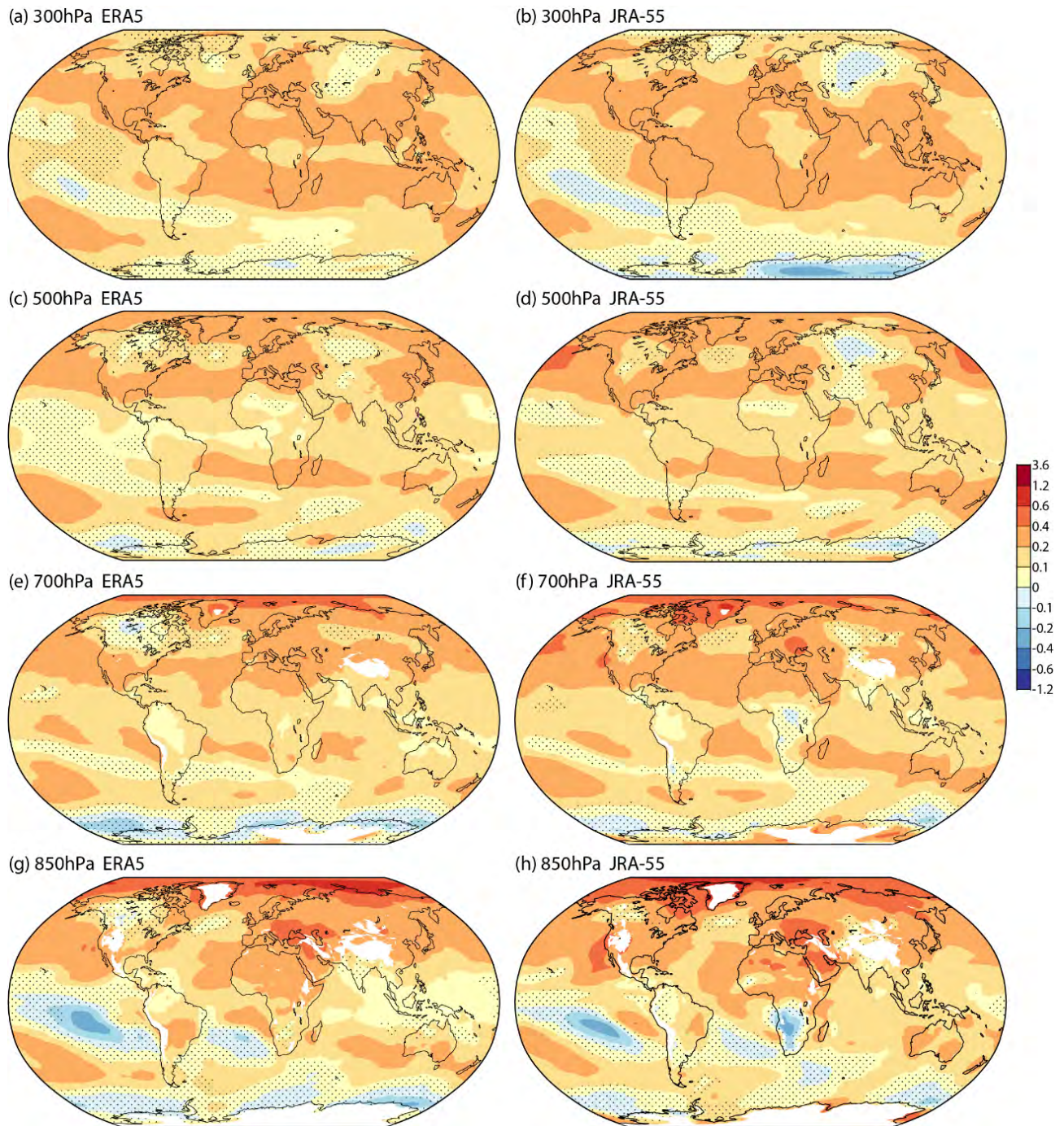
Figure 4: The least squares linear trend (K/decade) in monthly average ERA5 (left) and JRA-55 (right) temperatures from March 1979 to February 2022 for (a, b) 300 hPa, (c, d) 500 hPa, (e, f) 700 hPa and (g, h) 850 hPa. Dots show where the 95 % confidence interval is two-signed. Regions where the ERA5 model orography exceeds 1500 m (for 850 hPa) or 3000 m (for 700 hPa) are masked in white.
