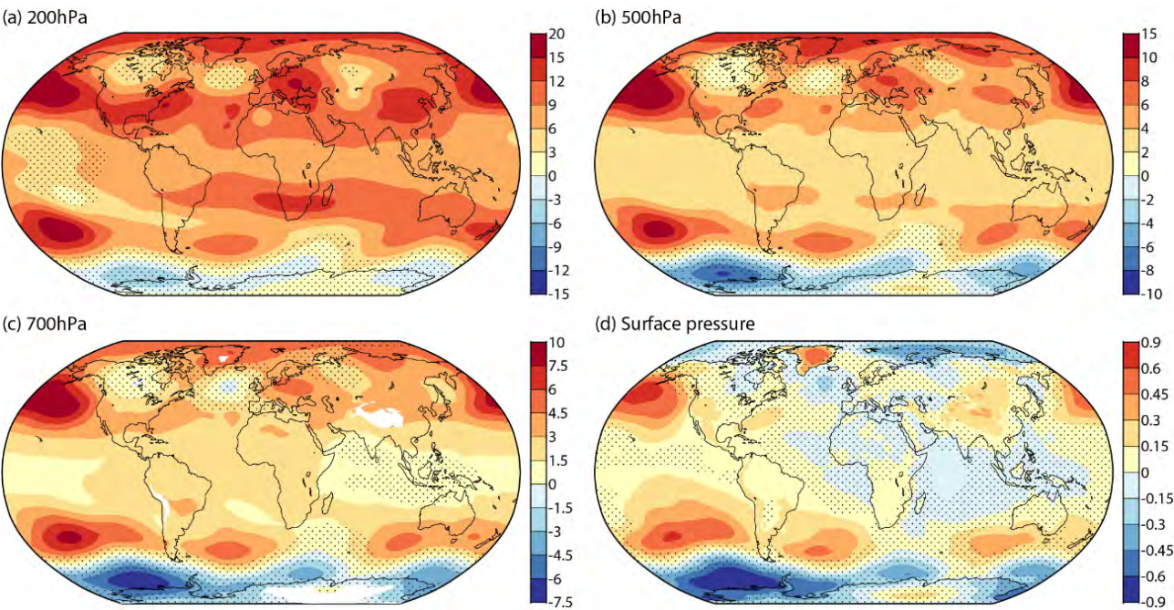
760 Figure 20: Trends in geopotential height (m/decade) and surface pressure (hPa/decade) derived from least squares linear fits of monthly mean deviations from average values for each month in the period March 1979 to February 2022. (a) 200 hPa height, (b) 500 hPa height, (c) 700 hPa height and (d) surface pressure. Dots show where the 95 % confidence interval is two-signed. 700 hPa regions where the ERA5 model orography exceeds 3000 m are masked in white.
