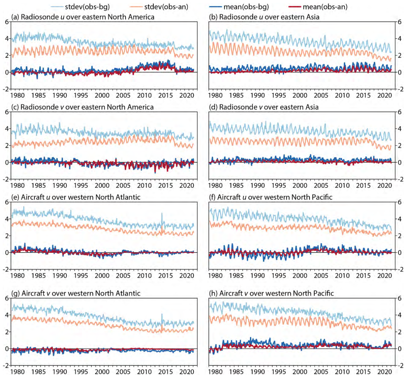
Figure 15: Monthly means and standard deviations of observation minus background (dark/light blue) and observation minus analysis (orange/red) departures ( \text{ms}^{-1} ) for the 175 to 225 hPa layer, from March 1979 to February 2022, for zonal ( u ) and meridional ( v ) wind components from radiosondes over the regions (a, c) 35^{\circ}\text{N} to 55^{\circ}\text{N} and 80^{\circ}\text{W} to 50^{\circ}\text{W} and (b, d) from 25^{\circ}\text{N} to 45^{\circ}\text{N} and 115^{\circ}\text{E} to 145^{\circ}\text{E} , and aircraft over the regions (e, g) from 35^{\circ}\text{N} to 55^{\circ}\text{N} and 60^{\circ}\text{W} to 30^{\circ}\text{W} and (f, h) from 25^{\circ}\text{N} to 45^{\circ}\text{N} and 145^{\circ}\text{E} to 175^{\circ}\text{E} .
