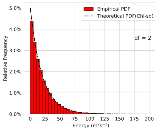
Figure 2. Atmospheric energy distribution for the Rossby wave with the zonal wavenumber k = 7 , meridional mode n = 3 and vertical mode index m = 1 in ERA5 for 1980–2014. The dashed black lines correspond to the theoretical \chi^2 -distribution ( df are the degrees of freedom).
