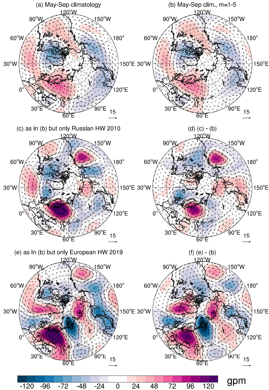
Figure 3. (a,b) Climatological Rossby wave circulation for extended boreal summer (MJJAS) at the \sigma level close to 500 hPa in the midlatitudes. (a) All zonal wavenumbers k > 0 , all meridional modes n and all vertical modes m are included. (b) As in (a), but only troposphere-barotropic vertical modes, m = 1 - 5 . (c) As in (b) but for the Russian Heat Wave (HW) in 2010. (d) Difference between the (c) and (b). (e) As in (b), and (f) as in (d) but for the European HW in 2019. Coloured contours are geopotential height anomalies (in gpm). The wind speed is shown by the length of the wind vectors (with 15 m/s -1 as a reference vector).
