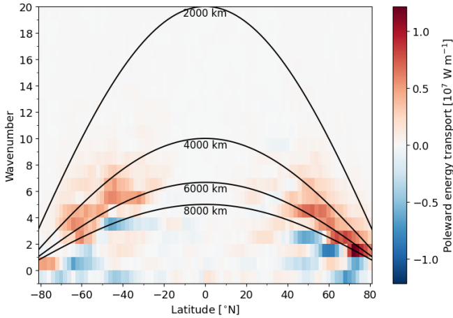
Figure 3. The composite of the anomalous poleward energy transport by individual waves ( \langle vE \rangle_n of Eq. 11) at different latitudes 4 d after situations of anomalous high (90th percentile) meridional temperature contrasts around the latitude of energy transport. The anomalies on a daily resolution are computed from the 21 d and 9-year running-mean climatology. The meridional temperature contrast is computed by the difference between the zone 10^\circ equatorward and 10^\circ poleward of the latitude of interest. Hence, red colours denote waves transporting more energy polewards 4 d after situations of enhanced meridional temperature differences. The wavenumbers corresponding to wavelengths of 2000, 4000, 6000, and 8000 km are depicted by black lines. Wave 0 is corrected by the meridional mass flux to express the instantaneous zonal-mean transport according to Lembo et al. (2019).
