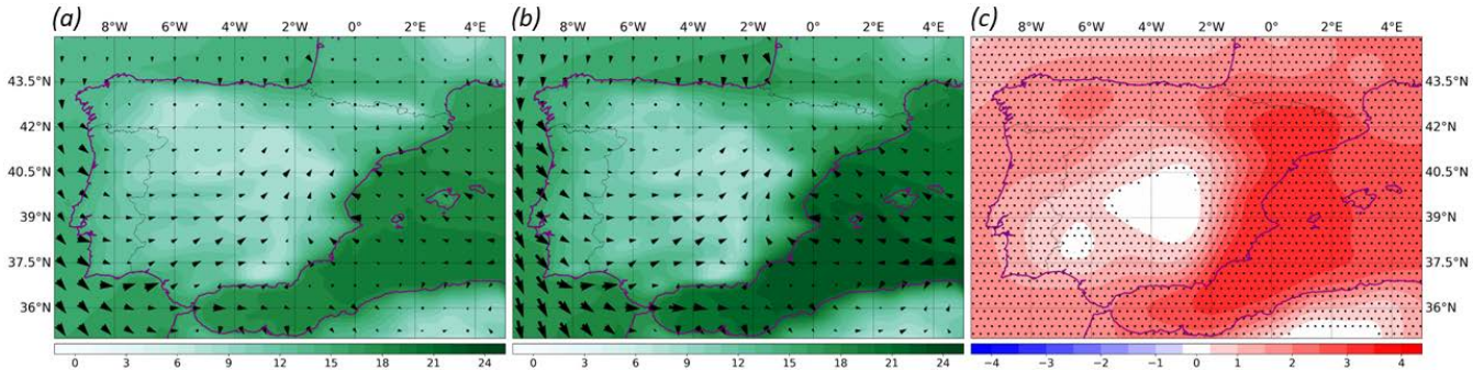
Figure 4: 2-m dew point temperature (contours; °C) and 10 meters wind (arrows; m s^{-1} ) composites at t_0 for (a) SP-NONHAIL, (b) SP-HAIL and (c) Differences between SP-HAIL and SP-NONHAIL. Black points in plot c) denote statistically significant differences ( p -value < 0.05 ) in dew point temperature.
