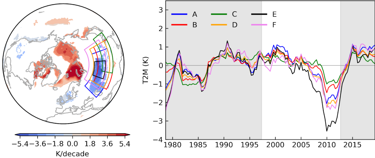
Figure S2. Left: Trends in 2 metre air temperature as in Figure 1. Boxes with various colors show the selected regions for calculating the Eurasian cooling. Regions include 40-60°N, 45-110°E (blue), 35-55°N, 60-120°E (yellow; He et al. 2020), 35-50°N, 80-130°E (green; Kug et al. 2015), 40-60°N, 60-120°E (orange; Mori et al. 2014), 46-59°N, 70-95°E (black; Outten and Esau 2012 Figure 1) and 45-65°N, 55E-125°E (violet; Ogawa et al. 2018). Right: Anomaly of 2 metre air temperature averaged over the various boxes for the period of 1998 to 2012.
