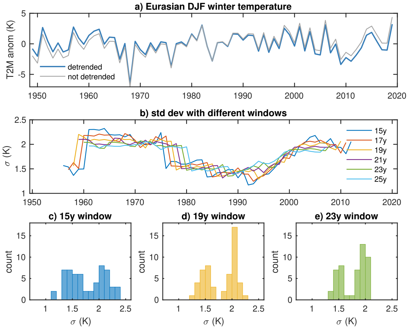
Figure S4. Eurasian winter temperature variability. a) Time series of 2-metre winter temperature anomalies from the ERA5 reanalysis area-averaged over 40-60°N and 60-120°E. The year corresponds to the December of each DJF season. b) Centered running standard deviation \sigma of the temperature time series for different windows (in years). (c-e) Histograms of standard deviations for three of the window lengths in (b).
