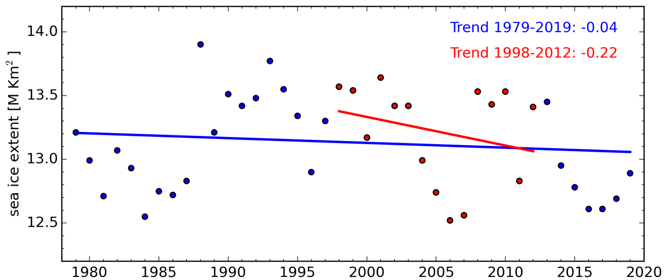
Figure S3. The March Arctic sea ice extent (dots) and its linear trend (solid lines) in National Snow Ice Data Centre (NSIDC) dataset in million sq. km. Trends are calculated over two periods, 1979-2019 (blue) and 1998-2012 (red).
