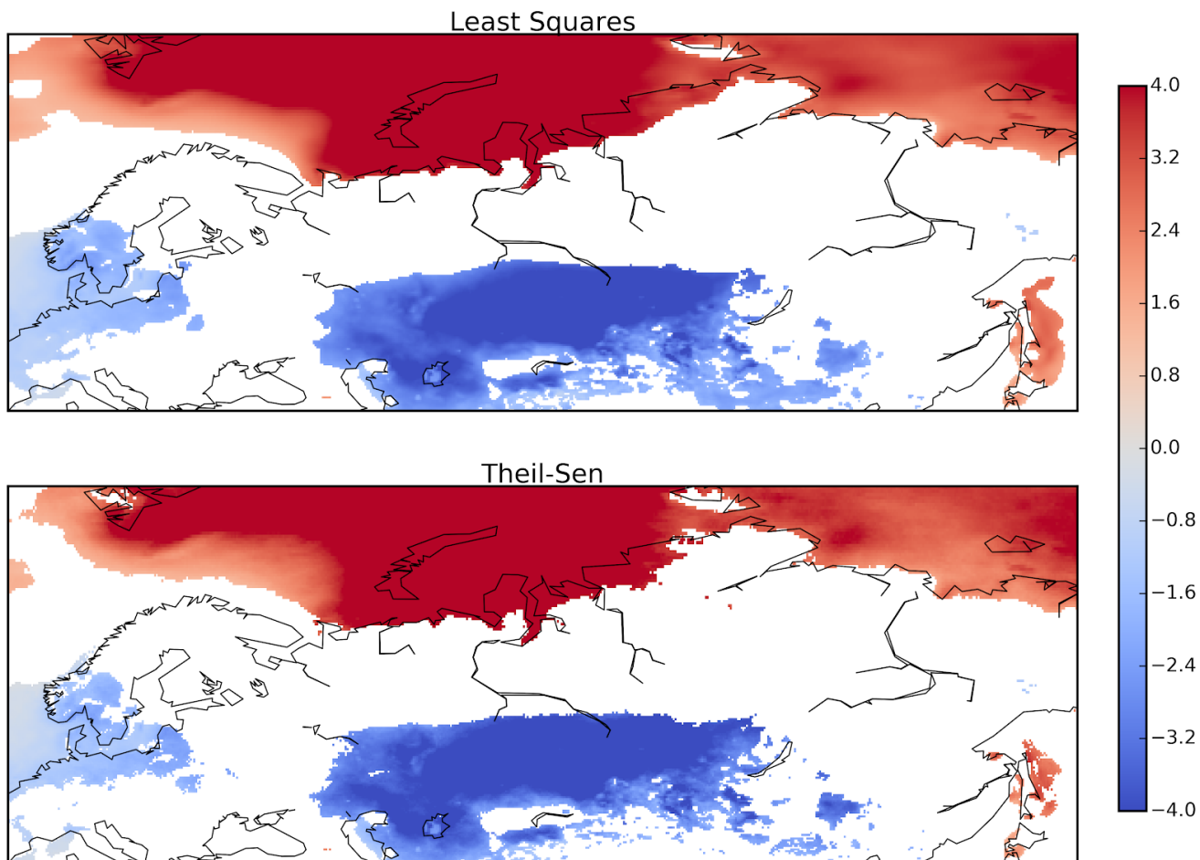
Figure S1. Trends in DJF mean 2-metre air temperature in ERA5 reanalysis for 1998 to 2012, calculated using the least squares (top) and Theil-Sen (bottom) methods. These are shown over the domain of 0-150°E and 40-80°N. Trends are only shown for locations that are significantly different at the 95% level from the mean Northern Hemisphere trend for the given period.
