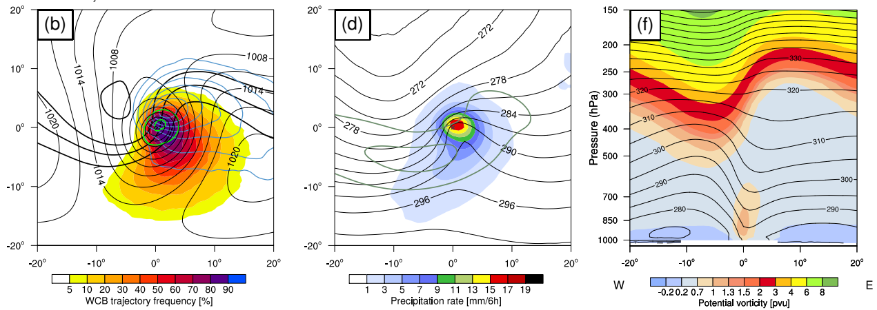
Figure 3. Composites of C1 cyclones in NH winter in (a, c, e) ERA-Interim and (b, d, f) CESM-HIST in the middle of the 24 h period of strongest deepening. (a, b) Frequency of WCB air parcels with p > 500 hPa (%; shading), p < 500 hPa (blue contours at 5%, 10%, 20%, 30%, ..., 80%) and WCB air parcels with PV > 1 pvu and 900 > p > 700 hPa (green contours at 10%, 50% and 60%), SLP (thin black contours every 3 hPa) and PV at 250 hPa (thick black contours at 2, 3, 4 and 6 pvu). (c, d) 6-h accumulated precipitation (mm; shading), potential temperature at 850 hPa (black contours every 3 K) and wind speed at 250 hPa (green contours at 50 and 60 \text{ m s}^{-1} ). (e, f) West-east oriented cross section across the centre of the composite cyclone, showing PV (pvu; shading) and potential temperature (black contours every 5 K).
