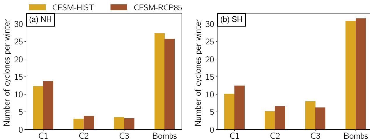
Figure 5. Number of C1, C2, C3 and bomb cyclones per winter in CESM-HIST and CESM-RCP85 in the (a) NH and (b) SH.
