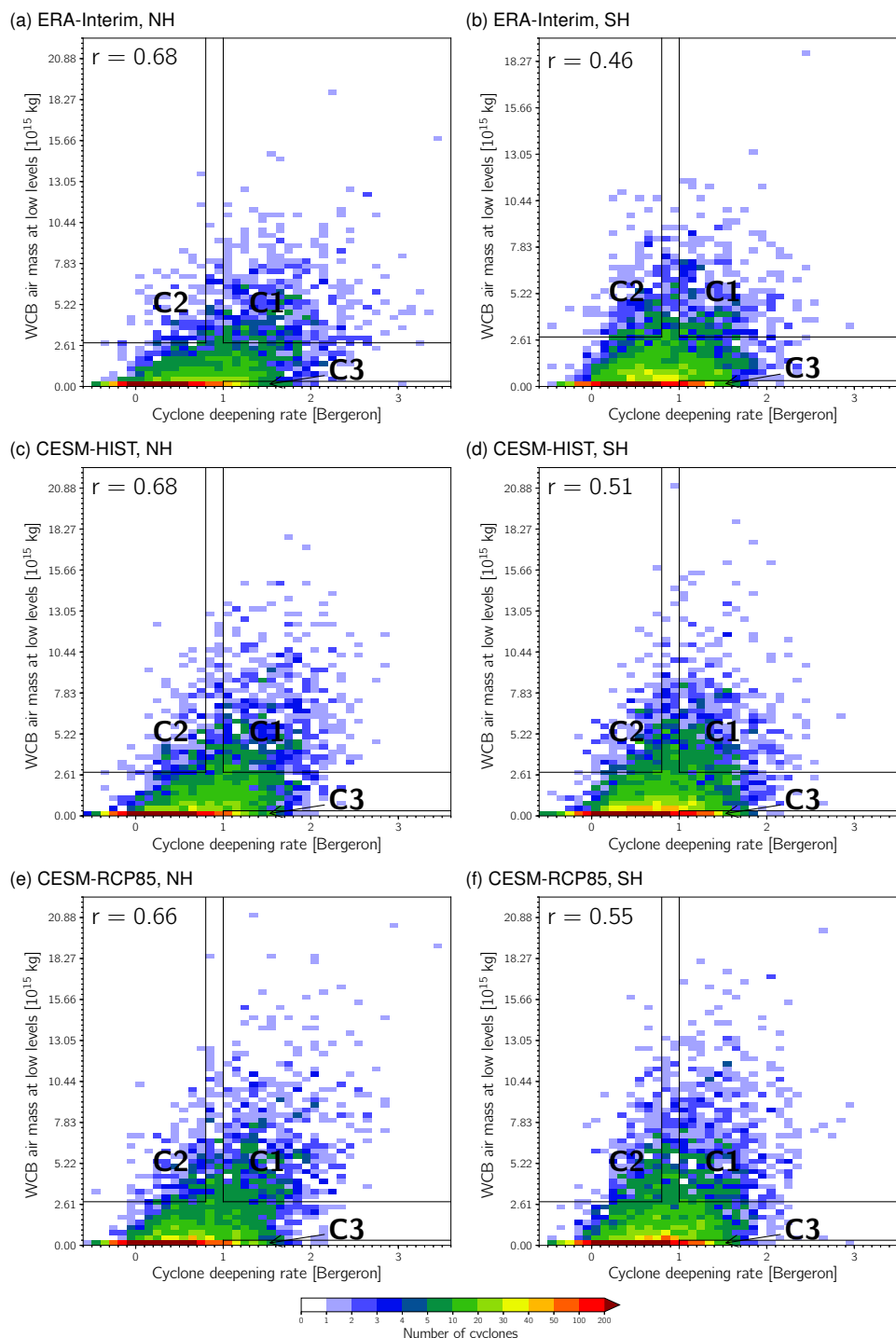
Figure 2. Two-dimensional histograms showing for all (a, c, e) NH and (b, d, f) SH winter cyclones in (a, b) ERA-Interim, (c, d) CESM-HIST, and (e, f) CESM-RCP85 the cyclone intensification rate \Delta SLP_{B,max} (bin width = 0.1 Bergeron) and the WCB strength (bin width \approx 0.33 \times 10^{15} kg, corresponding to 250 WCB trajectories). The colours specify the number of cyclones per bin. The black lines mark the borders of categories C1, C2 and C3.
