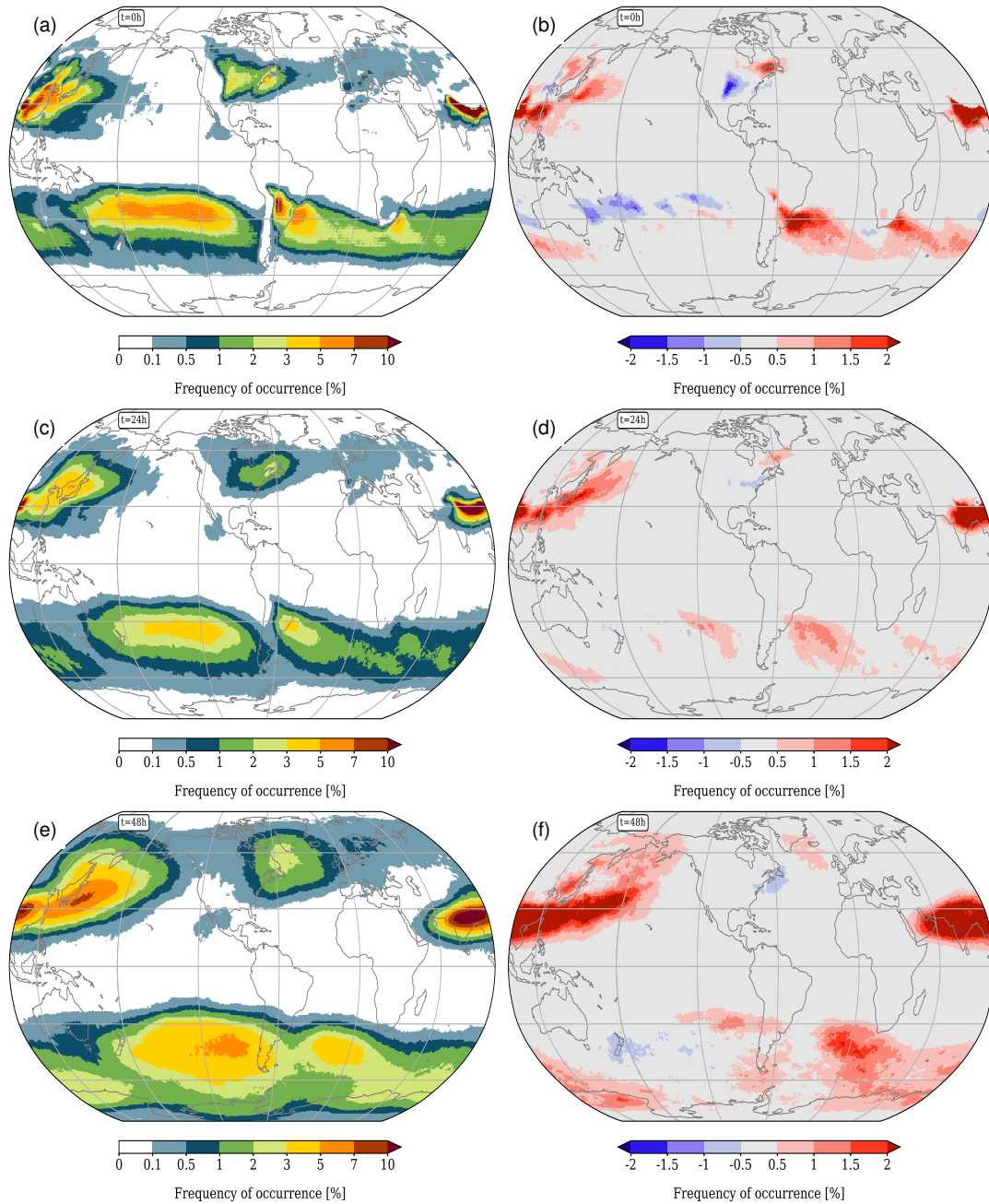
Figure 5. Same as Figure Fig. 4 but for JJA.
