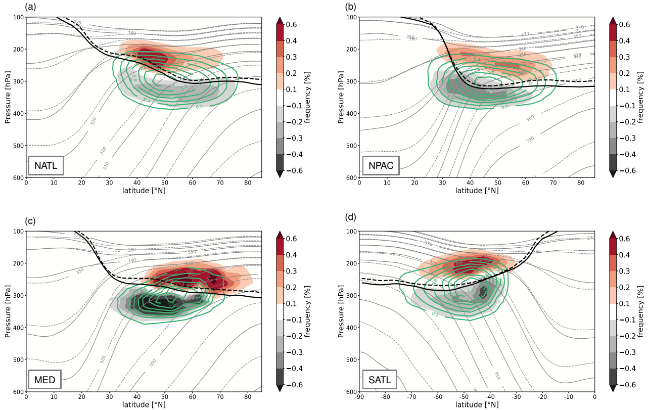
Figure 11. 50-year mean potential temperature (solid/dashed grey lines) and potential vorticity (2 pvu isolines; solid/dashed-thick black lines), zonally averaged over the four target regions (a) NATL, (b) NPAC, SATL and (c) MED, and (d) SATL. Dashed lines correspond to RCP85 and solid lines to HIST. Green solid lines show the distribution-normalized frequency (binsize 5°, 25 hPa) of the WCB air parcels at the end of their ascent for HIST (outermost line for 0.2% with an increment of 0.2 for NATL, NPAC, SATL and 0.3 for MED). The corresponding shift in a future effect of climate change on the normalized WCB frequency, RCP85 minus HIST, is shown in color shading. All panels are for winter in the corresponding hemisphere, i.e., DJF in (a, b, c) and JJA in (d) and the PV has been multiplied by -1 in SATL.
