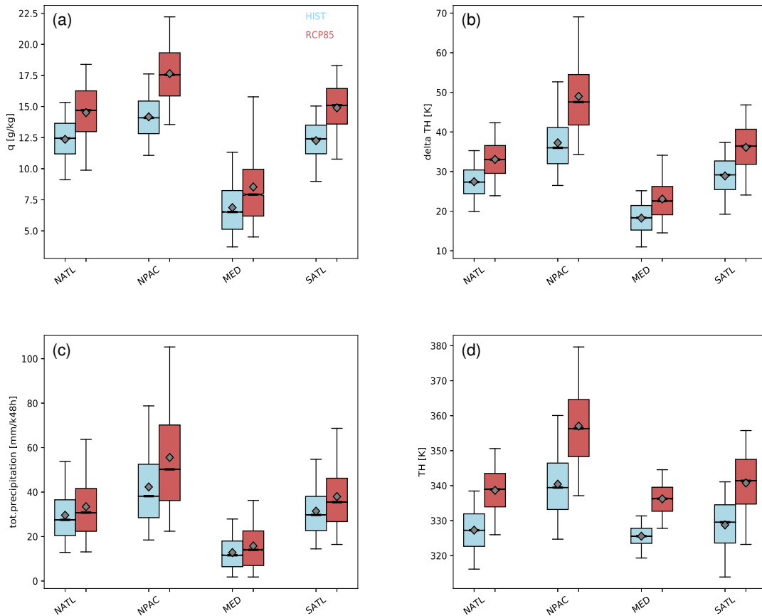
Figure 9. Same as Figure Fig. 8 but for summer, i.e., JJA for NATL, NPAC and MED, and DJF for SATL.
