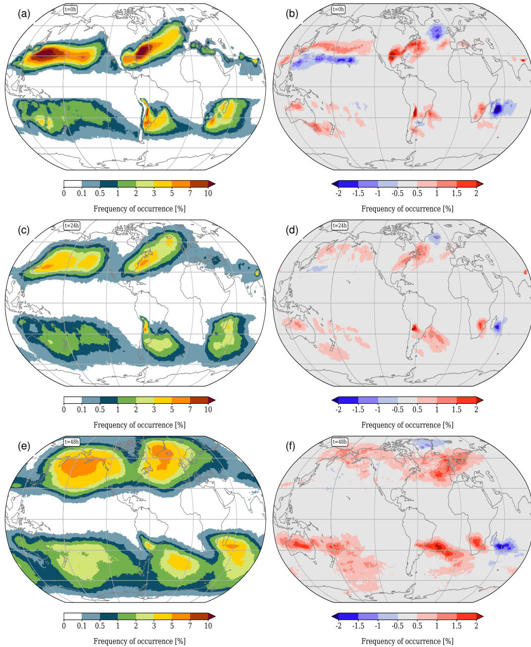
Figure 4. Absolute values of WCB frequency-frequencies (in %) of-for HIST (a, c, e) and difference between-RCP85 and- HIST during boreal winter (DJF) for WCB ascent times t=0t = 0 h (a, b), t=24t = 24 h (c, d), t=48 and t = 48 h (e,f).
