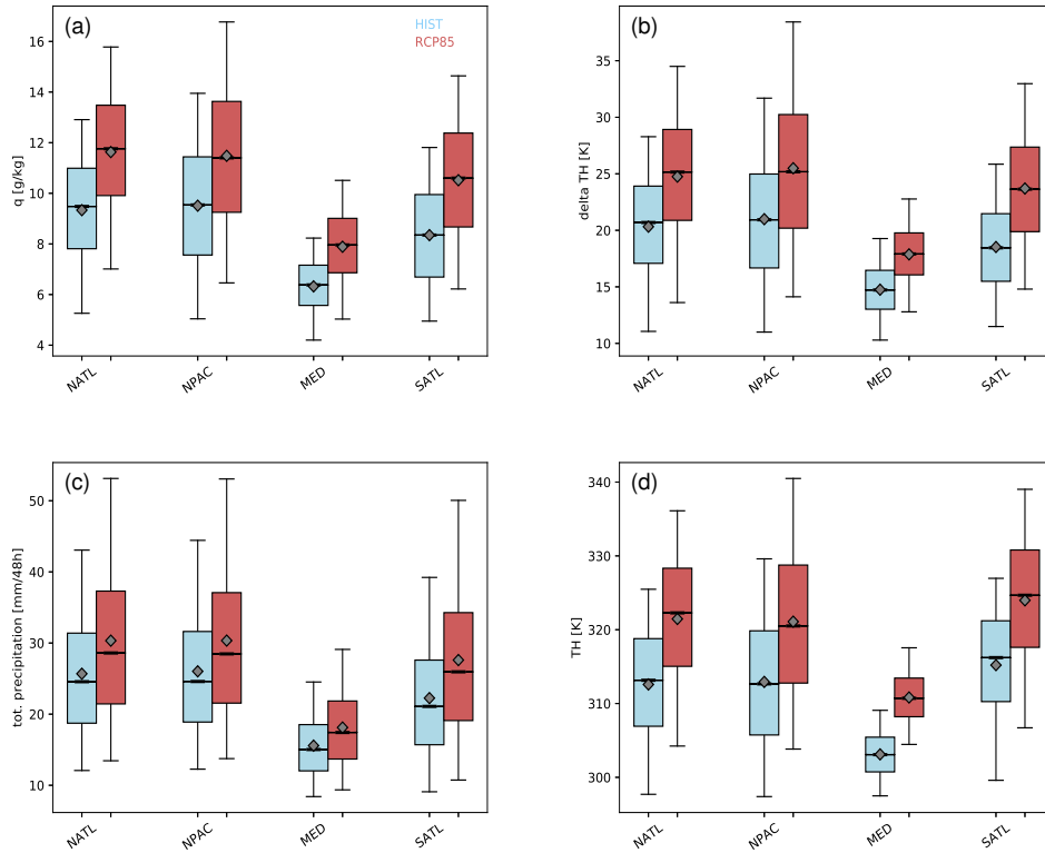
Figure 8. Box-and-whisker (BW) plot plots for different WCB characteristics for of WCBs in the North Atlantic (NATL), North Pacific (NPAC), Mediterranean (MED), and the South America-Atlantic (SATL). The panels show (a) specific humidity in the WCB inflow, (b) increase of potential temperature along the WCB, (c) accumulated surface precipitation along the WCB, and (d) potential temperature at the end of the WCB ascent. Only winter is considered, i.e., DJF for NATL, NPAC and MED, and JJA for SATL. The results for HIST are shown in blue bars, and for RCP85 in red bars. The BW bars diagrams show: lower-to-upper quartile-interquartile range (colored bar), median (bold black line), mean (diamond), and the 5th-to-95th percentile range (thin lines).
