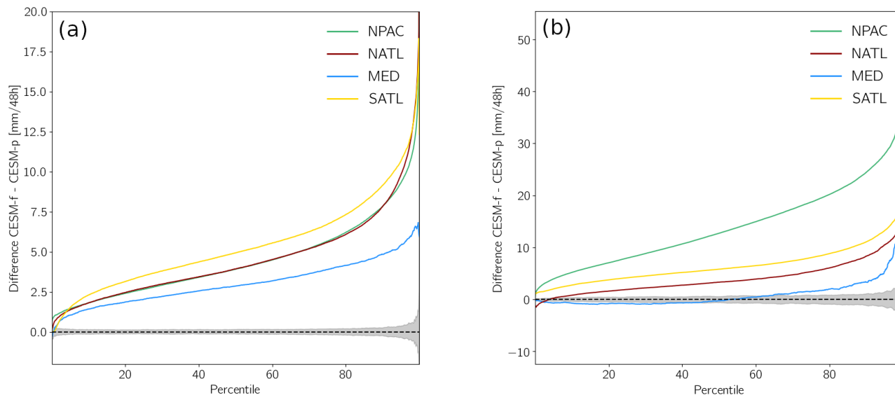
Figure 10. Difference of precipitation percentiles for the four target regions, for winter in (a) winter and for summer (b) summer . The grey-shaded area corresponds to a the 95% confidence interval under the null hypothesis that the two precipitation distributions for HIST and RCP85 do not differ. Exemplarily, the This confidence interval is only shown for the region MED; the confidence intervals for the other regions fall it falls within the one for MED. The confidence interval is calculated based on a resampling approach (see text for details). Note the different vertical axis scales in the two panels.
