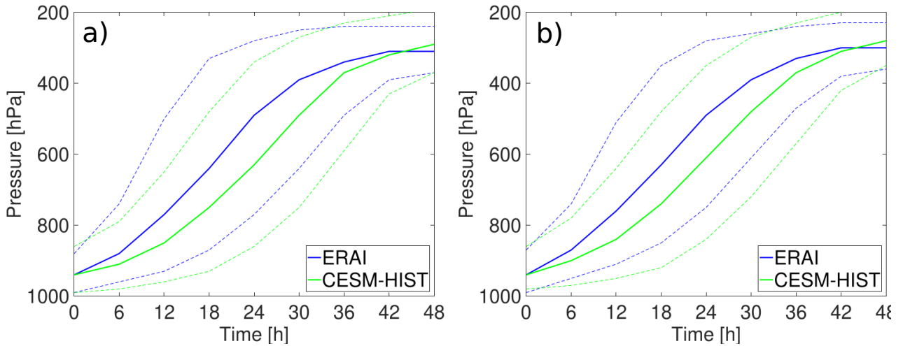
Figure 3. Mean time evolution of pressure (in hPa) along all WCB trajectories during in (a) winter and (b) summer. Solid lines denote the mean over all trajectories and dashed lines the 10th and 90th percentiles for ERA-Interim (blue) and HIST (green).
