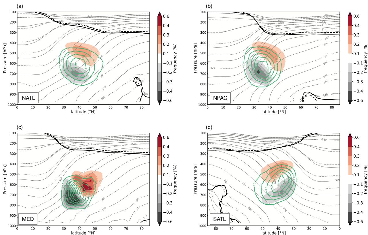
Figure 12. 50-year mean potential temperature (thin-grey solid-and-dashed-lines), potential vorticity (2 pvu isolines; solid-and-dashed-bold black lines), zonally averaged over the four target regions (a) NATL, (b) NPAC, SATL and (c) MED, and (d) SATL. Dashed lines correspond to RCP85 and solid lines to HIST. Green solid lines show the normalized frequency (binsize 5^\circ , 25 hPa) distribution of the WCB air parcels during the time of maximum diabatic heating for HIST (outermost line for 0.2% with an increment of 0.2 for NATL, NPAC, SATL, and 0.3 for MED). The corresponding shift in a future-climate change effect of the distribution of maximum latent heating, RCP85 - HIST , is shown in color shading. All panels are for winter in the corresponding hemisphere, i.e., DJF in (a, b, c) and JJA in (d) and the PV has been multiplied by -1 in SATL.
