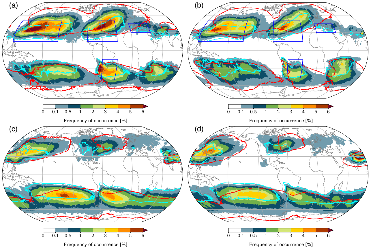
Figure 2. Climatological frequency of WCBs for in DJF (a, b) and JJA (c, d) for ERA-Interim (a, c) and HIST (b, d). Colours denote the percentage of six-hourly timesteps time steps during which at least one WCB trajectory is located in a circle of 100 km around the considered grid point, 24 h after the start of the ascent. The black-turquoise line shows a frequency of 1% for WCBs at their starting time t=0t=0 h and the red line shows a frequency of 1% for WCBs at the end of their ascent at t=48t=48 h. The blue boxes in panel (a) show the regions which that are used for the regional analysis of WCBs in Figures Fig. 8 and 9, 10, 11 and 12.
