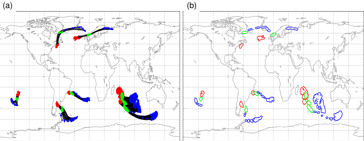
Figure 1. Example of identified WCB trajectories started on at 00 UTC on 15 December 1990 in an ensemble member of HIST. (a) 48-hour forward trajectories, colored according to pressure (in hPa black). The time instances; the positions at times 0 h (start of ascent), 24 h (during ascent) and 48 h (end of ascent) are marked with red, green and blue circles/dots, respectively. (b) WCB masks, with a 100 km blow-up radius, at the same time instances and with the same colours as in (a). The three WCB masks at times 00 h, 24 h and 48 h, averaged over the whole ERA-Interim and CESM periods and all ensemble members, build the basis for the climatologies in Section Sect. 3 and 4 (see text for details).
