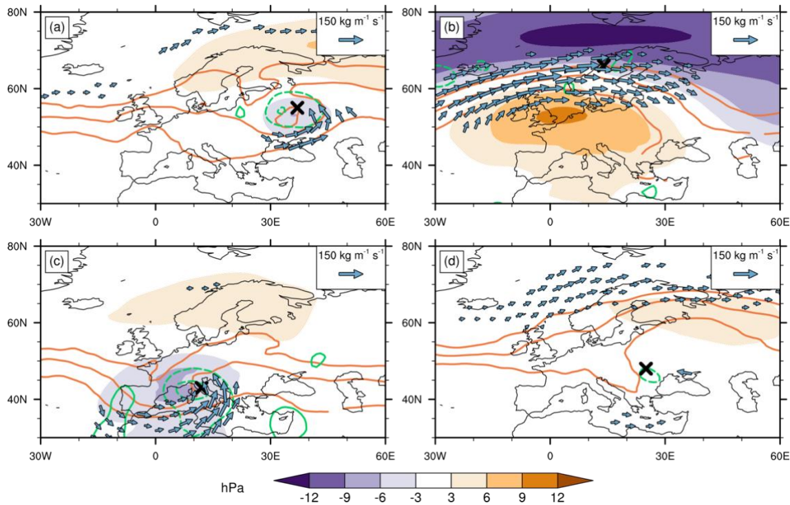
830 Figure 7. Composites of various fields for the (a) \mathcal{S}_{20}(37^{\circ}E, 55^{\circ}N) (Moscow), (b) \mathcal{S}_{20}(14^{\circ}E, 66^{\circ}N) (Norway), (c) \mathcal{S}_{20}(12^{\circ}E, 43^{\circ}N) (Tuscany) and (d) \mathcal{S}_{20}(25^{\circ}E, 48^{\circ}N) (Balkans). Shown are isentropic PV contours of 1, 1.5 and 2 PVU (orange, contours are masked where the respective isentrope intersects the orography on at least one time step of the respective \mathcal{S}_{20} on (a,c,d) 320 K and (b) 310 K, SLP anomalies (shading) and QG\omega anomalies of -1.5, -1, -0.5 hPa hour ^{-1} (green dashed contours) and of +0.5, +1 and +1.5 hPa hour ^{-1} (green solid contours). Furthermore, vectors depict IVT anomalies whose magnitude exceed 30 kg m^{-1} s^{-1} . All anomalies are computed relative to a climatology containing data from all calendar days on which at least one of the \mathcal{S}_{20} at the respective grid point occurred for the 1979–2018 period, i.e., the climatologies vary between the four panels, depending on the seasonality and duration of the respective \mathcal{S}_{20} .
