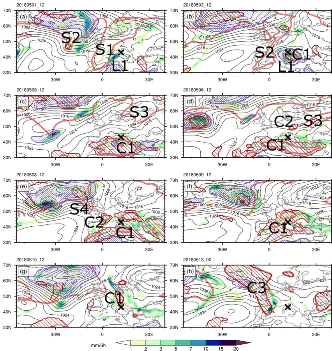
Figure 5. As Fig. 3 but for the longest wet spell at 12^{\circ}\text{E}/43^{\circ}\text{N} in Tuscany, Italy [ S_1(12^{\circ}\text{E}, 43^{\circ}\text{N}) ]. The light red lines depict 2 PVU on 320 K. The valid time of each panel is shown in the top left.
