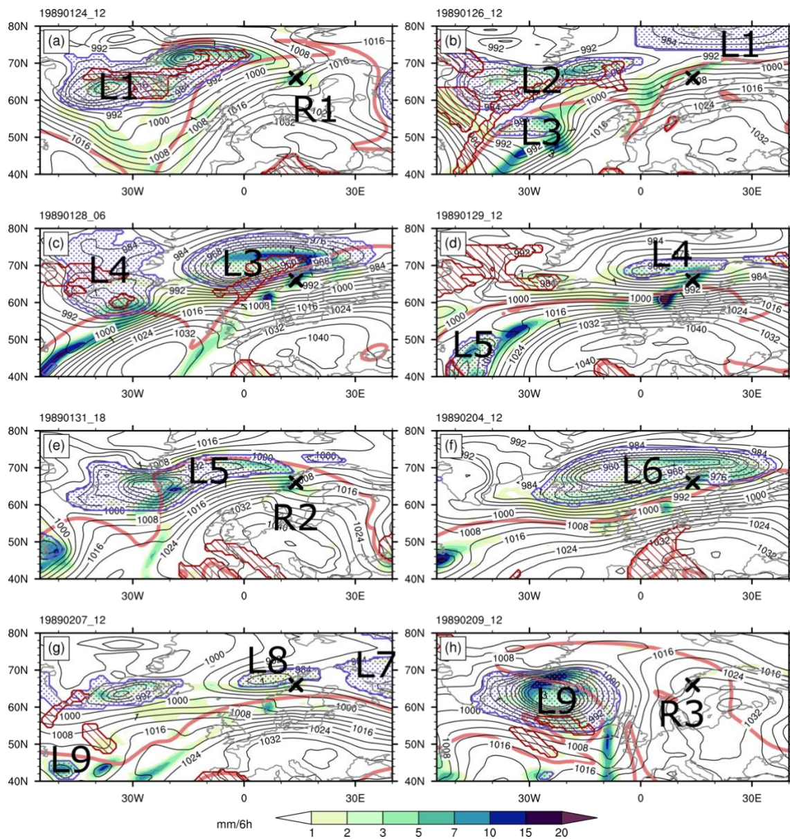
Figure 4. As Fig. 3 but for the longest wet spell at 14^{\circ}\text{E}/66^{\circ}\text{N} in Norway [ S_1(14^{\circ}\text{E}, 66^{\circ}\text{N}) ]. The light red lines depict 2 PVU on 310 K. The valid time of each panel is shown in the top left.
