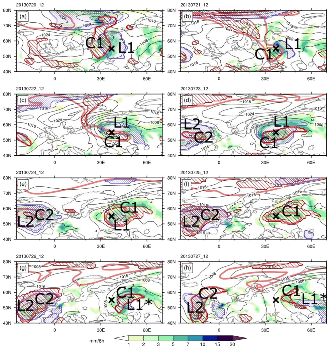
Figure 3. Synoptic evolution of the longest wet spell near Moscow, Russia [ S_1 ( 37^\circ E , 55^\circ N )]. Shading depicts total precipitation accumulated over the preceding 6 hours. Light red contours show the 2 PVU dynamical tropopause on 320 K, while black contours show SLP (contour interval of 4 hPa). Cyclones are depicted by blue stippling and the red hatching depicts the projection of cutoff objects (see methods for details), whose outline therefore does not need to be co-located with the 2 PVU contour on 320 K. The black cross in all panels marks the grid point at 37^\circ E/55^\circ N . Labels help to identify the features discussed in the main text. Panels are shown daily at 12:00 UTC from 20 to 27 July 2013.
