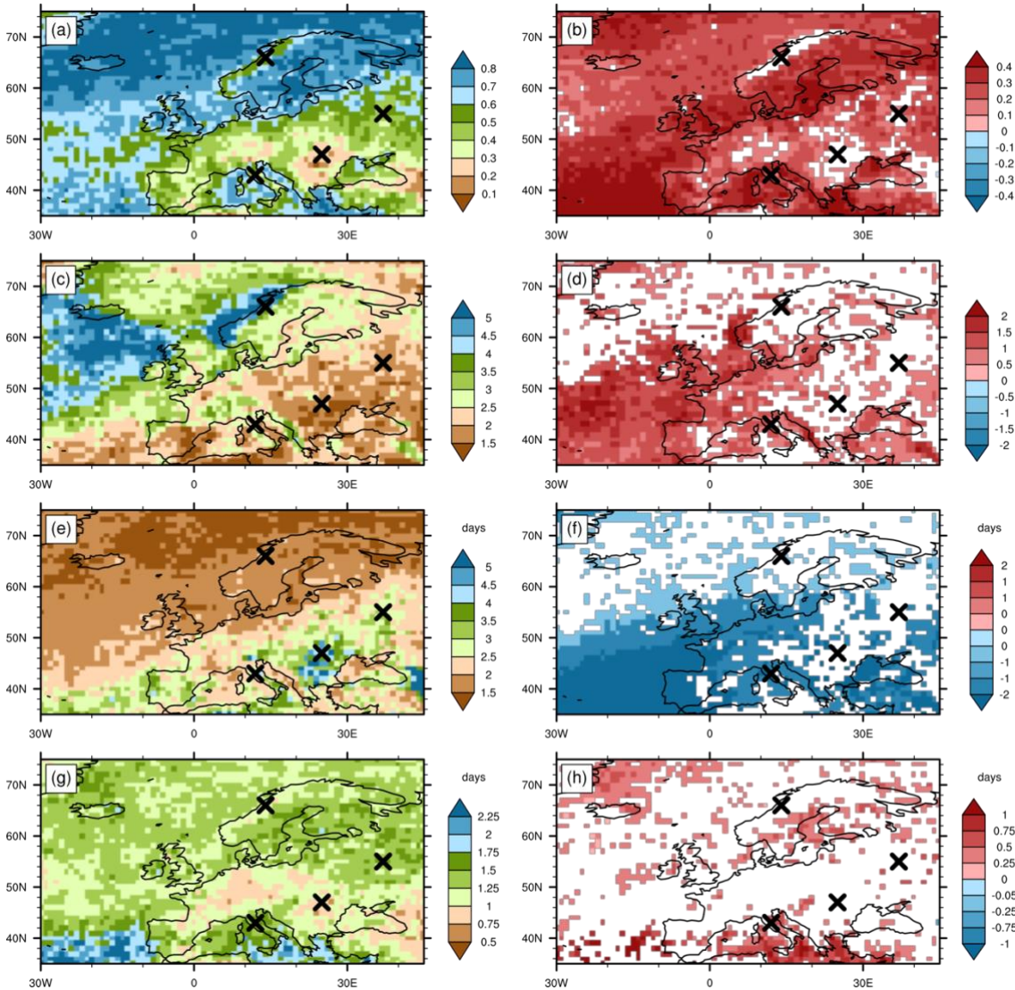
835 Figure 8. Cyclone characteristics during the \mathcal{S}_{20} (left column), and their respective anomalies (right column, see Section 2.5 for the technical definition of the four quantities and their climatological values). (a,b) the cyclone fraction, F_{cyclone} , i.e., fraction of total \mathcal{S}_{20} time steps with a cyclone, (c,d) number of distinct cyclones per \mathcal{S}_{20} spell, N_{cyclone} . (e,f) the cyclone period, P_{cyclone} , i.e., summed \mathcal{S}_{20} duration divided by number of distinct cyclones, and (g,h) the residence time, R_{cyclone} , i.e., the average time each distinct cyclone affects one of the \mathcal{S}_{20} spells. Statistically not significant values in panels (b,d,f,h) are masked out in white (see Section 2.5 for details).
