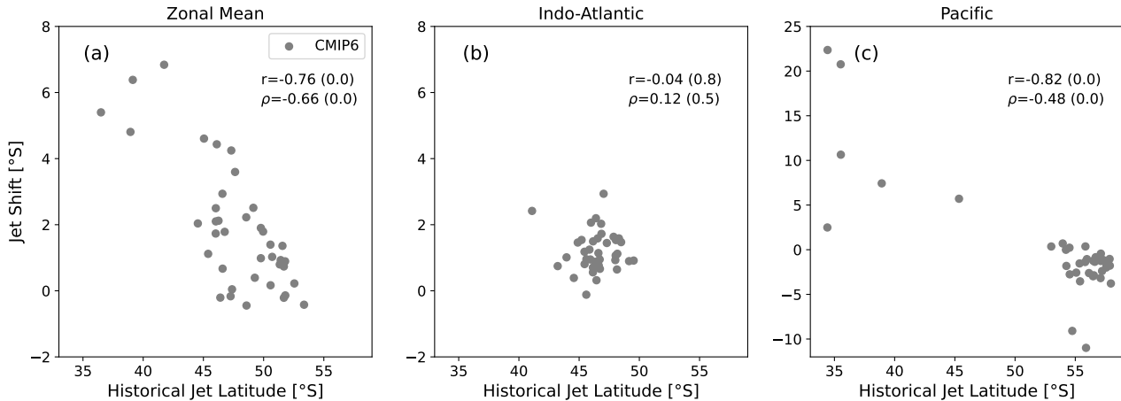
Figure 2. JJA future jet shift plotted against climatological jet latitude for the CMIP6 models. The Pearson correlation coefficient r and the Spearman rank correlation coefficient \rho are given for the CMIP6 values together with their respective p -values. The zonal mean was taken over (a) all longitudes, (b) 300^\circ - 120^\circ and (c) 120^\circ - 300^\circ . Note the larger y -axis range in (c).
