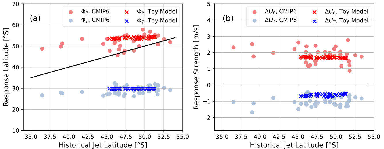
Figure 6. Comparison of the response structure of the CMIP6 ensemble with the toy model results. (a) \Phi_P and \Phi_T , respectively the latitude of the peak and trough of the zonal wind response, against the historical jet latitude. The black line shows the identity. (b) \Delta U_P and \Delta U_T , respectively the amplitude of the peak and trough of the zonal wind response, against the historical jet latitude. The black line marks zero response strength.
