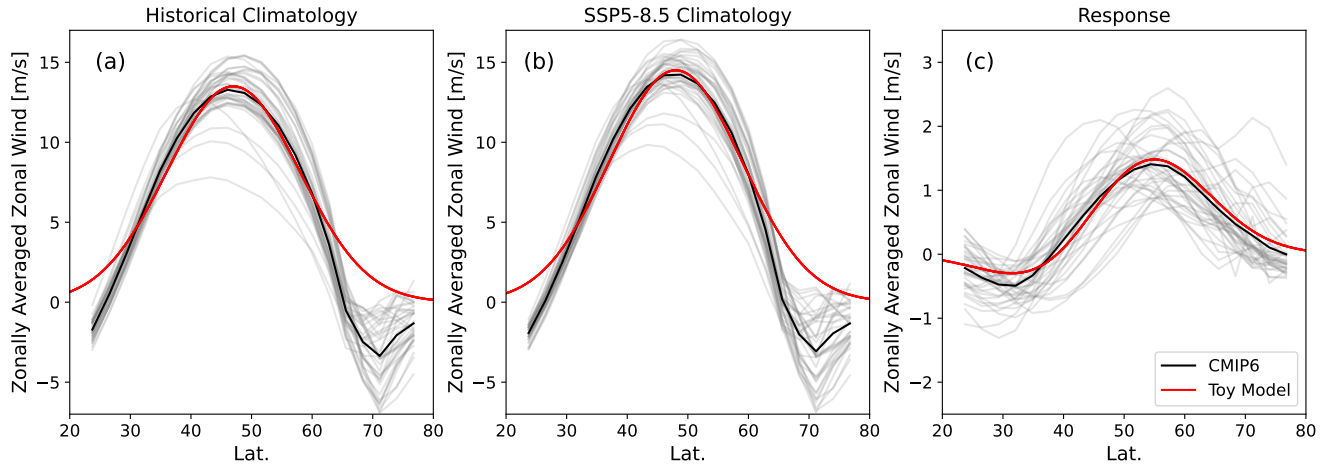
Figure B1. As in Fig. 5 but for the Indo-Atlantic sector ( 300^{\circ} - 120^{\circ} ).
