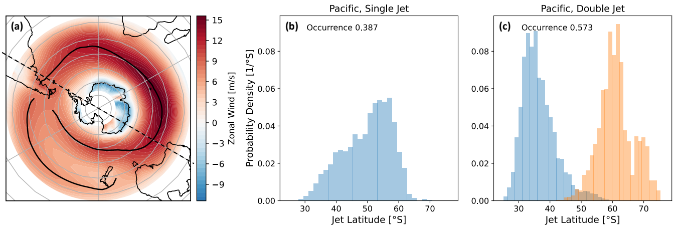
Figure 3. (a) 850 hPa climatological zonal wind averaged over all CMIP6 models; the solid black lines trace the jet positions. The dashed black line divides the hemisphere into the Indo-Atlantic and the Pacific sectors. (b) Jet latitude probability density for days with a single jet structure in the Pacific; (c) same as (b) for days with a double jet structure.
