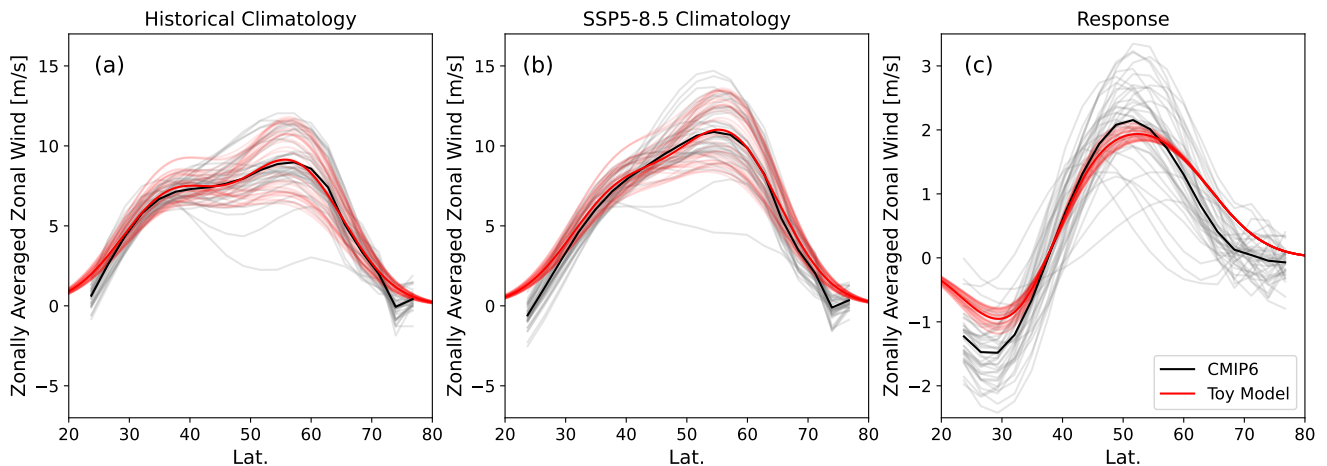
Figure 5. Zonal-mean zonal wind in the Pacific sector ( 120^\circ - 300^\circ ); individual CMIP6 models in grey and their average in black. In light red are the individual realisations of the toy model (see Section 3.3) and in dark red their average. (a) Historical period, (b) the SSP5-8.5 scenario, and (c) the climate-change response as the difference between (b) and (a).
