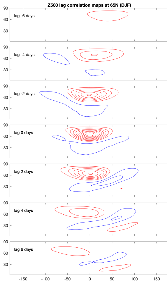
Figure 8. Lag correlation analysis of daily mean Z500 from the NCEP2 reanalysis. Shown is the average of 12 correlation maps calculated at 65^{\circ}\text{N} for 12 base points equally spaced in longitude. The contour interval is 0.1 with the zero correlation lines omitted.
