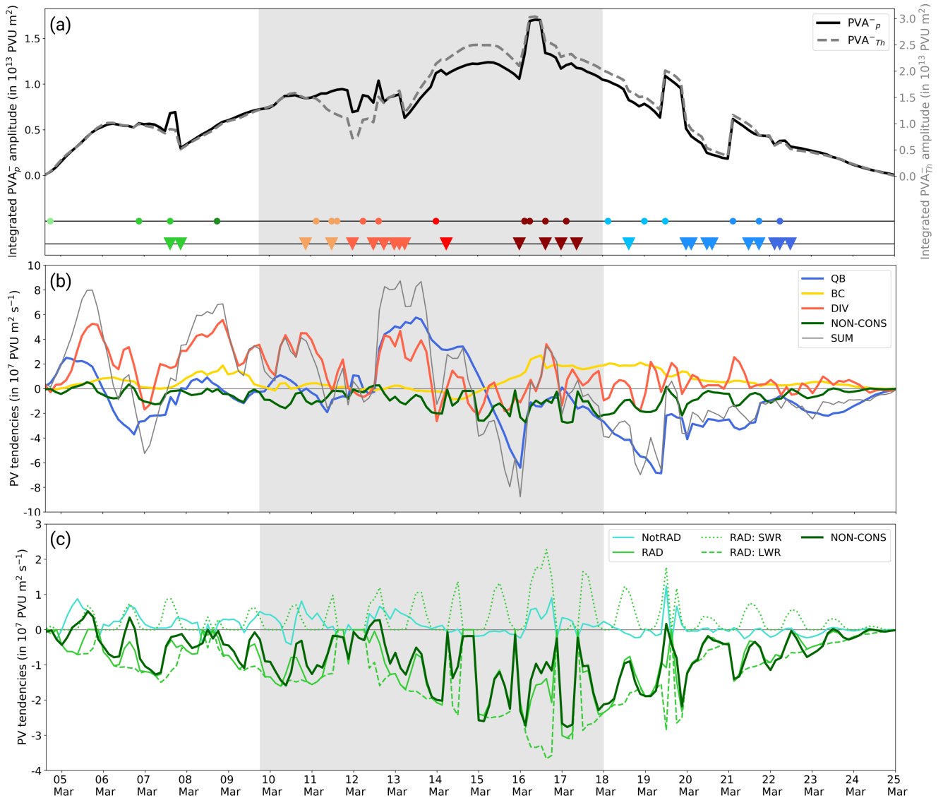
Figure 10. Process contributions to the amplitude evolution of the main PVA_{qL}^- associated with the EuBL episode in March 2016. (a) Integrated PVA_{qL}^- amplitude in terms of isentropic layer average (315–325 K, gray dashed) and pressure layer average (500–150 hPa, black solid) for the life time of the PVA_{qL}^- . Colored symbols along the two horizontal lines in the lower half of the panel mark the occurrence of splitting (triangles) and merging (dots) events. The color of the markers points to the timing of these events (see colorbar in Figs. 8 or 9). (b) Integrated PV tendency terms for PVA_{qL}^- that contribute to the PVA_{qL}^- amplitude evolution: Quasi-barotropic term (QB, blue), baroclinic term (BC, yellow), divergent term (DIV, red), non-conservative term (NON-CONS, green), and the sum of all four terms (SUM, gray). (c) Division of the non-conservative PV tendency term (NON-CONS, solid dark green) into its various components: non-radiative part (NotRAD, solid turquoise) and radiative part (RAD, solid light green). The radiative term is further partitioned into the non-conservative PV tendency by shortwave radiation (RAD: SWR, dotted light green) and by longwave radiation (RAD: LWR, dashed light green). Note the sign convention here is that positive tendencies signify a strengthening of PVA_{qL}^- amplitude. The period of the active EuBL life cycle is shown in all panels in gray shading.
