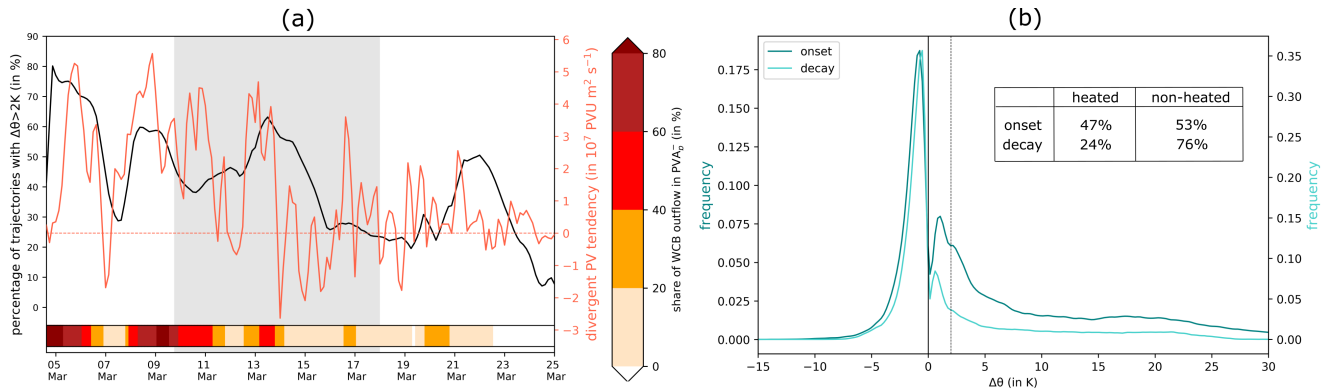
Figure 12. Results of the Lagrangian perspective on the PV dynamics of the EuBL regime life cycle in March 2016. (a) Evolution of divergent PV tendencies from Fig. 10b (red line), fraction of heated ( \Delta\theta > 2 K) three-day backward trajectories starting in PVA_{qL}^- (black), and fraction of WCB outflow within the in PVA_{qL}^- area (red shading, horizontal bar). Note that the divergent PV tendencies are integrated within the PVA_{qL}^- area for grid points with PVA < 0 PVU on the respective isentropic surfaces while WCB outflow and the backward trajectories are included for all grid points within the PVA_{qL}^- area and for latitudes < 80^\circ\text{N} and > 25^\circ\text{N} . The gray shaded area denotes the time of the active EuBL regime life cycle. (b) Frequency distribution of maximum heating and cooling rates along three-day backward trajectories starting in PVA_{qL}^- \pm one day around the onset (dark turquoise) and decay (light turquoise) of the EuBL. The vertical line (black, dashed) corresponds to the 2 K value. The table provides information on the proportion of heated ( \Delta\theta > 2 K) and non-heated ( \Delta\theta < 2 K) trajectories.
