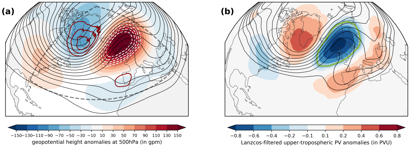
Figure 2. Year-round weather regime composite of EuBL after Grams et al. (2017) based on geopotential height at 500 hPa and upper-tropospheric PV. (a) Lanzeos-filtered Lanczos-filtered (10-days) geopotential height anomalies at 500 hPa (shading, in gpm), absolute geopotential height at 500 hPa (black lines every 40 gpm) and vertically-averaged PVAs between 500–150 hPa for negative (positive) values in dashed white (solid dark red) lines between 0.3 and 0.7 every 0.1 for all time steps attributed to the EuBL regime type (in PVU). The box (dashed gray) shows the area used to define the year-round weather regimes. (b) Lanzeos-filtered Lanczos-filtered (10-days) vertically-averaged PVAs between 500–150 hPa (shading) and vertically-averaged PV for all time steps attributed to the EuBL regime type (contours, in PVU, from 1.5 to 3.5 PVU in steps of 0.25 PVU). The bright green solid line illustrates the regime mask for the EuBL regime type, defined by the -0.3 PVU PVA contour.
