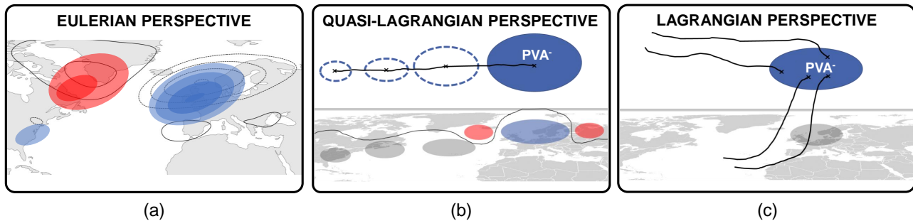
Figure 1. Schematic overview of the three perspectives on the PV dynamics of blocked weather regime life cycles. (a) The Eulerian perspective quantifies the PV dynamics by projecting different upper-tropospheric PV tendency terms onto the mean regime pattern. Black solid (dashed) contours schematically show the PV pattern for the EuBL regime and therefore the location of positive and negative upper-tropospheric PVAs. Red (blue) shading shows exemplary positive (negative) PVAs at a fixed point in time. (b) The quasi-Lagrangian perspective follows negative upper-tropospheric PVAs, assigns them to active regime life cycles and investigates the PVA amplitude evolution. The solid black line connects the center of masses of PVA objects (shown as blue dashed contours for different times) and points to the negative PVA track. Note that the tracked negative PVA is part of an Rossby wave packet as displayed by the sequence of negative (blue shading) and positive (red shading) PVAs. The thin black line on the map shows schematically the position of the wave guide. (c) The Lagrangian perspective calculates backward trajectories out of the negative PVA from the quasi-Lagrangian perspective in (b) and focuses on the diabatic and non-diabatic history of air parcels that end up in the negative PVA. Black lines represent backward trajectories from a negative PVA (starting points marked with a black cross).
