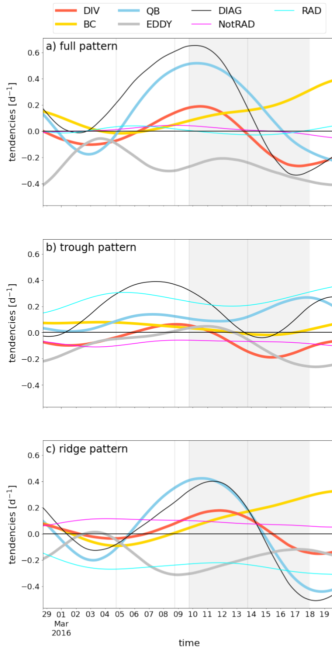
Figure 6. Quantified PV dynamics of the EuBL regime life cycle in March 2016 from a Eulerian perspective. Projection of low-frequency PV-tendencies (in \text{day}^{-1} ) onto (a) the full regime pattern consisting of positive and negative PVAs, (b) only the positive PVAs, and (c) only the negative PVAs of the regime pattern. The colored curves represent the different PV tendencies: divergent (DIV, red), quasi-barotropic (QB, blue), baroclinic (BC, yellow) and the convergence of eddy fluxes (EDDY, gray). The contribution due to direct diabatic modification is separated into radiation (RAD, turquoise) and non-radiative processes (NotRAD, pink). The gray shaded area denotes the time of the active EuBL regime life cycle. Gray vertical lines refer to the times for which spatial fields of PVAs and PV tendencies are shown in Fig. 7.
