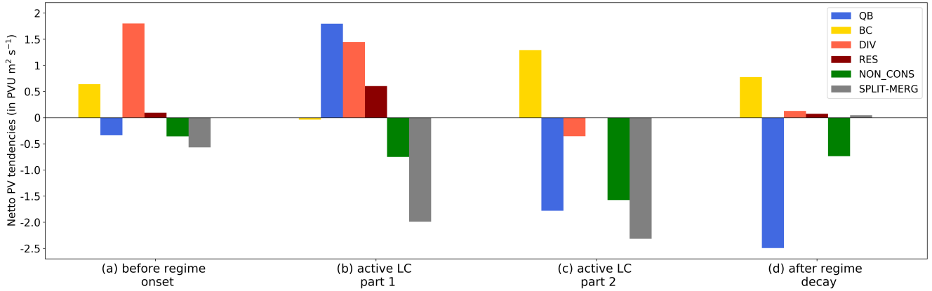
Figure 11. Net effect of PV tendencies and splitting/merging events on the amplitude evolution of the PVA_{qL}^- for different time periods within the PVA_{qL}^- life time. Different PV tendency terms of Fig. 10 are summed up over 4 different time periods (from left to right): (i) prior to EuBL onset (March 4, 15 UTC – March 9, 15 UTC), (ii) active EuBL life cycle part I (March 9, 18 UTC – March 14, 21 UTC), (iii) active EuBL life cycle part II (March 15, 00 UTC – March 18, 00 UTC), and (iv) after EuBL decay (March 18, 03 UCT – March 25, 00 UTC). Isentropic PVA amplitudes of the splitting and merging PVAs are summed up separately for the quantification of the net effect of splitting and merging events. To account for different lengths of the time periods, we divide the sums by the number of time steps in the period.
