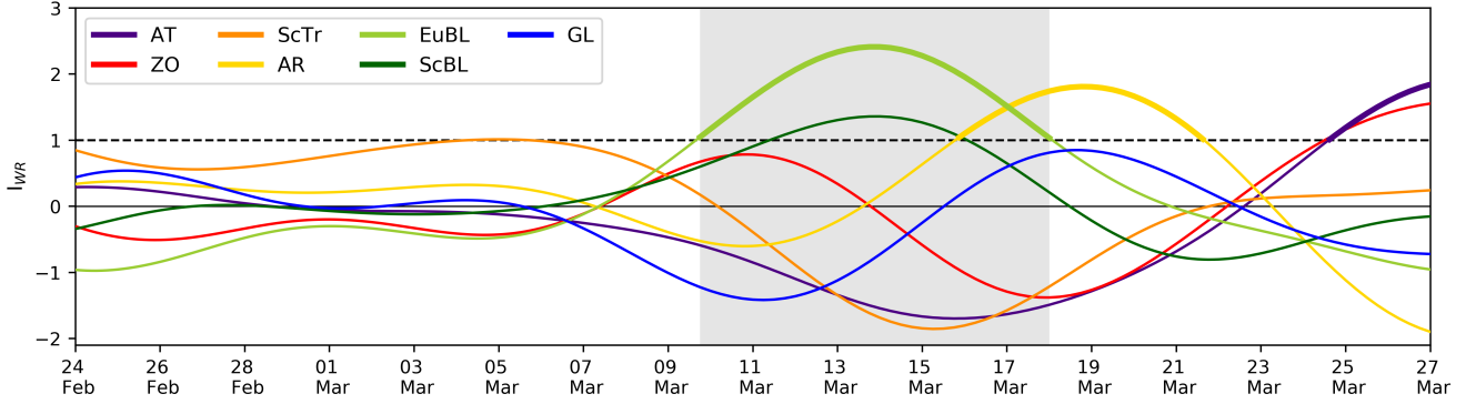
Figure 3. I_{WR} for all seven weather regimes around the EuBL life cycle in March 2016. I_{WR} for year-round weather regime definition from February 24, 00 UTC–March 27, 00 UTC for all seven Euro-Atlantic regimes: Atlantic Trough (AT), Zonal (ZO), Scandinavian Trough (ScTr), Atlantic Ridge (AR), European Blocking (EuBL), Scandinavian Blocking (ScBL) and Greenland Blocking (GL). Thick lines represent active regime life cycles. gray shading indicates the period of the active EuBL regime life cycle from March 9, 18 UTC–March 18, 00 UTC.
