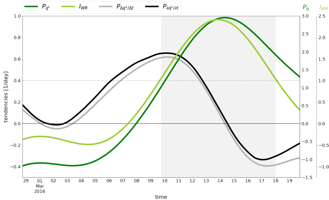
Figure 4. Difference between the I_{WR} evolution and the evolution of the projected low-frequency PVAs to the EuBI regime pattern P_q . Projection of 10-day low-pass filtered PVAs ( P_q , dark green) and I_{WR} in terms of geopotential height anomalies at 500 hPa (light green, cf. Fig 3) on the right y-axes. The gray and black solid line represent the projection of the observed ( P_{\Delta q^L/\Delta t} ) and the diagnosed (DIAG = \sum_j P_{\partial q^L/\partial t}|_j ) evolution of the PVAs, respectively (left y-axis). The gray shaded area denotes the time span of the active life cycle defined by I_{WR} \geq 1 .
