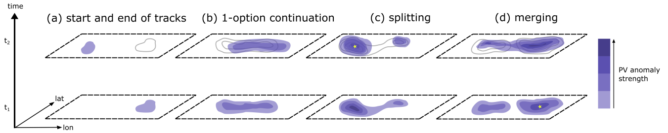
Figure A1. Schematic of the 2D tracking algorithm applied to PVAs_{qL}^{-} in the quasi-Lagrangian perspective. The sketch demonstrates the development of a PVA_{qL}^{-} object (blue shading) from one time step ( t_1 ) to the next ( t_2 ) upwards for different situations: (a) start and end of a track, (b) 1-option continuation, (c) splitting, and (d) merging. The gray thin lines in the upper row at t_2 indicate the position and amplitude of the PVA_{qL}^{-} object at t_1 to show the overlap more visually. Yellow dots in panels (c) and (d) indicate which tracking ID is continued between the time steps, which means that one PVA_{qL}^{-} object gets a new tracking ID (in case of splitting) or a tracking ID ends (in case of merging).
