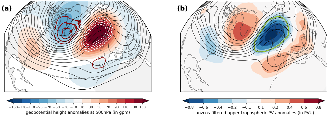
Figure 2. Year-round weather regime composite of EuBL after Grams et al. (2017) based on geopotential height at 500 hPa and upper-tropospheric PV. (a) Lanzcos-filtered (10-days) geopotential height anomalies at 500 hPa (shading, in gpm), absolute geopotential height at 500 hPa (black lines every 40 gpm) and vertically-averaged PVAs between 500–150 hPa for negative (positive) values in dashed white (solid dark red) lines between 0.3 and 0.7 every 0.1 for all time steps attributed to the EuBL regime type (in PVU). The box (dashed gray) shows the area used to define the year-round weather regimes. (b) Lanzcos-filtered (10-days) vertically-averaged PVAs between 500–150 hPa (shading) and vertically-averaged PV for all time steps attributed to the EuBL regime type (contours, in PVU, from 1.5 to 3.5 PVU in steps of 0.25 PVU). The bright green solid line illustrates the regime mask for the EuBL regime type, defined by the -0.3 PVU PVA contour.
