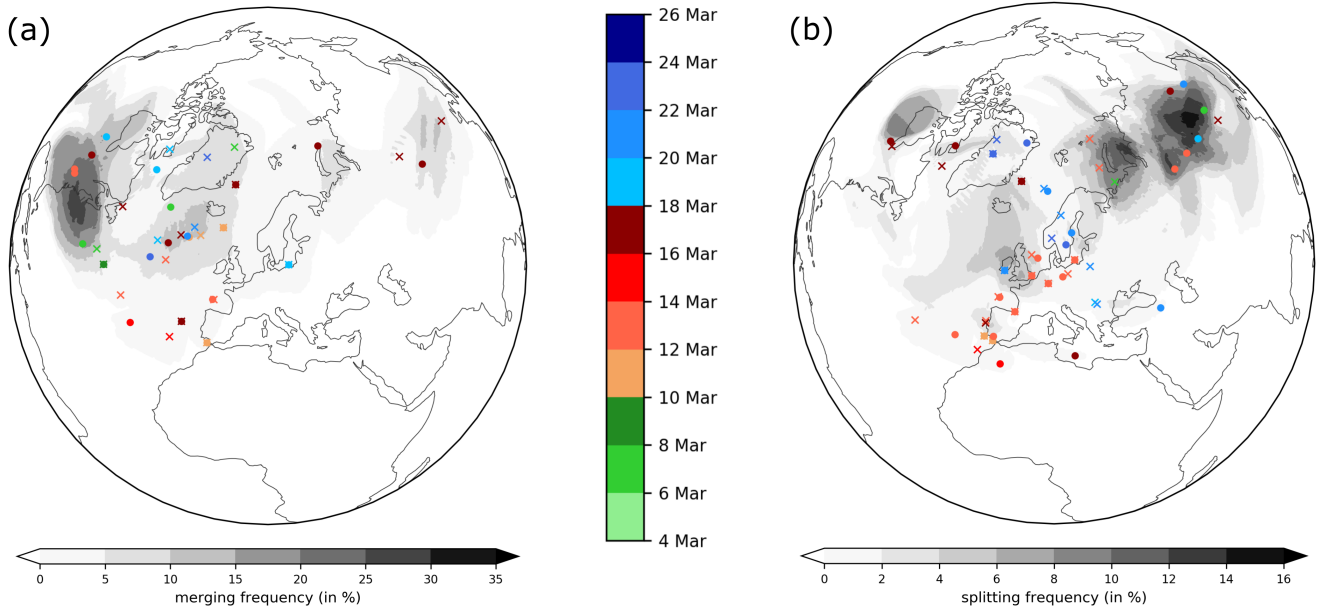
Figure 9. Occurrence frequency (in %) of (a) PVAs_{qL}^- that merge into the main contributing PVA_{qL}^- and (b) PVAs_{qL}^- that separate from the main contributing PVA_{qL}^- . We consider all splitting and merging events that take place along the life cycle of the main PVA_{qL}^- . For the calculation per event, the PVA_{qL}^- is traced back three days in case of merging or from the splitting event to three days later if possible. Crosses show the position (based on the center of mass) of the PVA_{qL}^- before they merge into the main PVA_{qL}^- (panel a) or at the time of splitting from the main PVA_{qL}^- (panel b). Points mark the position of the PVAs_{qL}^- at most three days before the merging event or at most three days after the splitting event. In case of a shorter lifetime of the PVA_{qL}^- the last possible (splitting) or first possible (merging) position is shown. The color indicates the time in the life cycle at which the respective event occurs.
