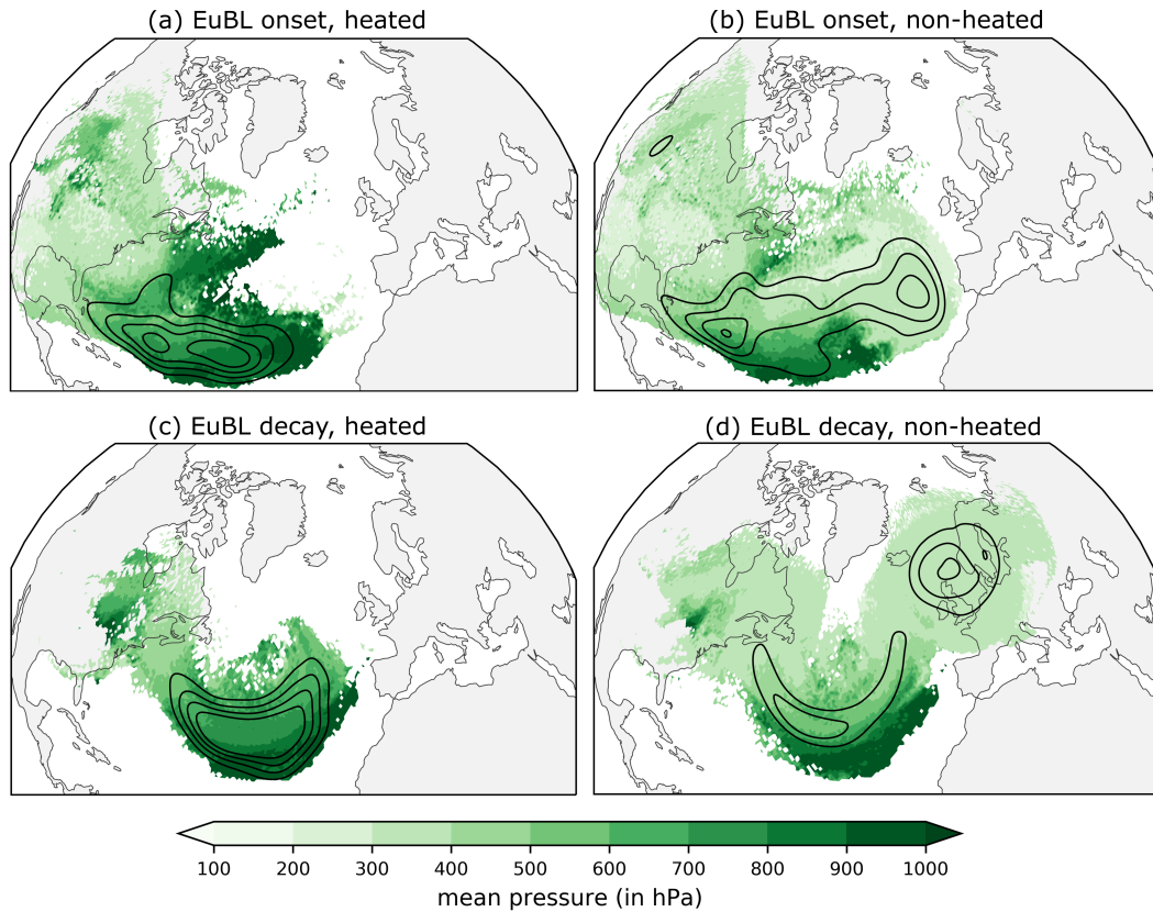
Figure 13. Origin of air parcels that end up in the PVA_{qL}^{-} around the EuBL onset (upper row) and the decay (lower row). The origin of air masses is shown separately for diabatically heated trajectories ( \Delta\theta > 2 K) and non-heated trajectories. We take into account all three-day backward trajectories out of the PVA_{qL}^{-} in the time window \pm one day ( \Delta t = 3 h) around the EuBL onset and decay. Pressure of the air parcels associated with the trajectory (in hPa) is shown at time t = -3 days in green shading. If there are several air parcels at the same grid point (by considering several times), we display the mean pressure. The occurrence frequency is shown in black contours for the heated trajectories in steps of 1.5, 2.5, 3.5 and 4.5 \cdot 10^{-2} and for the non-heated trajectories in steps of 1.0, 1.5, 2.0, 2.5 \cdot 10^{-2} . For a clearer visualization the field has been Gaussian filtered with \sigma = 4 . See Sect. 2.6 for more information on the backward trajectory calculations.
