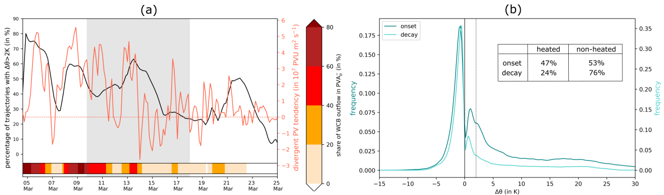
Figure 12. Results of the Lagrangian perspective on the PV dynamics of the EuBL regime life cycle in March 2016. (a) Evolution of divergent PV tendencies from Fig. 10b (red line), fraction of heated ( \Delta\theta > 2 K) three-day backward trajectories starting in PVA_{qL}^- (black), and fraction of WCB outflow within the in PVA_{qL}^- area (red shading, horizontal bar). Note that the divergent PV tendencies are integrated within the PVA_{qL}^- area for grid points with PVA < 0 PVU on the respective isentropic surfaces while WCB outflow and the backward trajectories are included for all grid points within the PVA_{qL}^- area and for latitudes < 80^\circ\text{N} and > 25^\circ\text{N} . The gray shaded area denotes the time of the active EuBL regime life cycle. (b) Frequency distribution of maximum heating and cooling rates along three-day backward trajectories starting in PVA_{qL}^- \pm one day around the onset (dark turquoise) and decay (light turquoise) of the EuBL. The vertical line (black, dashed) corresponds to the 2 K value. The table provides information on the proportion of heated ( \Delta\theta > 2 K) and non-heated ( \Delta\theta < 2 K) trajectories.
