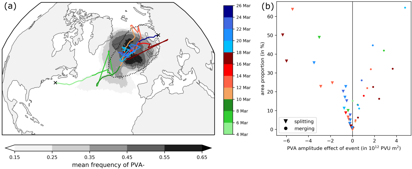
Figure 8. Track of the PVA_{qL}^{-} that contributed to the EuBL in March 2016 and detected splitting and merging events along the tracks. (a) The colored line shows the track of the PVA_{qL}^{-} based on the center of mass from March 4, 15 UTC – March 25, 00 UTC. The time information is given in color shades (green: before regime onset, red: active regime life cycle, blue: after regime decay). Jumps in the PVA_{qL}^{-} track can be attributed to abrupt changes in the center of mass due to splitting and merging events. The mean frequency of the PVA_{qL}^{-} during the time of the track is shown in gray shading (in %). The black dotted contour highlights the regime mask of EuBL (same as in Fig. 2b). (b) Scatter plot that shows the association between the PVA_{qL}^{-} amplitude effect of a splitting (triangle) or a merging (dot) event (in 10^{12} PVU m^2 ) and the area proportion of the splitting/merging PVA_{qL}^{-} and the main PVA_{qL}^{-} (in %). Each marker (triangle, dot) represents a splitting or merging event and the marker color indicates the time of the event.
