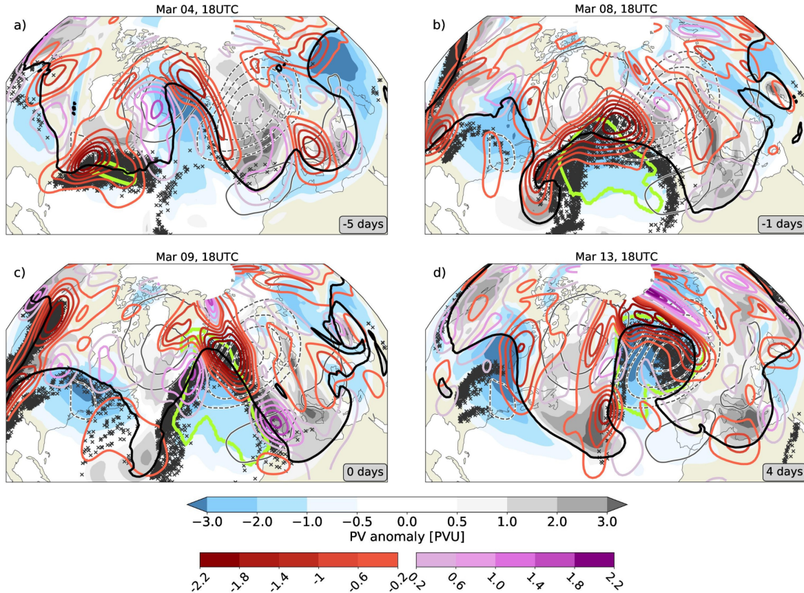
Figure 5. Synoptic evolution of the EuBL regime life cycle in March 2016. Upper-tropospheric PVAs (315–325 K isentropic layer mean, shading) and the 2-PVU contour (solid black) for selected time lags relative to the EuBL regime life cycle onset (March 9, 18 UTC): (a) five days prior to onset, (b) the day prior to onset, (c) onset, and (d) four days after onset. The negative PV anomaly that is later identified in the quasi-Lagrangian perspective in Sect. 4.2 ( PVA_{qL}^- ) as the main contributing negative PVA is shown in a light green contour line (corresponds to the -0.8 PVU anomaly contour). Red and purple solid contour lines point to negative and positive divergent PV tendencies ( -\mathbf{v}_{div} \cdot \nabla q ) likewise shown as isentropic mean between 315–325K (in PVU \text{ day}^{-1} ). Note that divergent PV tendencies are smoothed by a Gaussian filter. Black crosses mark every fifth intersection point of WCB trajectories in the 317.5–322.5 K isentropic layer. The thin dark grey contours indicate the regime pattern of EuBL ( \pm (0.2, 0.4, 0.6, 0.8) PVU, negative dashed).
