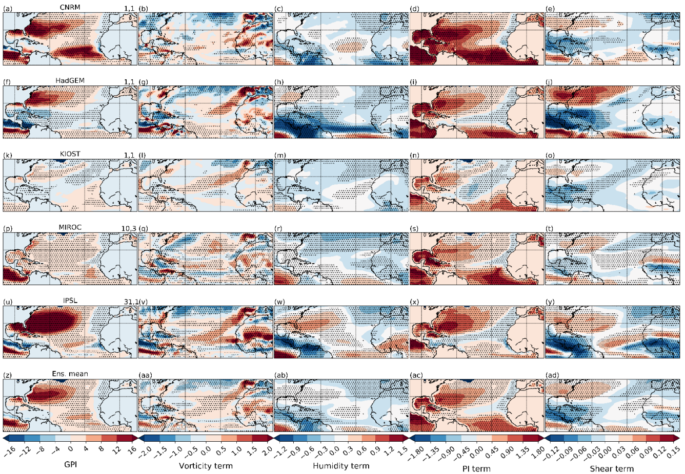
405 Figure 6: Projected change (future minus historical) in the GPI (first column) and the individual terms of the GPI equations (columns 2-5) for CNRM (top row), HadGEM (second row), KIOST (third row) MIROC (fourth row) and IPSL (fifth row) and ensemble mean (sixth row): vorticity term (second column), humidity term (third column), PI term (fourth column) and shear term (fifth column). Note that the vertical wind shear term is a function of the reciprocal of the wind shear, and so a positive difference indicates less vertical wind shear in the future. Number of 410 ensemble members used for the historical and future periods are shown to the upper-right of each column (historical, future). Stippling represents statistical significance at the 95% level using Welch’s t-test.
