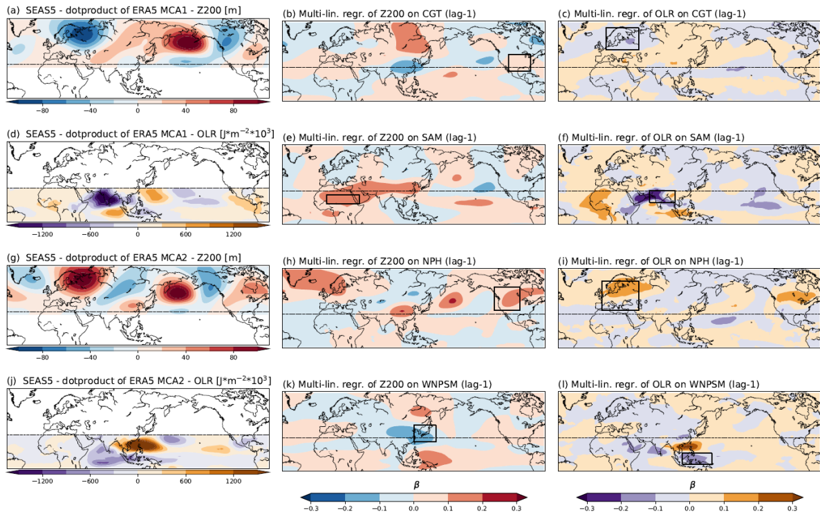
Fig. R2.2 Same as for Fig. R2.1 but for SEAS5 data.
