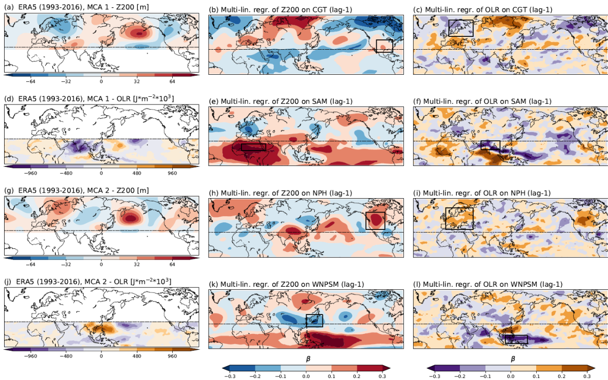
Fig. R2.1. Same as for Figure 3 but showing the multilinear regression coefficient of Z200 on CGT (Panel b) and OLR on CGT (panel c) with the regression coefficients calculated assuming that the grid point time series for Z200 (or OLR) depend on Z200 itself, CGT at lag -1 and SAM at lag -1. Panel e and f: same as for panels b and c but for the effect of SAM on Z200 and OLR. Panels h, i and k, l: same as for panels b, c and e, d but for the effect of NPH and WNPSM on Z200 and OLR fields. Plot obtained using the 600 years as a unique time series.
