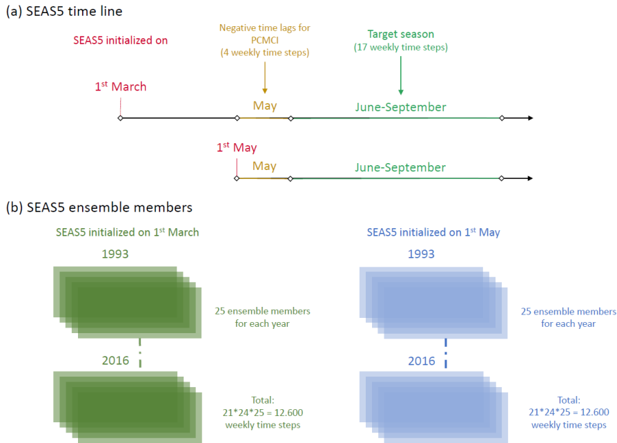
Figure 1. Schematic representation of the SEAS5 forecasting setup. Panel (a) shows the time line for SEAS5 initialization and target period. Panel (b) shows a schematic of the SEAS5 ensemble members.
