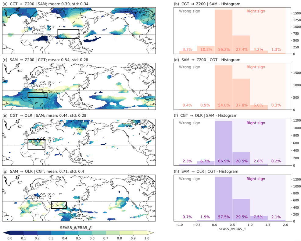
Figure 5. Differences between ERA5 and SEAS5 for MCA mode 1. Left column: \Delta\beta maps, where \Delta\beta = \frac{\beta_{SEAS5}}{\beta_{ERA5}} for CGT \rightarrow Z200|SAM (panel a), SAM \rightarrow Z200|CGT (panel c), CGT \rightarrow OLR|SAM (panel e) and SAM \rightarrow OLR|CGT (panel g). Right column: Histograms for SEAS5-ERA5 \Delta\beta for CGT \rightarrow Z200|SAM (panel b), SAM \rightarrow Z200|CGT (panel d), CGT \rightarrow OLR|SAM (panel f) and SAM \rightarrow OLR (panel h). All grid-points in the domain 15°S-75°N, 0°-360°E are used. The black boxes highlight Southeast Asia (Panel a), the Sahel region (Panel c), the Mediterranean (Panel e) and India (Panel g). The mean and the standard deviation for \Delta\beta values for each plot are shown in the plot title. Only grid points with corrected p -values significant at \alpha = 0.05 in both ERA5 and SEAS5-ERA5 causal maps are shown.
