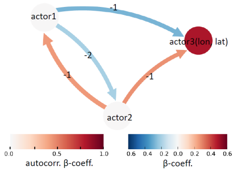
Figure 2. Schematic representation of CEN and \mathcal{C} Causal map. Panel (a) an example of a CEN built with three actors and \text{lag}_{\max} = 2 . Panel (b) shows an example of a causal map: the \beta value for the causal effect of actor1 and actor2 on actor3 (a time-varying field) vary with the latitude and longitude in the map.
