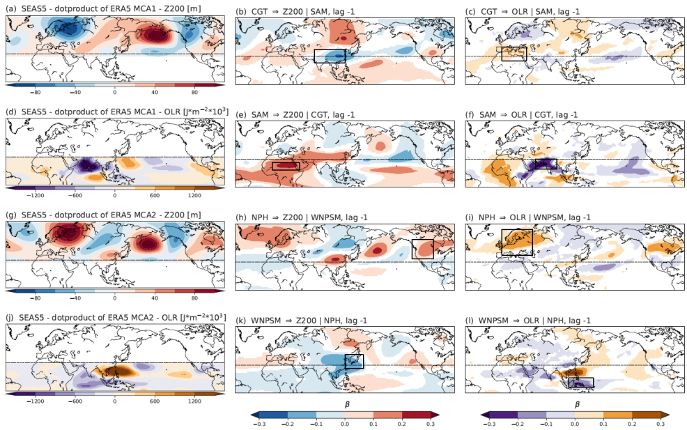
930 Figure 4. Causal maps for SEASS. Same as for Fig. 3 but for SEASS-ERA5 MCA (calculated as the projection of ERA-S on SEASS Z200 and OLR fields) and related causal maps. The black boxes highlight Southeast Asia (Panel b), the Mediterranean (Panel c), the Sahel region (Panel e) and India (Panel f) for MCA mode 1 and central western US (Panel h), eastern Europe (Panel i), Japan (Panel k) and the Maritime Continent (Panel l). Refer to the text in Section 3.2 for an interpretation of the results. Only grid points with corrected p -values significant at \alpha = 0.05 are shown (see Method section for further details).
