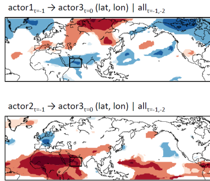
Figure 2. Schematic representation of CEN and \mathcal{C} Causal map. Panel (a) an example of a CEN built with three actors and \text{lag}_{\max} = 2 . Panel (b) shows an example of a causal map: the \beta value for the causal effect of actor1 and actor2 on actor3 (a time-varying field) vary with the latitude and longitude in the map.
