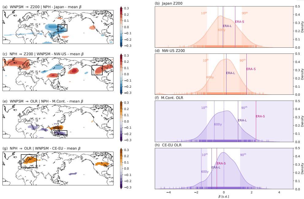
Figure 8. Ensemble spread for MCA mode 2 SEAS5-ERA5. Causal effect averaged over four key regions. Composites of high ( >90^{\text{th}} quantile) minus low ( <10^{\text{th}} quantile) Mean causal effect averaged over the 1000 subsamples over Japan for WNPSM \rightarrow Z200/NPH (panel a), NPH \rightarrow Z200/WNPSM (panel c), WNPSM \rightarrow OLR/NPH (panel e) and NPH \rightarrow OLR/WNPSM (panel g) (Panel a), north-western US (Panel c), Maritime continent (Panel e) and central eastern Europe (Panel g). PDF (standardized) of the distribution with highlighted 10 th and 90 th quantiles for Japan (Panel b), north-western US (Panel d), Maritime Continent (Panel f) and central eastern Europe (Panel h). The value for ERA-L (ERA-S) is shown in the PDFs for comparison by a vertical solid purple (magenta) line. The black boxes highlight Japan (Panel a), central western US (Panel c), the Maritime Continent (Panel e) and Eastern Europe (Panel g). The significance of the \beta values shown in the causal maps in panels a,c,e,g is described in Section 3.3.
