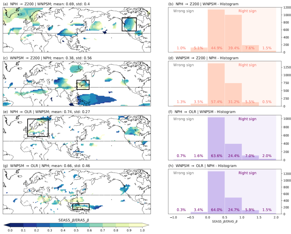
Figure 6. Differences between ERA5 and SEAS5 for MCA mode 2. Left column: \Delta_\beta maps where \Delta_\beta = \frac{\beta_{SEAS5}}{\beta_{ERA5}} for NPH \rightarrow Z200|WNPSM (panel a), WNPSM \rightarrow Z200|NPH (panel c), NPH \rightarrow OLR|WNPSM (panel e) and WNPSM \rightarrow OLR|NPH (panel g). Right column: Histogram for SEAS5-ERA5 \Delta_\beta for NPH \rightarrow Z200|WNPSM (panel b), WNPSM \rightarrow Z200|NPH (panel d), NPH \rightarrow OLR (panel f) and WNPSM \rightarrow OLR|NPH (panel h). All grid-points in the domain 15°S-75°N, 0°-360°E are used. The black boxes highlight central western US (Panel a), Japan (Panel c), Eastern Europe (Panel e), and the Maritime Continent (Panel g). The mean and the standard deviation for \Delta_\beta values for each plot are shown in the plot title. Only grid points with corrected p -values significant at \alpha = 0.05 in both ERA5 and SEAS5-ERA5 causal maps are shown.
