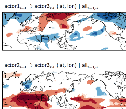
Figure 2. Schematic representation of CEN and causal map. Panel (a) an example of a CEN built with three actors and lag_{max} = -2 . Panel (b) shows an example of a causal map: the \beta value for the causal effect of actor1 and actor2 on actor3 (a time-varying field) vary with the latitude and longitude in the map.
