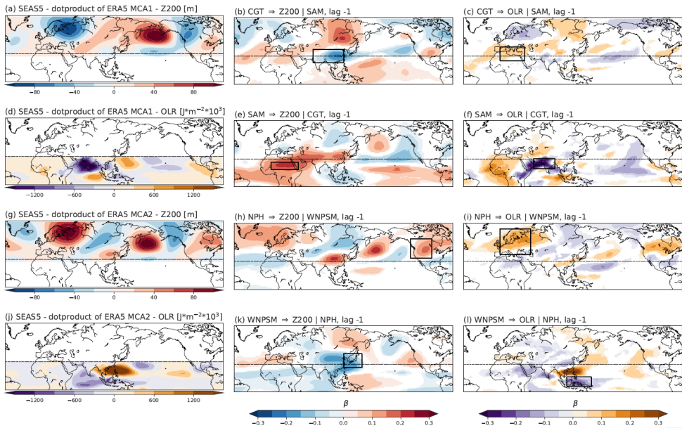
Figure 4. Causal maps for SEASS-R. SEASS-R MCA (calculated as the projection of ERA-S on SEASS Z200 and OLR fields) and related causal maps. Left column: MCA patterns for Z200 and OLR fields for SEASS-R calculated as composites of time steps with the MCA time series values higher than 1 standard deviation (s.d.). MCA mode 1 Z200 (panel a) shows the CGT pattern. MCA mode 1 OLR shows the SAM (panel d). MCA mode 2 Z200 shows the NPH (panel g). MCA mode 2 OLR shows the WNPSM (panel j). Same as for Fig. 3 but for SEASS-ERA5 MCA (calculated as the projection of ERA-S on SEASS Z200 and OLR fields) and related causal maps: Central column (Panels b,e,h,k): causal maps for the effect of each MCA pattern on Z200 fields. Right column (Panels c,f,i,l): causal maps for the effect of each MCA pattern on OLR fields.
