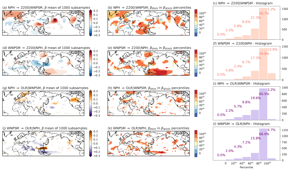
Figure 6. Strength of the \beta coefficients in subsample experiment A for MCA 2. Differences between ERA5 and SEAS5 for MCA mode 2. Left column: \Delta_{\beta} maps where \Delta_{\beta} = \frac{\beta_{SEAS5} - \beta_{ERA5}}{\beta_{SEAS5}} for Panel (a): causal effect for NPH \rightarrow Z200|WNPSM averaged over the 1000 subsamples obtained in the SEAS5 dataset (initialized on the 1 st of May). Direction and significance of the causal links are imposed to be the same as calculated in Fig. 3. Panel (b): \beta_{ERA5} compared to \beta_{SEAS5} quantiles for the NPH \rightarrow Z200|WNPSM link. Panel (c): Histogram showing the percentage of grid points for which the \beta_{ERA5} falls in a certain quantile range as obtained for \beta_{SEAS5} coefficients. (panel a). Panels d,e,f: Same as for panels a,b,c but for the WNPSM \rightarrow Z200|NPH link. Panels g,h,i: Same as for panels a,b,c but for the NPH \rightarrow OLR|WNPSM link. Panels j,k,l: Same as for panels a,b,c but for the WNPSM \rightarrow OLR|NPH link (panel g). Right column: Histogram for SEAS5-ERA5 \Delta_{\beta} for NPH \rightarrow Z200|WNPSM (panel b), WNPSM \rightarrow Z200|NPH (panel d), NPH \rightarrow OLR (panel f) and WNPSM \rightarrow OLR|NPH (panel h). All grid-points in the domain 15°S-75°N, 0°-360°E are used. The black boxes highlight central-western US (Panel a), Japan (Panel e), Eastern Europe (Panel e), and the Maritime Continent (Panel g). The mean and the standard deviation for \Delta_{\beta} values for each plot are shown in the plot title. Only grid points with corrected p -values significant at \alpha = 0.05 in both ERA5 and SEAS5-ERA5 causal maps are shown.
