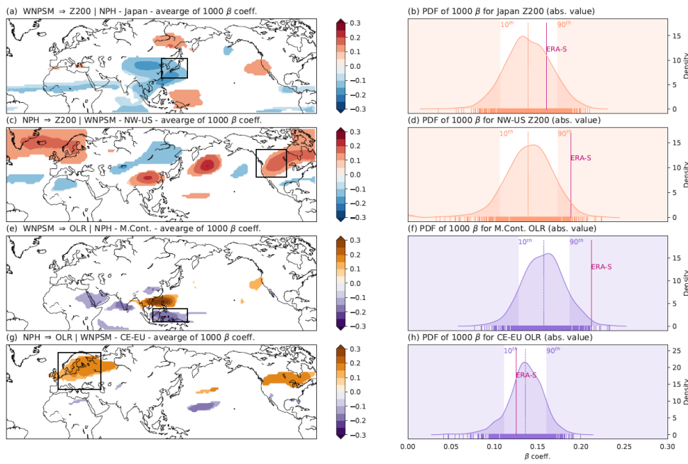
955 Figure 8. Ensemble spread for subsample experiment B for MCA mode 2. Ensemble spread for MCA mode 2 SEAS5-ERA5. The mean causal effect is averaged over four key regions. Mean causal effect averaged over the 1000 subsamples for WNPSM \rightarrow Z200|NPH (panel a), NPH \rightarrow Z200|WNPSM (panel c), WNPSM \rightarrow OLR|NPH (panel e) and NPH \rightarrow OLR|WNPSM (panel g). Only grid point with \beta coefficients significant at \alpha = 0.10 (after applying the Benjamini-Hochberg false discovery rate correction) are shown. PDF (standardized) of the distribution with highlighted 10 th and 90 th quantiles-percentiles for Japan (Panel b), north-western US (Panel d), Maritime Continent (Panel f) and central eastern Europe (Panel h). \beta coefficients The value for ERA-L (ERA-S) is are shown in the PDFs for comparison by a vertical solid purple (magenta) line. The black boxes highlight Japan (Panel a), central western US (Panel c), the Maritime Continent (Panel e) and Eastern Europe (Panel g). The significance of the \beta values shown in the causal maps in panels a,c,e,g is described in Section 3.34. 960
