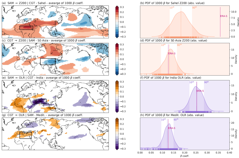
Figure 7. Ensemble spread for subsample experiment B for MCA mode 1-SEASS-ERAS. The mean causal effect is averaged over four key regions. Mean causal effect averaged over the 1000 subsamples for SAM \rightarrow Z200|CGT (panel a), CGT \rightarrow Z200|SAM (panel c), SAM \rightarrow OLR|CGT (panel e) and CGT \rightarrow OLR|SAM (panel g). Only grid point with \beta coefficients significant at \alpha = 0.10 (after applying the Benjamini-Hochberg false discovery rate correction) are shown. PDF (standardized) of the distribution with highlighted 10 th and 90 th quantiles-percentiles for the Sahel region (Panel b), Southeast Asia (Panel d), India (Panel f) and the Mediterranean (Panel h). \beta coefficients The value for ERA-S (ERA-S) is arc shown in the PDFs for comparison by a vertical solid purple (magenta) line. The black boxes highlight the Sahel region (Panel a), Southeast Asia (Panel c), India (Panel e) and the Mediterranean (Panel g). The significance of the \beta values coefficients shown in the causal maps in panels a,c,e,g is described in Section 3.34.
