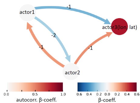
Figure 2. Schematic representation of CEN and causal map. Panel (a) an example of a CEN built with three actors and lag_{max} = -2 . Panel (b) shows an example of a causal map: the \beta value for the causal effect of actor1 and actor2 on actor3 (a time-varying field) vary with the latitude and longitude in the map.
