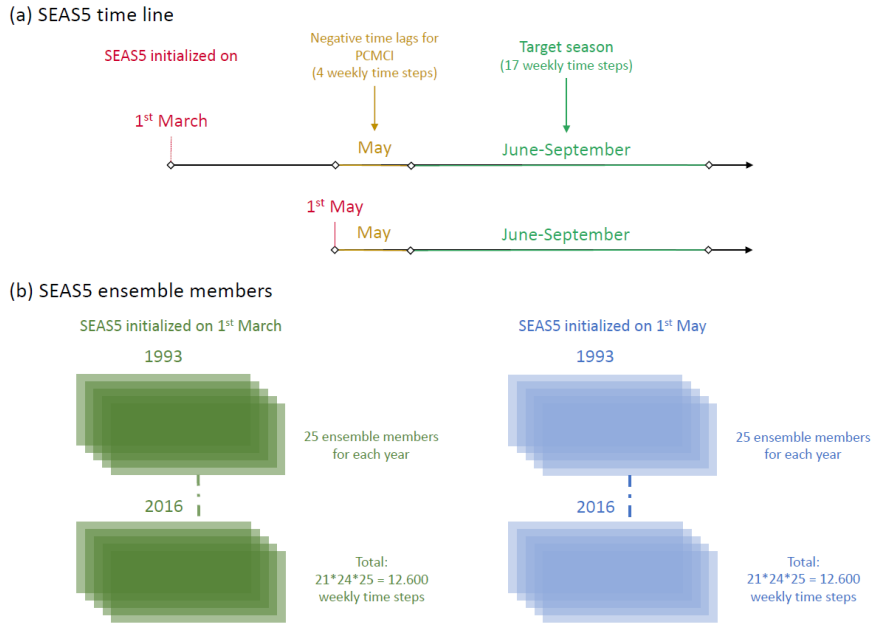
Figure 1. Schematic representation of the SEASS forecasting setup. Panel (a) shows the time line for SEASS initialization and target period. Panel (b) shows a schematic of the SEASS ensemble members.
