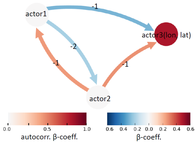
Figure 2. Schematic representation of CEN and causal map. Panel (a) shows an example of a CEN built with three actors and lag_{max} -2 .
