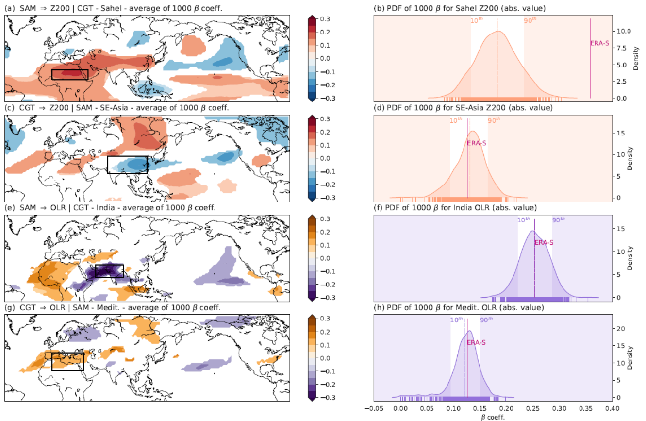
Figure 87. Ensemble spread for subsampling Experiment B for MCA mode 1. The mean causal effect is averaged over four key regions. Mean causal effect averaged over the 1000 subsamples for SAM \rightarrow Z200|CGT (panel a), CGT \rightarrow Z200| SAM (panel c), SAM \rightarrow OLR| CGT (panel e) and CGT \rightarrow OLR| SAM (panel g). Only grid point with \beta coefficients significant at \alpha = 0.10 (after applying the Benjamini-Hochberg false discovery rate correction) are shown. PDF for the absolute values of the 1000 \beta coefficients are shown with highlighted 10 th and 90 th percentiles for the Sahel region (Panel b), Southeast Asia (Panel d), India (Panel f) and the Mediterranean (Panel h). \beta coefficients for ERA-S are shown in the PDFs for comparison by a vertical solid magenta line. The black boxes highlight the Sahel region (Panel a), Southeast Asia (Panel c), India (Panel e) and the Mediterranean (Panel g). The significance of the \beta coefficients shown in the causal maps in panels a,c,e,g is described in Section 3.4.
