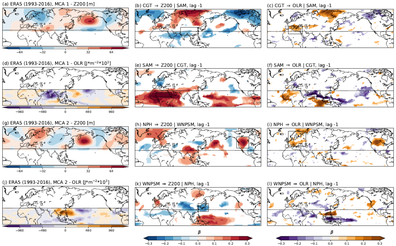
895 Figure 3. Causal maps for ERA5. Left column: MCA patterns for Z200 and OLR fields for ERA-S. MCA mode 1 Z200 (panel a) shows the CGT pattern. MCA mode 1 OLR shows the SAM (panel d). MCA mode 2 Z200 shows the NPH (panel g). MCA mode 2 OLR shows the WNPSM (panel j). Central column (Panels b,e,h,k): causal maps for the effect of each MCA pattern on Z200 fields. Right column (Panels c,f,i,l): causal maps for the effect of each MCA pattern on OLR fields. The black boxes highlight Southeast Asia (Panel b), the Mediterranean (Panel c), the Sahel region (Panel e) and India (Panel f) for MCA mode 1 and central western US (Panel h), eastern Europe (Panel i), Japan (Panel k) and the Maritime Continent (Panel l) for MCA mode 2 . Refer to the text in Section 3.2 for an interpretation of the results. Only grid points with corrected p-values significant at \alpha = 0.1 are shown. 900
