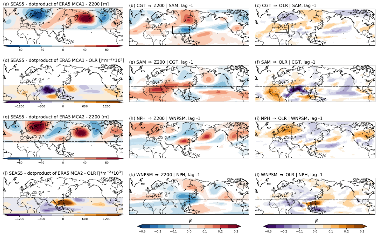
905 Figure 4. Causal maps for SEAS5-R. SEAS5-R MCA (calculated as the projection of ERA-S on SEAS5 Z200 and OLR fields) and related causal maps. Left column: MCA patterns for Z200 and OLR fields for SEAS5-R calculated as composites of time steps with the MCA time series values higher than 1 standard deviation (s.d.). MCA mode 1 Z200 (panel a) shows the CGT pattern. MCA mode 1 OLR shows the SAM (panel d). MCA mode 2 Z200 shows the NPH (panel g). MCA mode 2 OLR shows the WNPSM (panel j). Central column (Panels b,e,h,k): causal maps for the effect of each MCA pattern on Z200 fields. Right column (Panels c,f,i,l): causal maps for the effect of each MCA pattern on OLR fields. The black boxes highlight Southeast Asia (Panel b), the Mediterranean (Panel c), the Sahel region (Panel e) and India (Panel f) for MCA mode 1 and central western US (Panel h), eastern Europe (Panel i), Japan (Panel k) and the Maritime Continent (Panel l) for MCA mode 2 . Refer to the text in Section 3.2 for an interpretation of the results. Only grid points with corrected p -values significant at \alpha = 0.05 are shown (see Method section for further details). 910
