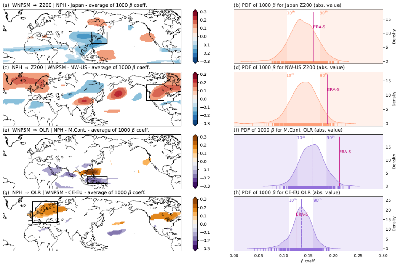
Figure 89. Ensemble spread for subsampling Experiment B for MCA mode 2. Same as for Fig 7 but for MCA mode 2. Mean causal effect averaged over the 1000 subsamples for WNPSM \rightarrow Z200|NPH (panel a), NPH \rightarrow Z200|WNPSM (panel c), WNPSM \rightarrow OLR|NPH (panel e) and NPH \rightarrow OLR|WNPSM - CE-EU - average of 1000 \beta coeff. (panel g). PDF for the absolute values of the 1000 \beta coefficients are shown for Japan (Panel b), north-western US (Panel d), Maritime Continent (Panel f) and central eastern Europe (Panel h).
