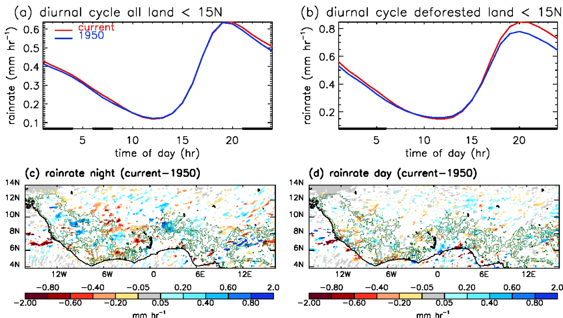
Figure 7: Diurnal cycle of rainfall with times where differences are significant at p=0.1 indicated by black bar for (a) all land points below 15^\circ \text{N} and (b) deforested pixels only. Maps of rainfall differences for (c) 19:00-6:00 UTC and (d) 7:00-18:00 UTC. Insignificant changes are shown in white, whereas small but significant changes either side of zero are shown in grey. Green contours show where there has been deforestation.
