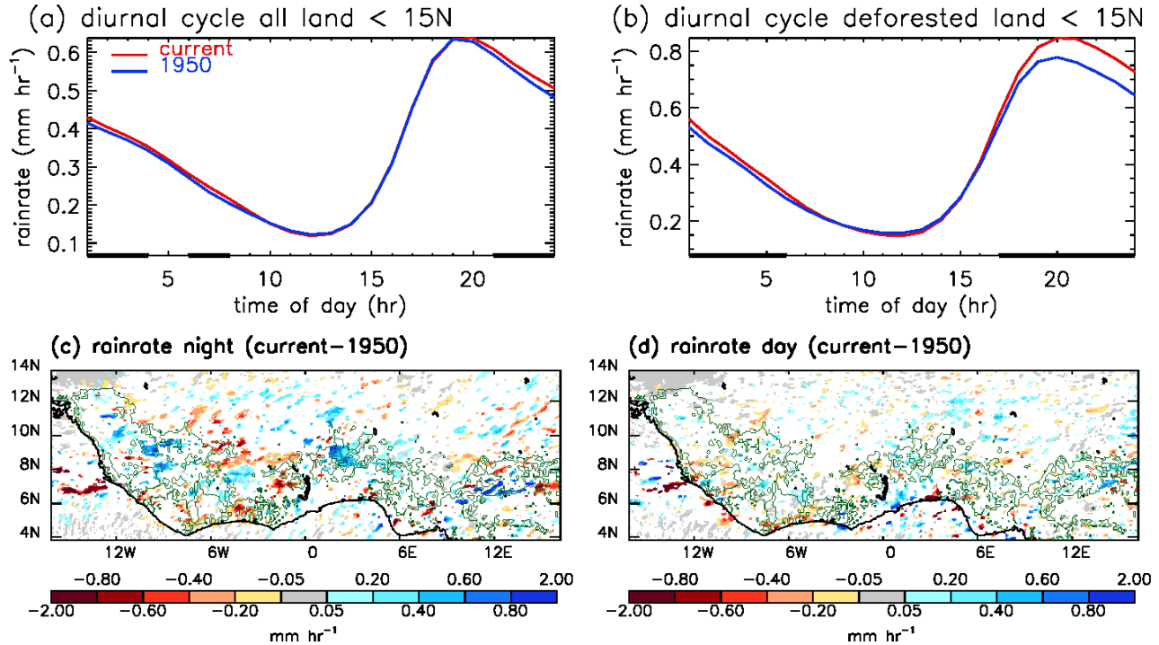
Figure 7: Diurnal cycle of rainfall with times where differences are significant at p=0.1 indicated by black bar for (a) all land points below 15° N and (b) deforested pixels only. Maps of rainfall differences for (c) 19:00-6:00 UTC and (d) 7:00-18:00 UTC. Insignificant changes at the individual pixels level are shown in white, whereas small but significant changes either side of zero are shown in grey. Green contours show where there has been deforestation.
