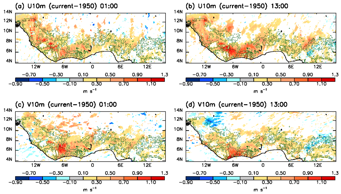
Figure S7: Changes in components of 10m winds
