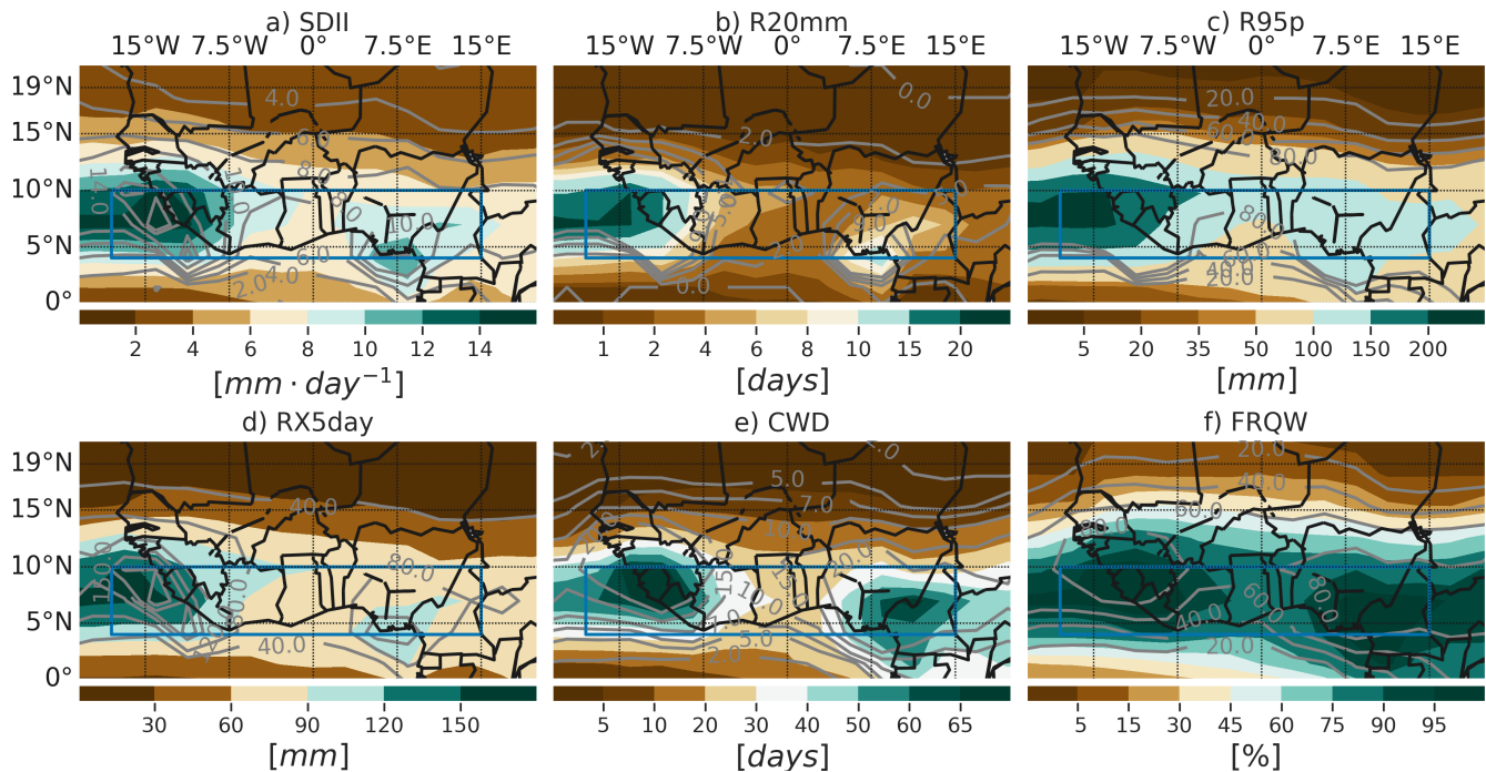
Figure 2. EnsMedian distribution of the mean JAS extreme rainfall indices over the 1995-2014 period from 24 CMIP6 models. The blue rectangles indicate the Guinea Coast region. Contours in grey show the observations EnsMedian values.
