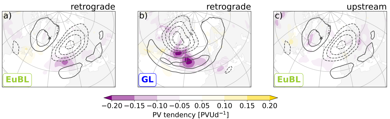
Figure 12. Same as Figure 6, but for the divergent tendency for the retrograde cluster for EuBL (a) and GL (b), and the upstream cluster for EuBL (c). Note the different color bar.
