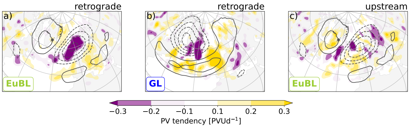
Figure 11. Same as Figure 6, but for the convergence of the eddy PV flux for the retrograde cluster for EuBL (a) and GL (b), and the upstream cluster for EuBL (c). Note the different color bar.
