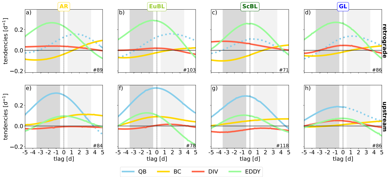
Figure 9. Same as Figure 7, but for the retrograde (top row) and the upstream cluster (bottom row).
