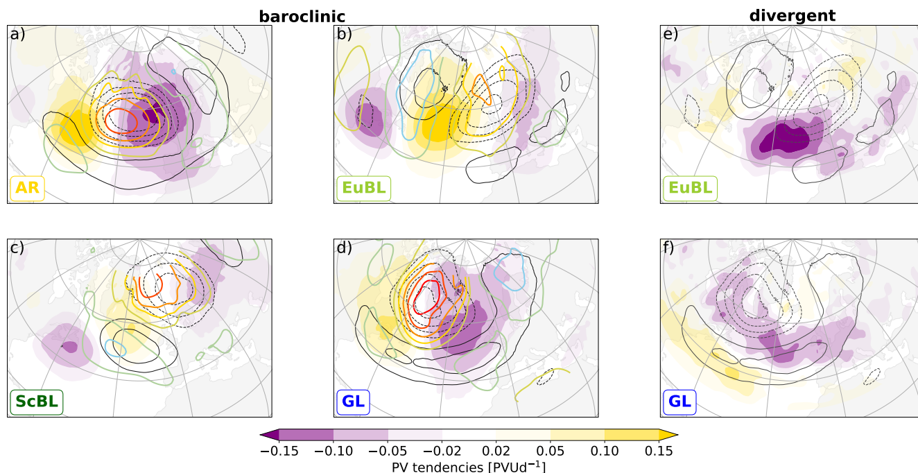
Figure 6. Same as Figure 5, but for baroclinic coupling for AR (a), EuBL (b), ScBL (c), and GL (d) and the divergent tendencies (EuBL (e) and GL (f)). Note the different color bar compared to Figure 5. Colored contours in a)-d) denote potential temperature at 850 hPa, warm colors for positive and cold colors for negative values, with a contour interval of 1 K, omitting the zero line.
