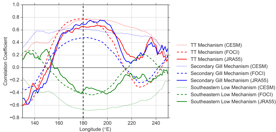
Figure 4. Pointwise longitudinal correlation between the peak of the major mechanisms (same mechanisms as Figure 3) and the ONDJF Pacific 200 hPa divergence averaged between 10^{\circ}S - 10^{\circ}N . The respective peak season for each index is used, i.e. FMA for TT (red), and JFM for the Secondary Gill (blue), and Southeastern Low (green). CESM-WACCM (dotted line) and FOCI (dashed line) are also compared to JRA-55 data from 1958 until 2021 (solid line).
