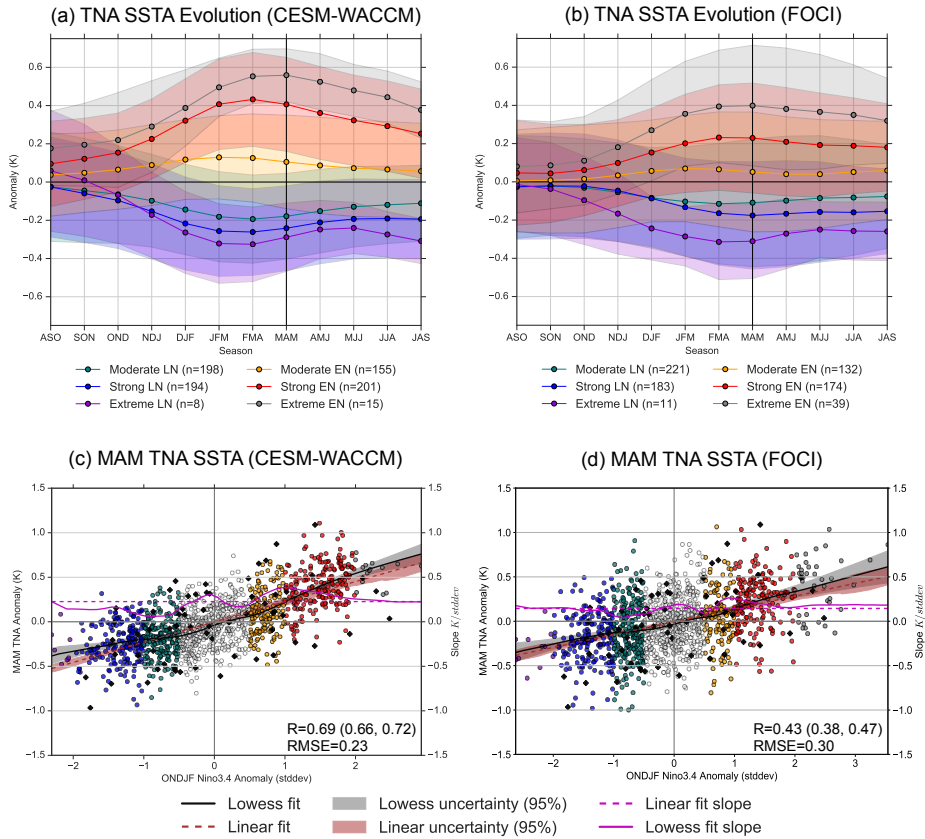
Figure 1. Tropical North Atlantic SSTAs relationships. a-b represent represents the composited seasonal evolution of the TNA SSTAs for CESM-WACCM (left) and FOCI (right) following an ENSO event. c-d show the scatter plots between the TNA SSTAs (in °C) and Niño3.4 (in stddev) for MAM for CESM-WACCM (left) and FOCI (right). The linear fit is represented by the dashed black-red line, while the LOWESS fit is represented by the solid black line (with both with a 95% confidence interval in shading). The slopes of these fits are represented by the magenta dashed and solid lines, respectively, and the right y-axis indicates the corresponding slope values. Scatter coloring represents the subsampling ranges from extreme La Niña (in purple) to extreme El Niño (in dark grey) (see labeling below Figures 1a-b). Neutral events are included in white. Results from JRA-55 (1958-2021) are shown as black diamonds, and an equivalent figure for JRA-55 can be seen in Supplementary Figure S3S10.
