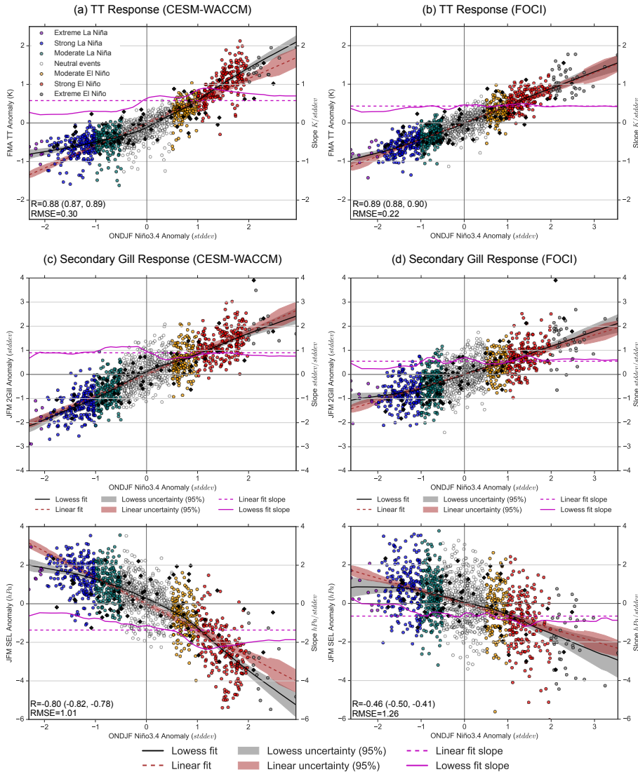
Figure 3. Relationship between the major mechanisms for the tropical/extratropical pathways and the Niño3.4 SSTAs. The Niño3.4 SSTAs is-are shown for ONDJF, while the mechanisms are shown for their peak seasons (3-month average). Scatter plot colors match those found in Figure 1c-d. Results from JRA-55 (1958-2021) are shown in black diamonds, and the corresponding seasonal evolutions are shown in Supplementary Figure 4- S7 .
