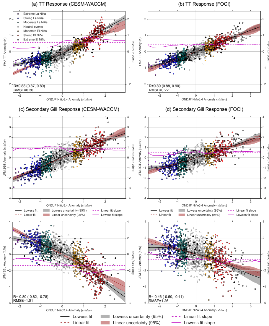
Figure 3. Relationship between the major mechanisms for the tropical/extratropical pathways and the Niño3.4 SSTs. The Niño3.4 SSTs are shown for ONDJF, while the mechanisms are shown for their peak seasons (3-month average). Scatter plot colors match those in Figure 1c-d. Results from JRA-55 (1958-2021) are shown in black diamonds, and the corresponding seasonal evolutions are shown in Supplementary Figure S7.
