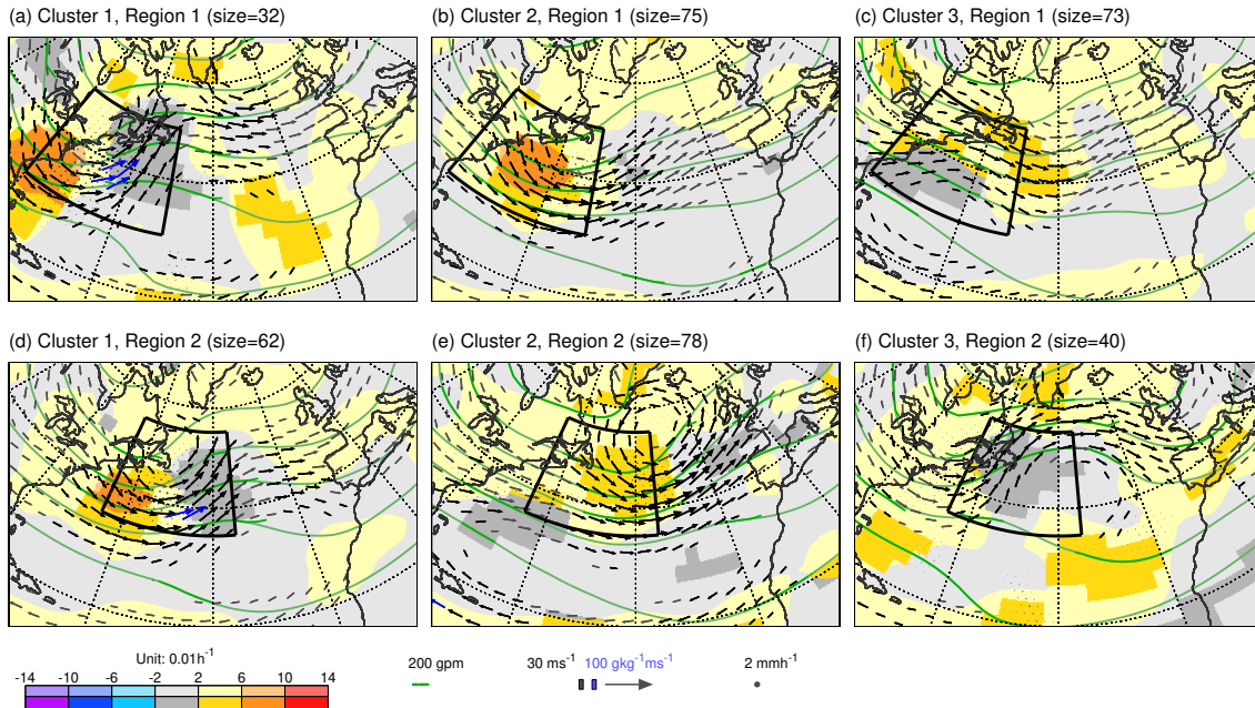
Figure 6. Means over the date/times for the three clusters obtained from K -means clustering in the first (top) and second (bottom) region on the fields of Z_{250} (contours), u_{850} and v_{850} (vectors) from ECMWF control (unperturbed) forecasts at step 0, and ensemble mean 12 h accumulated precipitation (dots) valid (or end of accumulation) at 00 and 12 UTC within the period DJF 2020/21. The two clustering regions are indicated by the black borders in each panel. Although not used in the clustering, shading shows the corresponding mean 12 h uncertainty growth rate LGR_z for Z_{250} . Vectors are coloured blue when the humidity flux at 850 hPa exceeds 100 \text{ g kg}^{-1} \text{ m s}^{-1} . More saturated shading, contours, vectors and dots indicate statistical significance at the 5% level (not accounting for autocorrelation due to the discontinuous nature of date/times in each cluster).
