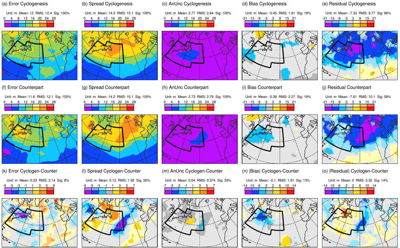
Figure 7. As Fig. 5 but separately for the cyclogenesis composite date/times (top) and the non-cyclogenesis counterpart composite date/times (middle), for forecasts that start two days prior to the cluster classifications. The bottom row shows cyclogenesis minus counterpart. Note that differences in absolute Bias and Residual are shown, so that blue (red) colours anywhere on the bottom row show where results for the cyclogenesis composite are better (worse) than for the counterpart. The union of the two clustering regions is indicated by the black border.
