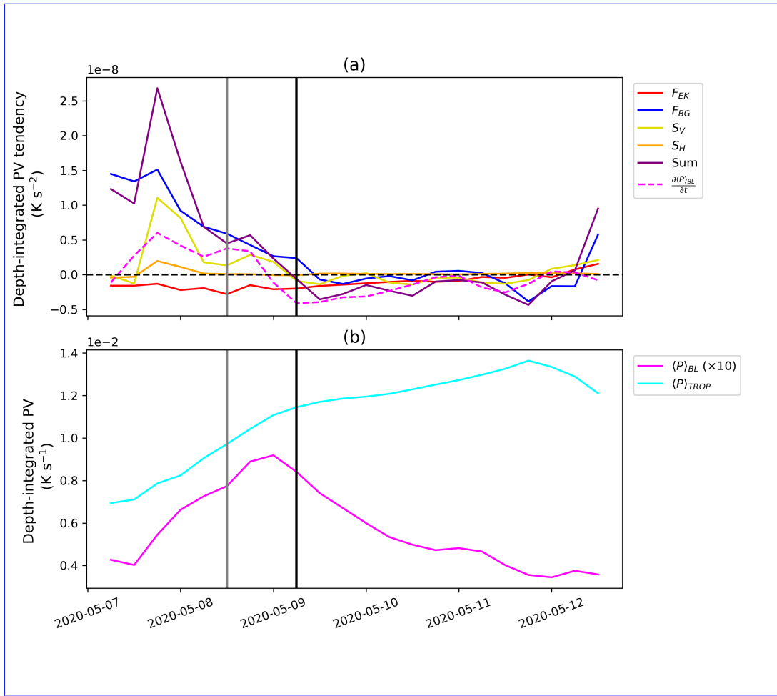
Figure 7. Time series of depth-integrated circulation-PV and tendencies associated with Cyclone A, from IFS run starting 00Z 7 May 2020, from 00Z 7 May to 12Z 12 May 2020. (a) BL depth-integrated PV tendencies ( \text{K s}^{-2} ): F_{EK} (red line), F_{BG} (blue line), S_V (yellow line), S_H (orange line), sum (purple line) and the BL depth-integrated circulation-volume-averaged PV tendency calculated explicitly (LHS of Equation 14; magenta dashed line). (b) Depth-integrated circulation-volume-averaged PV ( \text{K s}^{-1} ) in the BL and the tropospheric layer with the 330 K isentropic surface as the top of the layer. The grey and black vertical lines correspond to the time of maximum growth rate and maximum intensity.
