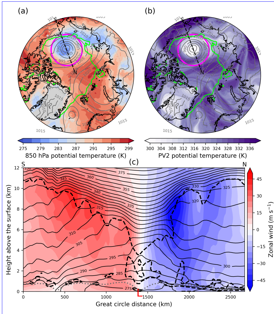
Figure 4. As in Fig. 3, but for Cyclone B from IFS run starting 00Z 25 July 2020, at 12Z 28 July 2020.
