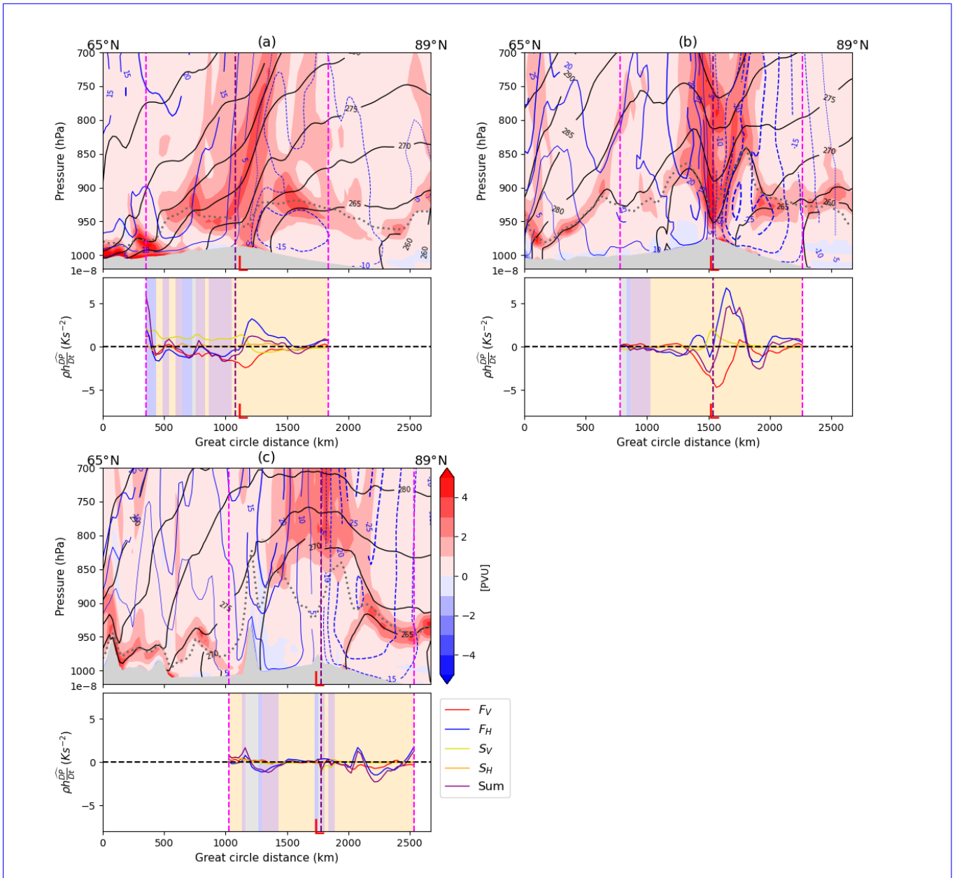
Figure 9. North-south cross-sections of Cyclone A, from IFS run starting 00Z 7 May 2020, at the longitude of the cyclone centre from 65°N to 89°N at (a) 12Z 8 May ( maximum growth rate ), (b) 06Z 9 May ( maximum intensity ), and (c) 06Z 10 May 2020 ( 24 hours after maximum intensity ). The top panels display potential vorticity (PVU; shading), potential temperature (K; black solid contours), zonal wind ( \text{m s}^{-1} ; blue contours), and the BL top (grey dotted line). Minimum mean sea level pressure along the section is marked with a red L . The bottom panels display the BL PV tendency terms (scaled to depth-integrated circulation-PV tendencies) due to friction and sensible heat fluxes, within 750 km radius of the cyclone centre . The background shading denotes the surface type: land (grey), ocean (blue; sea ice concentration < 0.15), marginal ice zone (purple; sea ice concentration > 0.15 and < 0.8), and pack ice (orange; sea ice concentration > 0.8). The vertical purple line marks the cyclone centre from TRACK, and the magenta lines mark 750 km distance from the cyclone centre. Minimum sea level pressure along the section is marked with a red L in the top and bottom panels.
