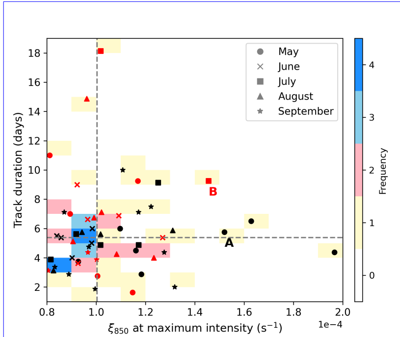
Figure 1. 2D histogram of \xi_{850} at maximum intensity (x-axis) and track duration (y-axis) of summer 2020 Arctic cyclones from ERA5. Black and red markers refer to low-level and upper-level dominant cyclones respectively, as diagnosed by the thermal Rossby number, Ro_T , from the modified cyclone phase space (Section 2.4) at the time of maximum growth rate. The shading illustrates the number of cyclones that populate a region of the histogram space. The median values of \xi_{850} at maximum intensity and track duration are demonstrated by the grey dashed lines. Cyclone cases A and B are annotated with the respective letter to the bottom right of the marker.
