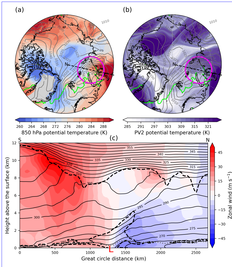
Figure 3. Cyclone A at 18Z 8 May 2020 from IFS run starting 00Z 7 May 2020. (a) 850 hPa potential temperature (K; shading), (b) potential temperature on the PV2 surface (K; shading), overlain with mean sea level pressure (hPa; grey contours), the sea ice edge (0.15 sea ice concentration; green contour). The magenta circle marks the 750 km radius about the cyclone centre as determined by TRACK. The black dashed lines mark the north-south cross-section taken at the longitude of the cyclone centre from S (65°N) to N (89°N). (c) Vertical cross-sections linearly interpolated at 100 points between S and N of zonal wind ( \text{m s}^{-1} ; shading), potential temperature (K; black solid contours), 2 PVU contour (black dashed line) and BL top (grey dotted line). Minimum mean sea level pressure is marked with a red L.
