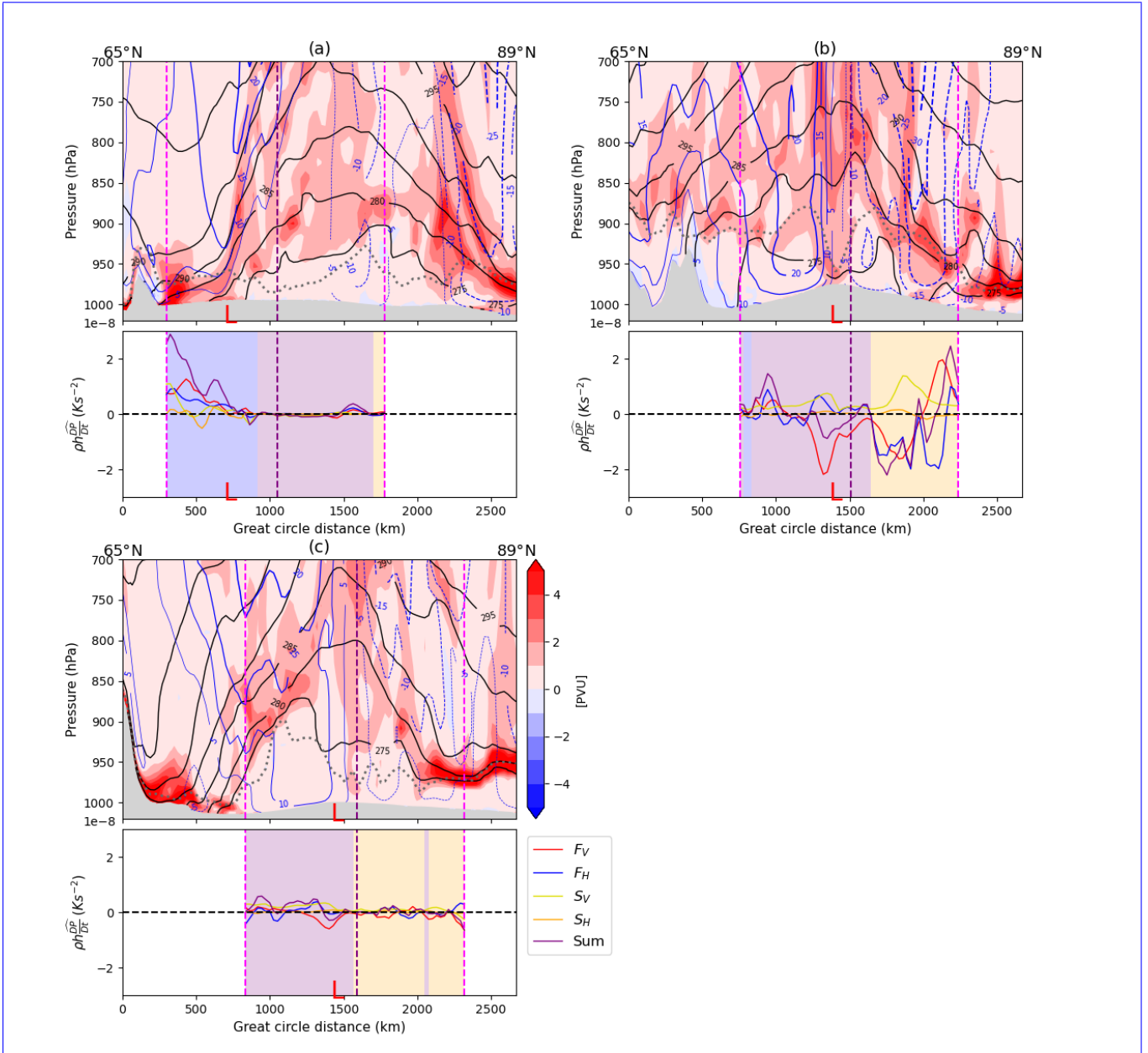
Figure 10. As in Fig. 10, but for Cyclone B, from IFS run starting 00Z 25 July 2020, at (a) 18Z 26 July ( maximum growth rate ), (b) 12Z 28 July ( maximum intensity ), (c) 12Z 31 July ( 72 hours after maximum intensity ).
