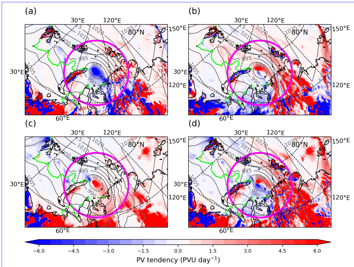
Figure 5. BL depth-averaged PV tendencies from Equation (11) for Cyclone A at 18Z 8 May 2020 ( 6 hours before maximum growth rate ) from IFS run starting 00Z 7 May 2020. (a) F_{EK} , (b) F_{BG} , (c) S_V , and (d) the sum of F_{EK} , F_{BG} , S_V and S_H (PVU day -1 ; shading), mean sea level pressure (hPa; grey contours) and the sea ice edge (0.15 sea ice concentration; green contour). The magenta circle marks 750 km from the cyclone centre.
