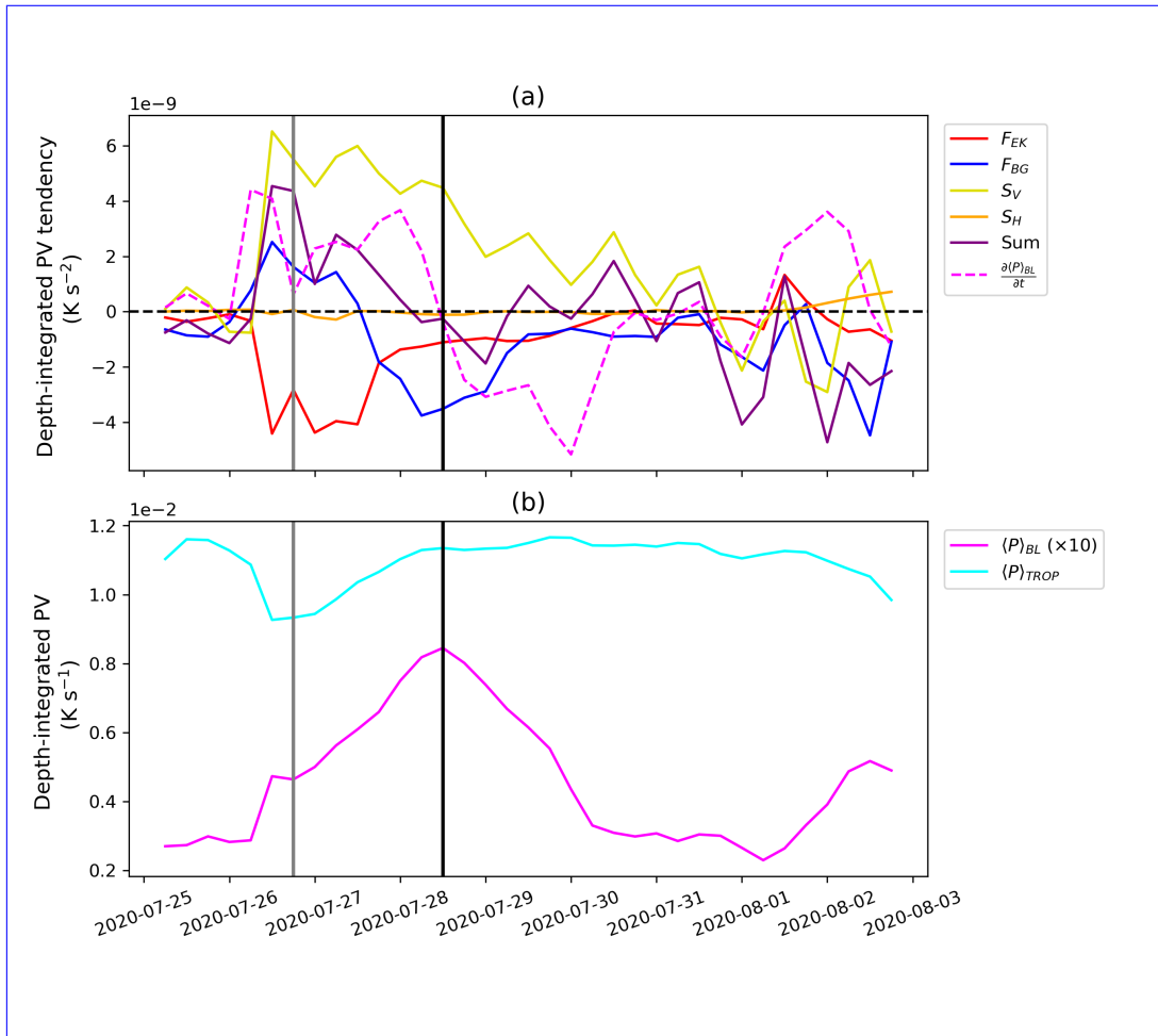
Figure 8. As in Fig. 7, but for Cyclone B from IFS run starting 00Z 25 July 2020, from 00Z 25 July to 00Z 2 August. Note that the y-scale in (a) is an order of magnitude smaller than that of Fig. 7a.
