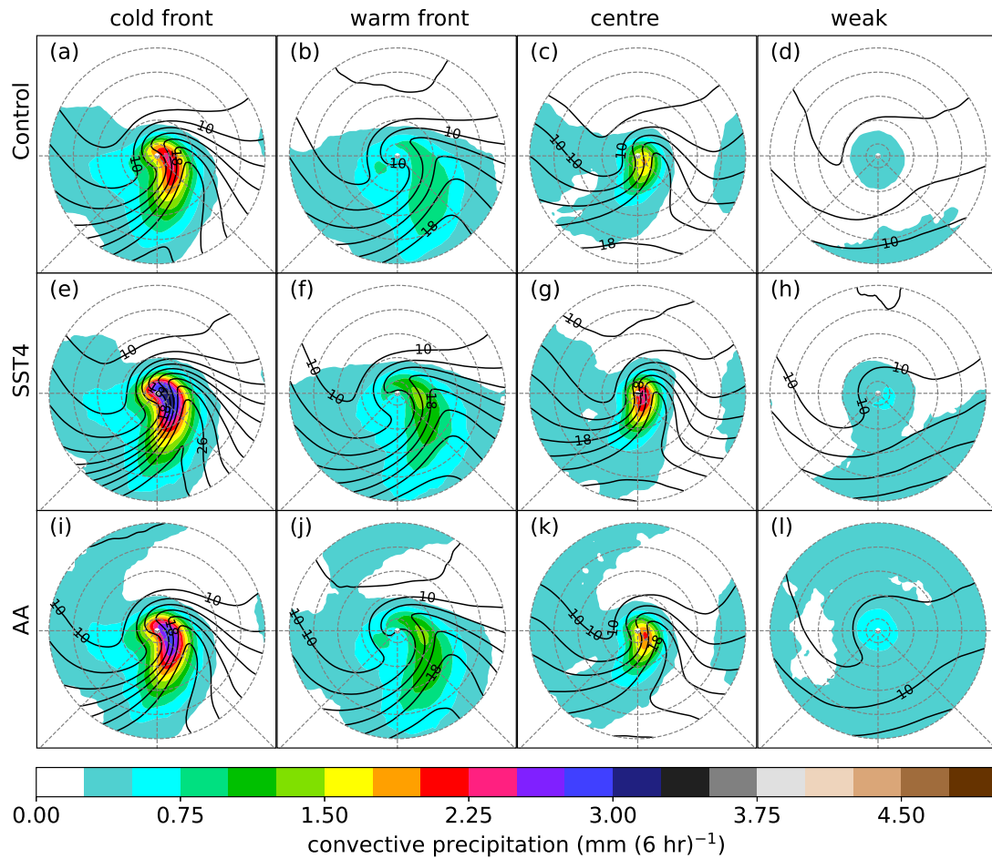
Figure 7. Composite mean of the convective precipitation (shading, mm / 6 hr) and the total column water vapour (black contours, every 2 g kg -1 ) 12 hours before the time of the maximum vorticity. Different columns show different clusters and different rows show different experiments.
