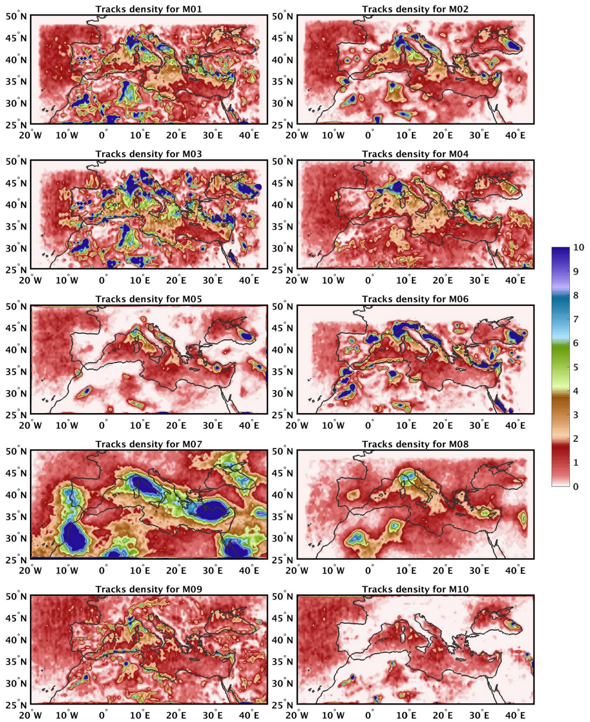
Figure 65 Spatial density of cyclone tracks for each CDTM. Spatial density expresses the average count of track points per year within a circular area with a radius of 0.5° .
