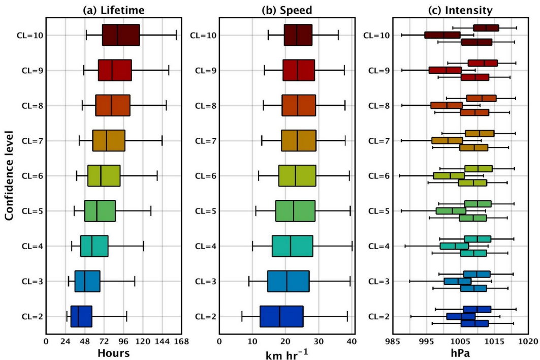
Figure 142 as in Fig. 7 but for composite tracks of different confidence levels (CL) and an overlapping criterion of 12 hours.
