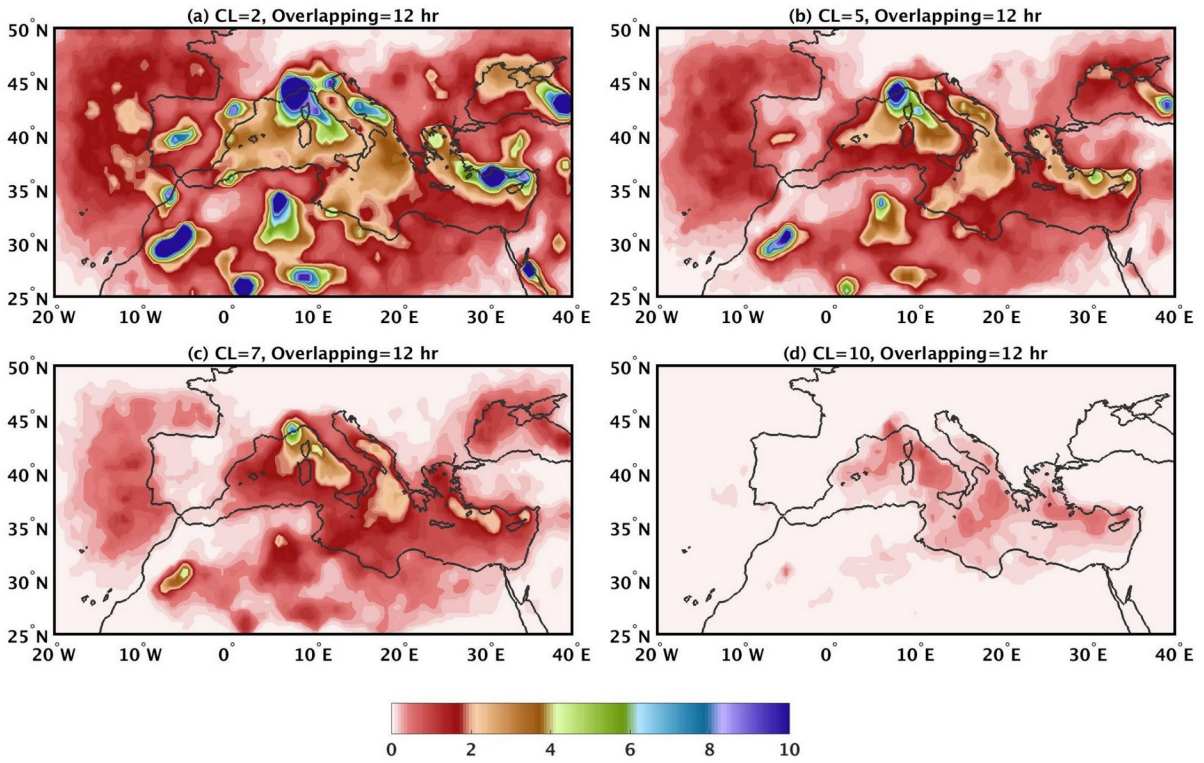
Figure 131 Spatial density of cyclone tracks for composite tracks of four different confidence levels (CL) and an overlapping criterion of 12 hours. Spatial density expresses the average count of track points per year within a circular area with a radius of 0.5^\circ .
