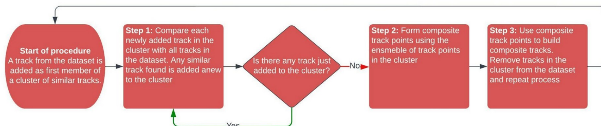
175 Figure 1 Flowchart of the procedure that builds composite tracks
