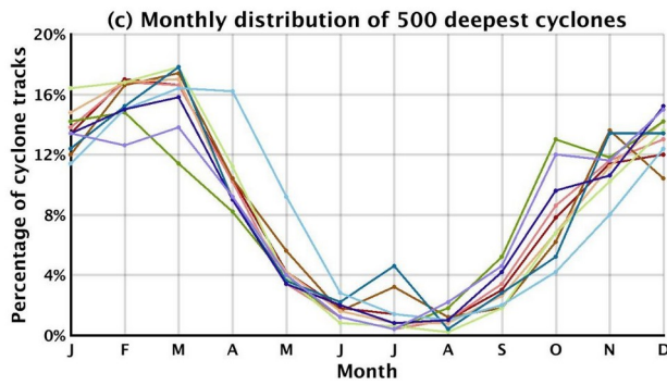
460 Figure 5 a Number of cyclone tracks per year for each CDTM b Average monthly distribution of cyclone tracks occurrence for each CDTM with respect to the total number of cyclone tracks per year c Monthly distribution of 500 deepest cyclones for each CDTM.
