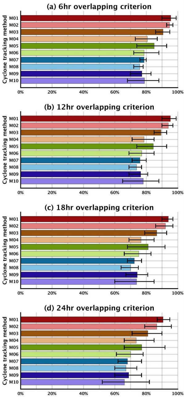
520 | Figure 87 Bars depict the average similarity score when comparing each of the 10 CDTMs to the five datasets of subjectively tracked cyclones. Minimum and maximum scores are depicted by whiskers in black colors. Each of the four panels presents similarity scores for different overlapping criteria.
