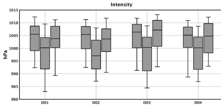
925 Figure B2 Boxplots showing the distribution of cyclone intensities -measured by core MSLP- for each 930 dataset of subjectively tracked cyclones . Three boxplots are shown for each dataset: the lower one shows the distribution of MSLP at cyclone first track points, the middle one shows the distribution of MSLP at the time of lowest MSLP and the upper one shows the distribution of MSLP at cyclone last track points. For all boxplots, the boxes depict the 25th, 50th and 75th percentiles, while whiskers depict the 5th and 95th percentiles.
