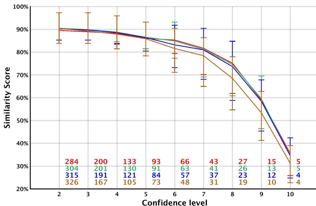
565 Figure 109 Similarity scores per confidence level between composite tracks and five datasets of subjectively tracked cyclones. Similarity scores are defined as the number of similar tracks in two datasets divided by the number of subjectively tracked cyclones tracks in the smallest dataset. Scores are produced for composite tracks, built with four overlapping criteria of 6 (in red), 12 (in green), 18 (in blue) and 24 hours (in brown). Lines show averages and whiskers show minimum and maximum similarity scores. Numbers show the average number of cyclones per year for each confidence level and overlapping criterion.
