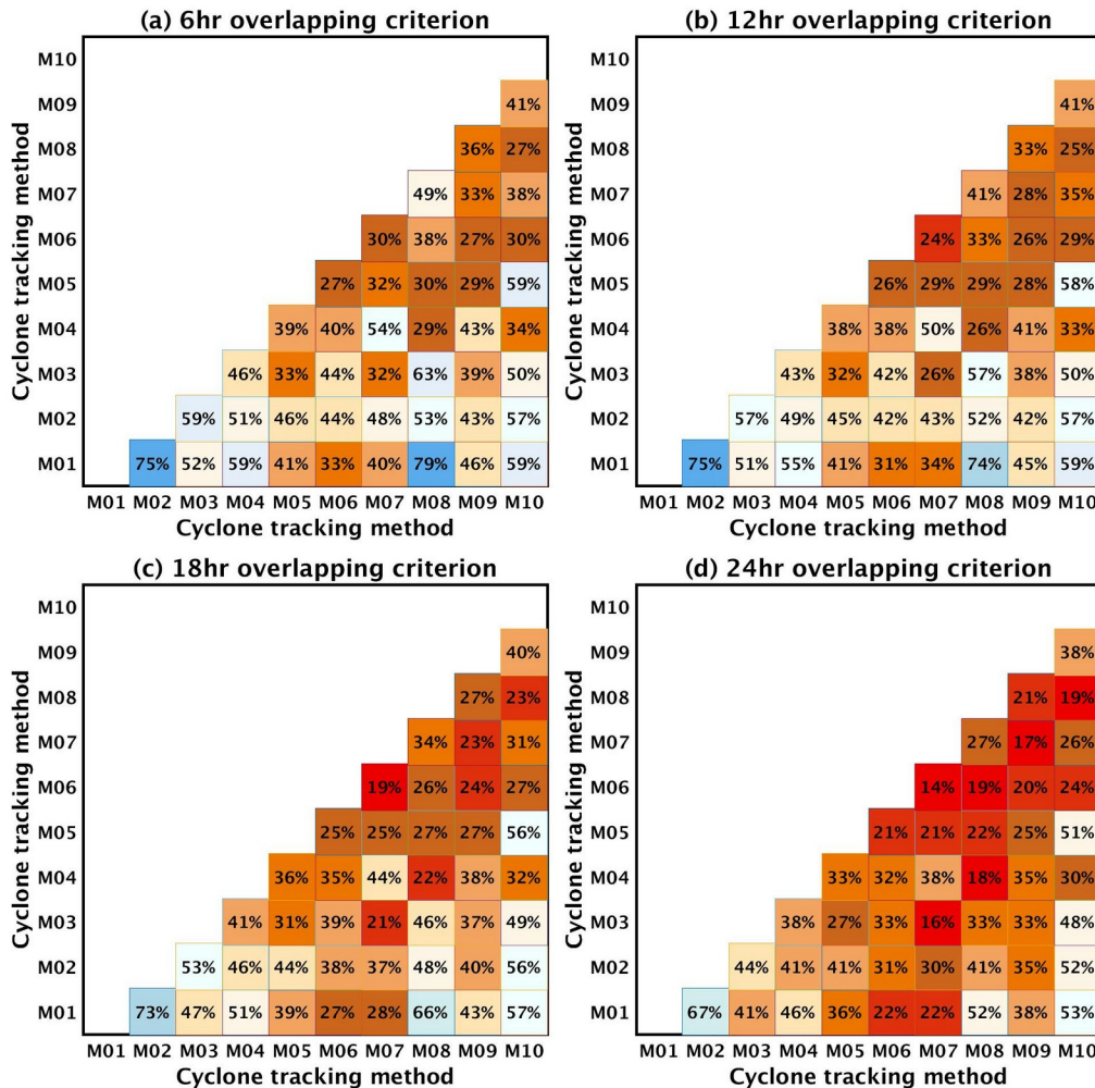
525 | Figure 98 Similarity scores between the 10 CDTMs, defined as the number of similar tracks in two datasets divided by the number of tracks in the smallest dataset. Each of the four panels presents similarity scores for different overlapping criteria.
