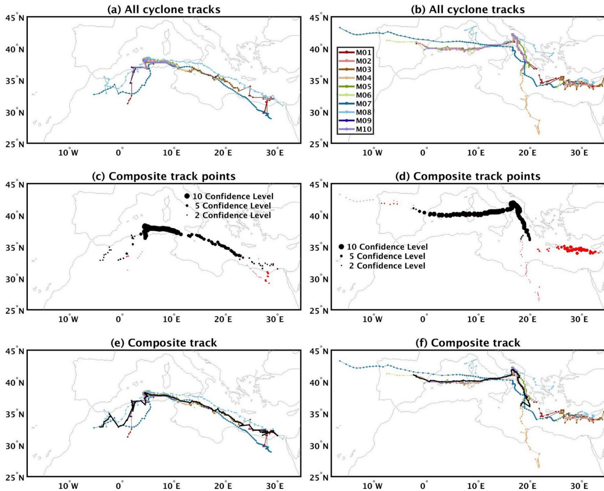
Figure 2 a Step 1 of the method (see text): similar cyclone tracks that have been reproduced by 10 different CDTMs for the cycloneexemplary case of November 2020. c Step 2: Composite track points produced by the combination of the tracks in a . Black (red) color marks the composite track points that have (not) been eventually used for composite tracks. The size of the dots depicts the confidence level of the composite track points. e Step 3: as in a , but overlaying the composite track (in black line). b, d, and f, and h as in a, c, and e, and g respectively but for a second cycloneexemplary case that took place in November 2018.
