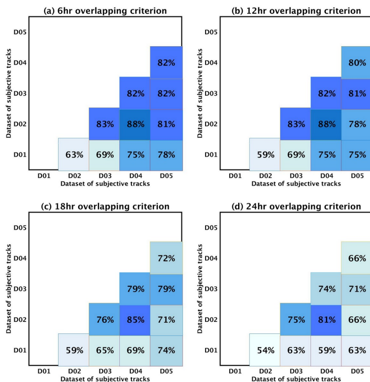
360 Figure 43 Similarly scores among the five datasets of subjectively tracked cyclones (D01, D02., D05), defined as the number of similar tracks in two datasets divided by the number of tracks in the smallest dataset. Each of the four panels presents similarity scores for different overlapping criteria.
