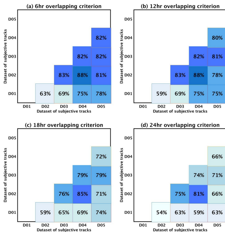
345 Figure 4 Similarly scores among the five datasets of subjectively tracked cyclones (D01, D02..., D05), defined as the number of similar tracks in two datasets divided by the number of tracks in the smallest dataset. Each of the four panels presents similarity scores for different overlapping criteria.
