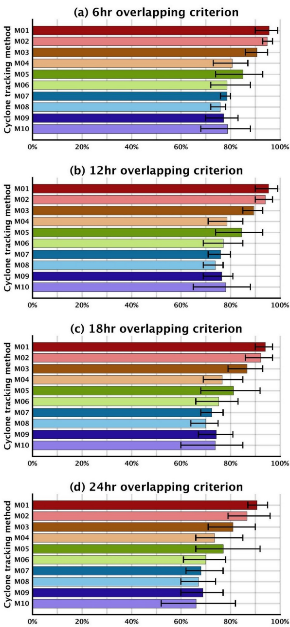
Figure 8 Bars depict the average similarity score when comparing each of the 10 CDTMs to the five datasets of subjectively tracked cyclones. Minimum and maximum scores are depicted by whiskers in black colors. Each of the four panels presents similarity scores for different overlapping criteria.
