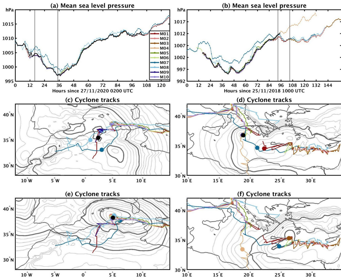
265 Figure 3 a The MSLP evolution of cyclone tracks for the cyclone case (in coloured lines) of November 2020, shown in Fig. 2a. MSLP of the composite track is overlaid in black color. c MSLP field in gray contours at the time of the first vertical line in panel a (1 hPa contour intervals where thick contours are drawn every 5 hPa starting from 1000 hPa). Tracks from different CDTMs are shown in coloured lines. Colored dots depict the location of cyclone centers and the black dot depicts the location of the corresponding composite track point. e As in c but for the time of the second vertical line in panel a. b, d, and f as in a, c, and e but for a second cyclone case that took place in November 2018 shown in Fig. 2b.
