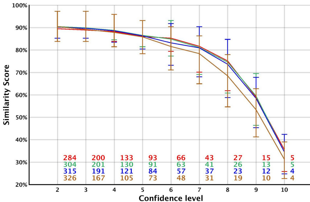
Figure 10 Similarity scores per confidence level between composite tracks and five datasets of subjectively tracked cyclones. Similarity scores are defined as the number of similar tracks in two datasets divided by the number of subjectively tracked cyclones. Scores are produced for composite tracks, built with four overlapping criteria of 6 (in red), 12 (in green), 18 (in blue) and 24 hours (in brown). Lines show averages and whiskers show minimum and maximum similarity scores. Numbers show the average number of cyclones per year for each confidence level and overlapping criterion. 520
