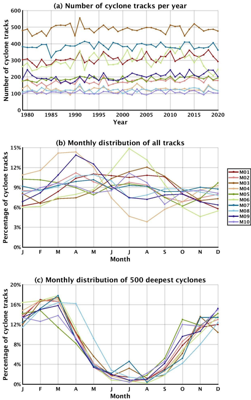
415 Figure 5 a Number of cyclone tracks per year for each CDTM b Average monthly distribution of cyclone tracks occurrence for each CDTM with respect to the total number of cyclone tracks per year c Monthly distribution of 500 deepest cyclones for each CDTM.
