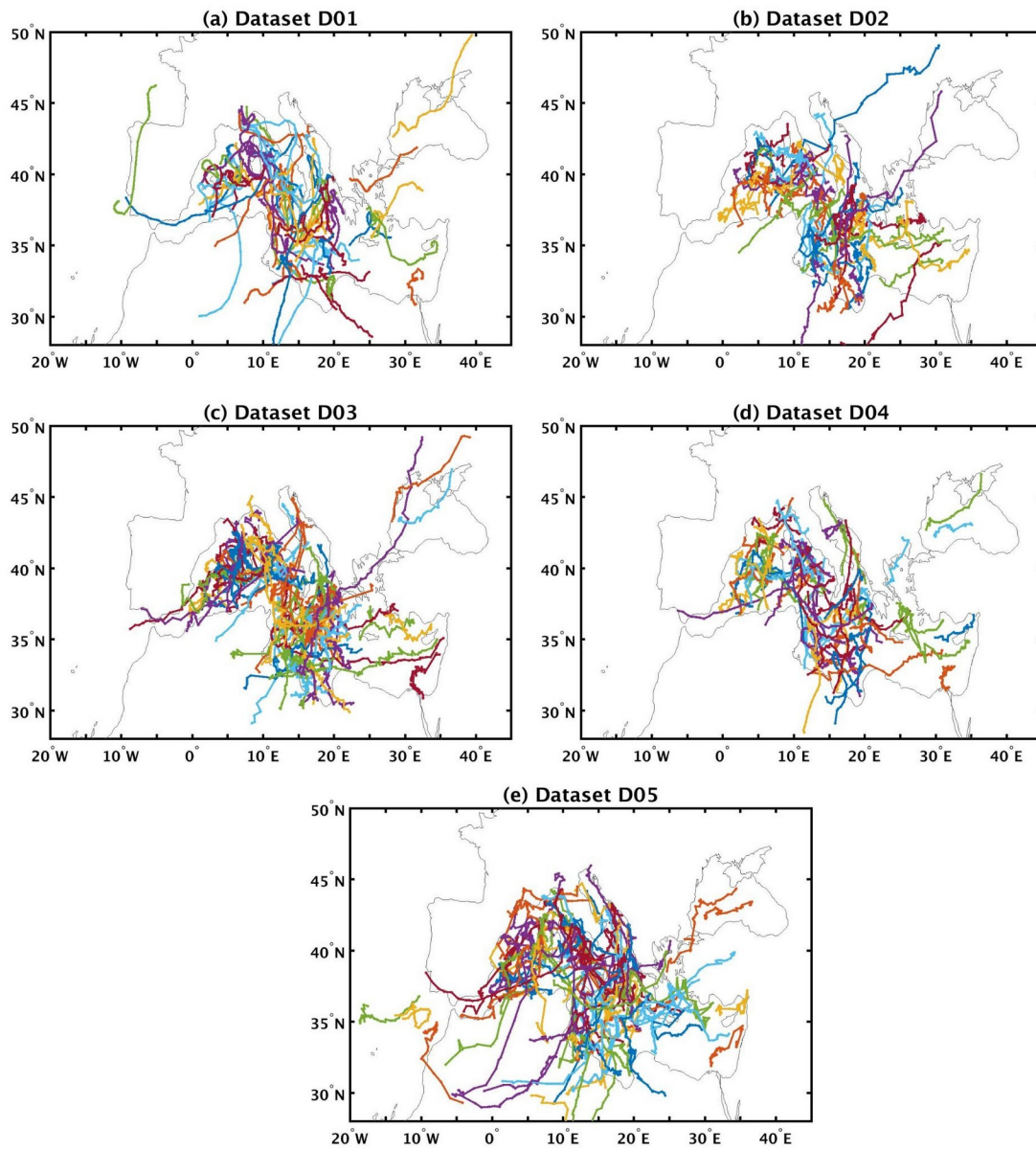
860 Figure B1 Tracks in the five datasets of subjectively tracked cyclones. Colors are produced randomly to ease readability.
