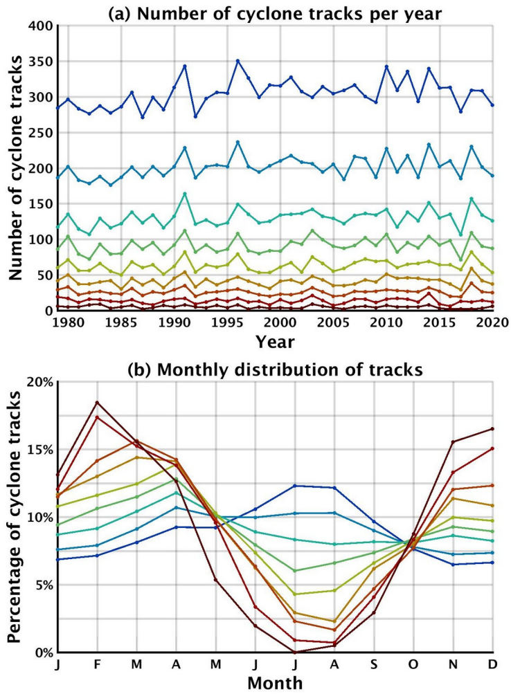
605 Figure 12 a Number of composite cyclone tracks per year when using different confidence levels and an overlapping criterion of 12 hours. Highest number of tracks (line in dark blue) corresponds to the dataset with confidence level of 2 and lowest number of tracks (in dark brown) to the dataset with confidence level of 10 b Seasonal cyclone of composite cyclone tracks.
