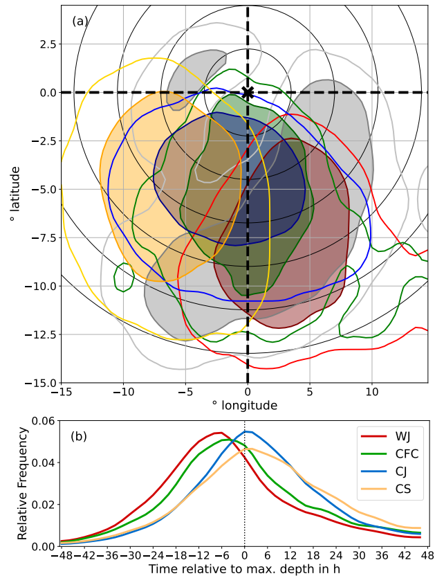
Figure 7. Occurrence of the identified mesoscale wind features (a) relative to the cyclone centre including NF in grey and (b) relative to the cyclone life cycle. The contours in (a) show the area with most feature occurrences, including 25% (filled contours) and 50% (outer contours) of the detected features. Black circles show the distance to the cyclone centre in 250 km increments using 50°N as a reference latitude .
