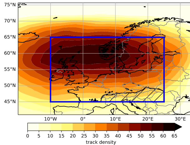
Figure 2. Track-Cyclone track density in number of all-cyclones per year per (° lat) 2 within the examined time period (2000–2019). The blue box represents the study area, with hatching indicating excluded areas.
