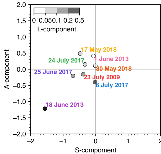
Figure 3. SAL diagrams of daily accumulated total precipitation in COSMO simulations compared to IMERG observations over the analysis domain for all eight analyzed cases. The S, A, L components evaluate the differences in structure, amplitude, and location of the events, respectively. Values near zero signal a perfect match with observations.
