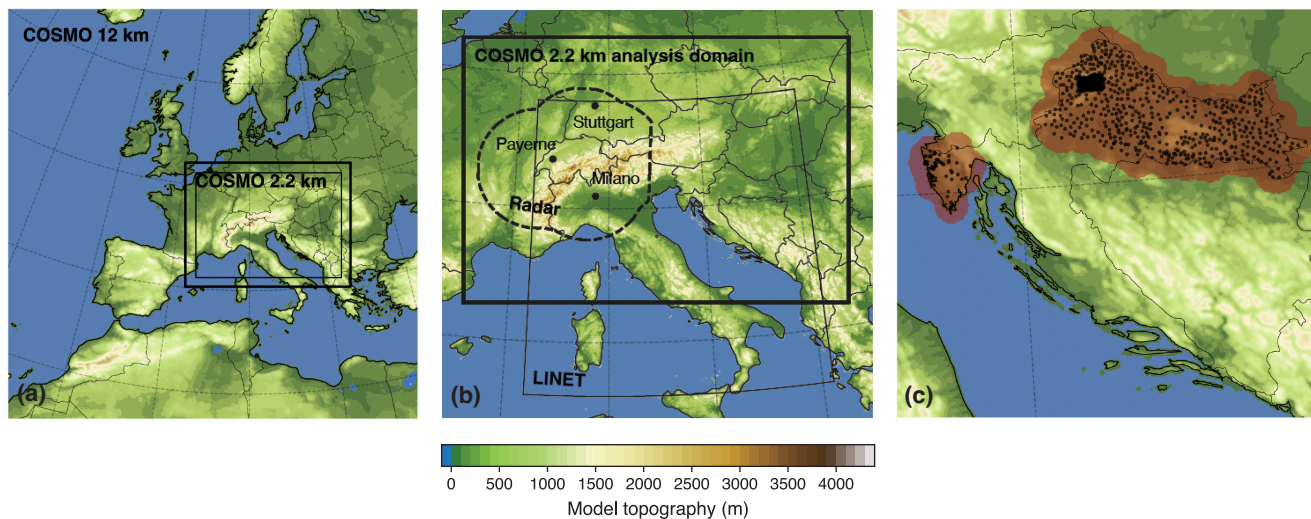
Figure 1. COSMO model topography, analysis domains, and observational coverage. (a) Computational domains for the simulations with 12 and 2.2 km grid spacings. The innermost box denotes the analysis domain. (b) COSMO 2.2 km analysis domain (thick solid line), LINET lightning observations (thin line), radar-based hail observations (dashed line). Black dots represent the four sounding stations used in this study: Payerne, Milano and Stuttgart. (c) Available hailpad measurements over Croatia (black dots). A dense hailpad polygon (150 hailpads aligned with a distance of around 2 km between hailpads) is located in the northwestern part of Croatia. The red-shaded area indicates the region used to evaluate hail simulated by COSMO HAILCAST.
