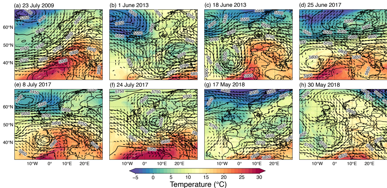
Figure 2. Synoptic overview of the eight case studies cases considered in this paper. Panels show geopotential height at 500 hPa (m, black contours), temperature at 850 hPa (°C, shaded), and wind barbs at 500 hPa obtained from ERA5 reanalysis at 12 UTC on the day when the respective case was observed.
