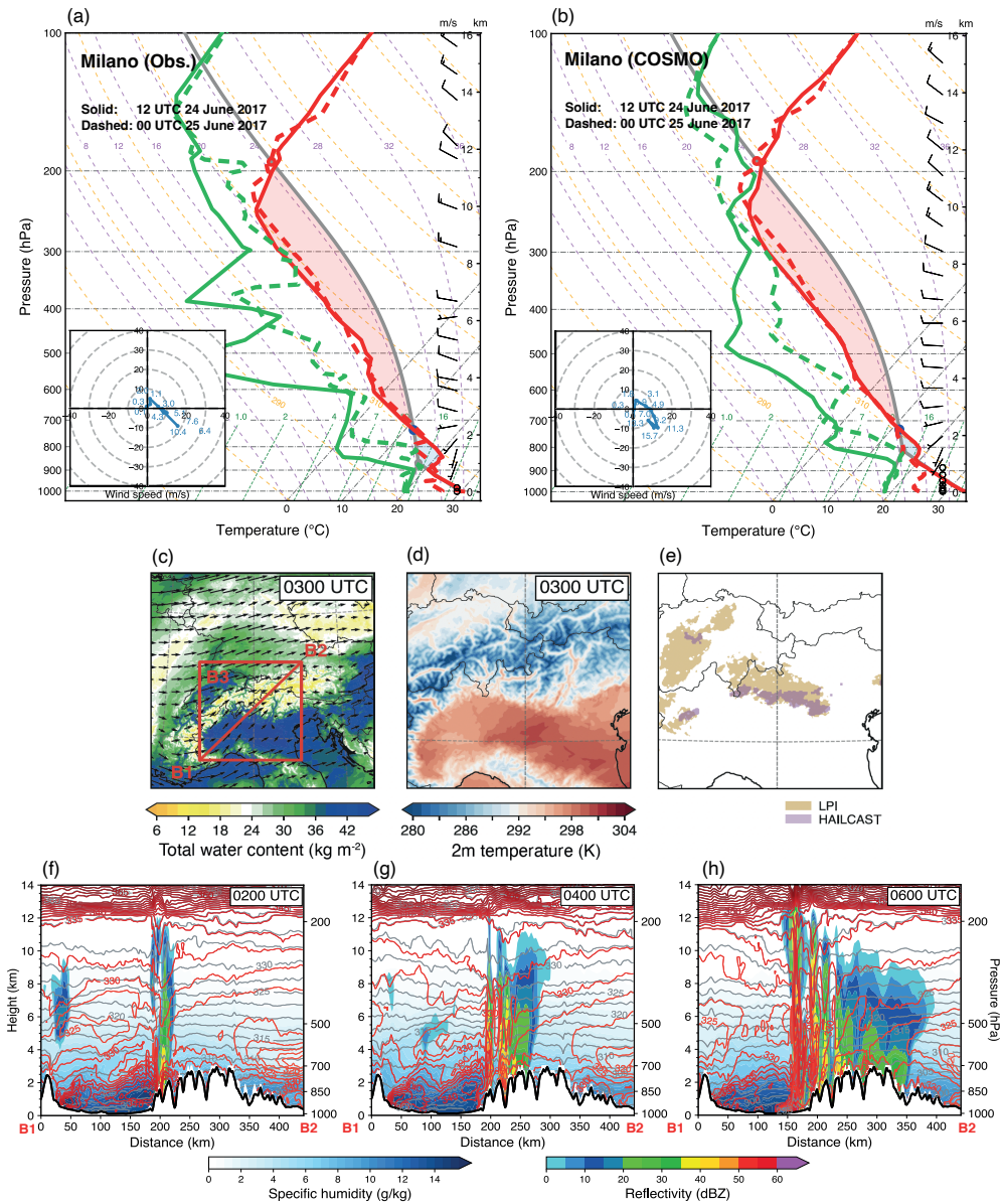
Figure 11. Similar as As in Fig. 10, but for the case of 25 June 2017. (a) Sounding observations and (b) COSMO extracted profiles at Milano station at 12 UTC on 24 June 2017 (solid lines) and 00 UTC on 25 June 2017 (dashed lines). (c) COSMO simulated total water content and vertically integrated water flux vectors, (d) 2m temperature at 03 UTC on 25 June 2017, and (e) footprints of LPI and HAILCAST obtained between 03 and 04 UTC are shaded in yellow and purple, respectively. The red box B3 in (c) indicates the zoomed subdomain shown in (d-e). (f-h) Vertical cross-sections of potential temperature (gray contours), equivalent potential temperature (red contours), specific humidity (blue shaded), and simulated reflectivity (colour shaded) along the red transect B1-B2 at 02, 04 and 06 UTC on 25 June 2017.
