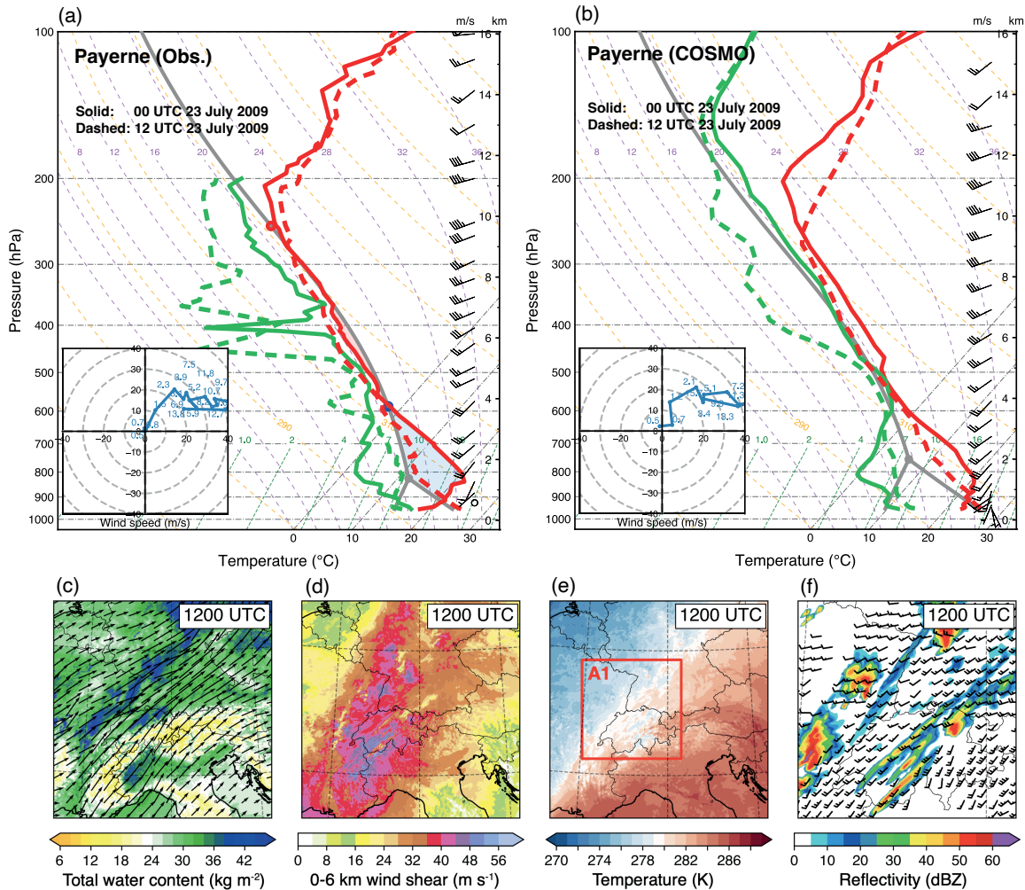
Figure 10. Detailed characteristics of the case 23 July 2009. Thermodynamic skew-T \log -P \log -p diagrams of (a) sounding observations and (b) COSMO extracted profiles at Payerne station at 00 (solid) and 12 UTC (dashed). Red and green lines represent the temperature and dew-point temperature profiles, respectively. Corresponding wind hodographs, shown in the bottom left corner, are obtained for 12 UTC on 23 July 2009. COSMO simulated (c) COSMO-simulated total water content and vertically integrated water flux vectors, (d) 0-6 km bulk wind shear, (e) temperature at 700 hPa, and (f) simulated reflectivity and wind barbs at 1 km above ground level at 12 UTC on 23 July 2009. The red box A1 indicates the zoomed subdomain shown in (f).
