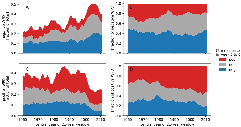
Figure 8. Left column: Prevalence of West Pacific Dipole phases over time (WPD index in week -3 to 0), as colored by the resulting Western European t2m response in week 3 to 6. Right column: Presented as fraction of the WPD phase itself, namely responses following negative WPD (B) and responses following positive WPD (D). Like in Fig. 4, tercile thresholds for WPD are determined over the entire dataset from 1950-2021, and tercile thresholds for t2m are re-computed in each window. A) Count of positive WPD phases and its resulting t2m responses in a moving window of 21 summer seasons. Positive WPD phases are recorded when the west Pacific Dipole index in week -3 to 0 is in its upper tercile class (thresholds are determined over entire dataset, from 1950-2021). The total count is subdivided into positive WPD phases resulting in negative, neutral or positive t2m anomalies in week 3 to 6 (respectively: blue, grey and red). Tercile thresholds for t2m are re-computed in each window (as in Fig. 4). B) As panel A, but presented as a fraction of the total count.
