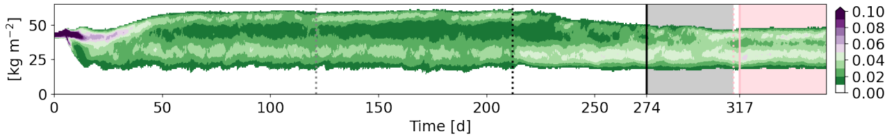
Figure 1. Evolution of the frequency density distribution of precipitable water in the equatorial belt between 20°N/S over a successive set of aquaplanet and aquachannel simulations including P13 and P5 in Table 1. The gray dotted line indicates when the horizontal grid spacing is reduced from 40 km to 26 km, the black dotted line from 26 km to 13 km and the pink dotted line from 13 km to 5 km. The solid lines indicate when the analysis periods of 40 days each begin. Colored shading in the background indicates the analysis period.
