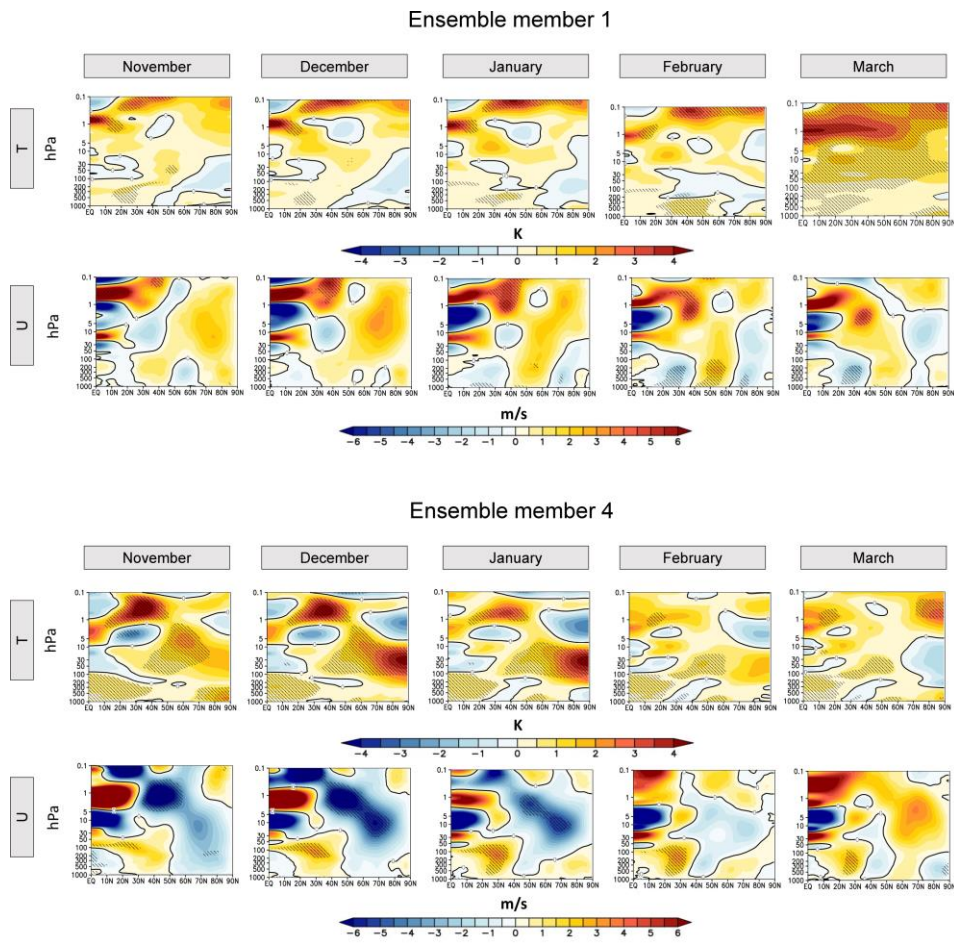
477 Figure 5: Long-term response (based on MLR) to the solar cycle of the zonal-mean temperature (first row) and the 478 zonal-mean zonal wind (second row) (hatched regions mark the 95% level of significance) in the two ensemble 479 members EM1 (top panels) and EM4 (bottom panels) in the NH during the boreal winter season. All results have been 480 scaled to 180 SSN.
