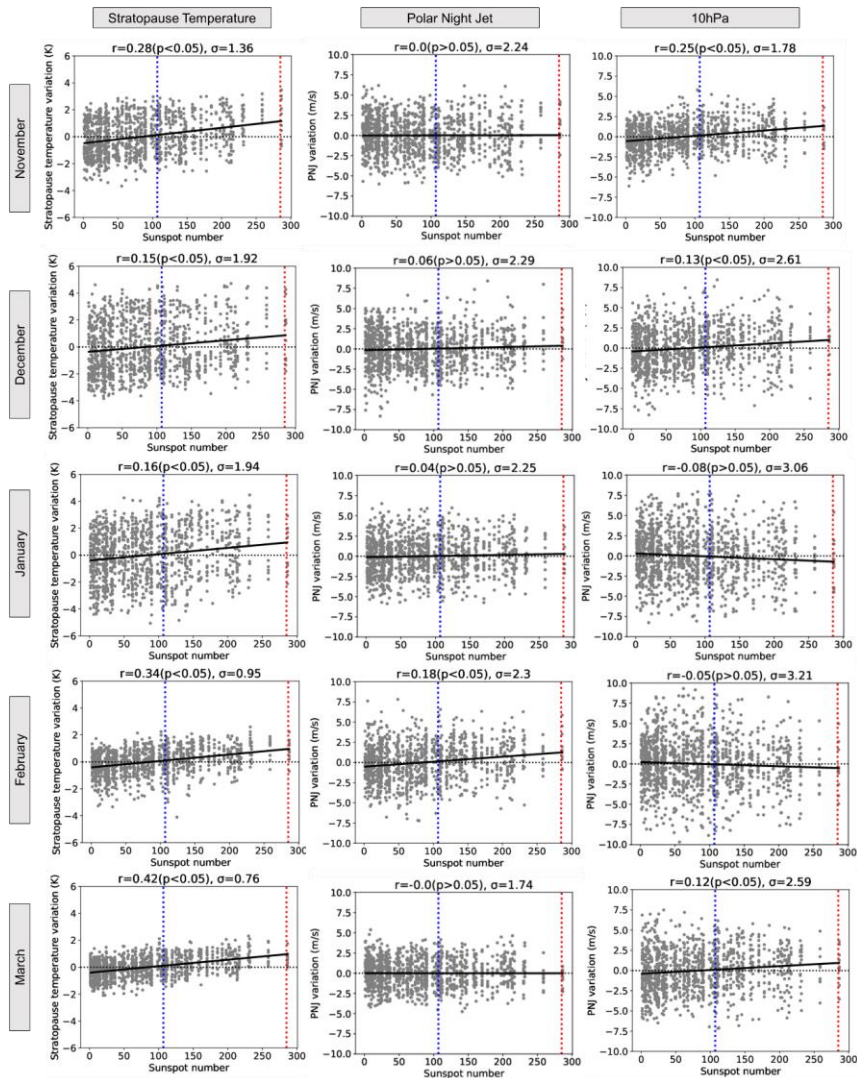
363 Figure 3: Scatter diagram of the stratopause temperature (left column), PNJ (middle column) and zonal-mean zonal 364 wind averaged over 55°N – 65°N at 10 hPa (right column) variations vs. SSN. The numbers given in the headings 365 show the correlation coefficients ( r ), their statistical significance ( p < 0.05 : significant correlation, or p > 0.05 : 366 insignificant correlation), and the overall variation ( \sigma ). The dotted blue and red lines indicate the SSN at solar cycle 367 maximum for SC14 and SC19 (the weakest/strongest solar cycles considered in the simulations). 368 369
