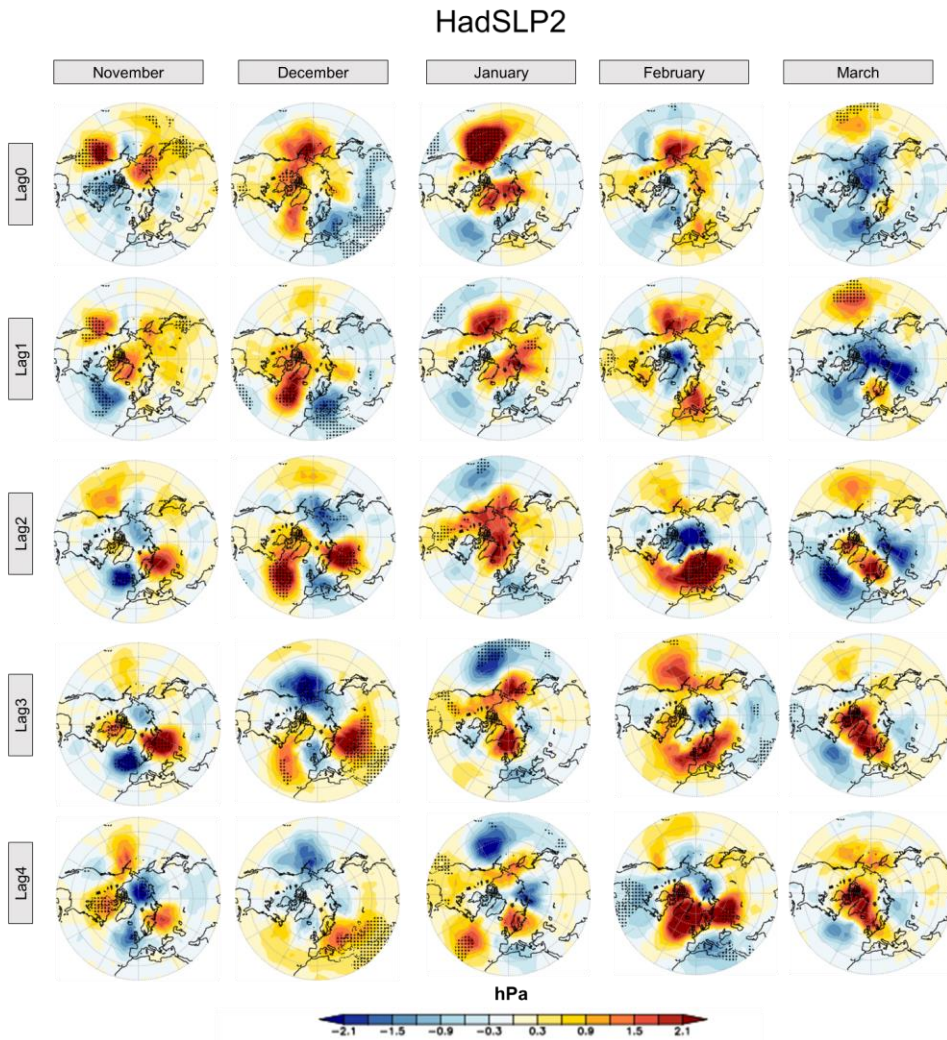
510 Figure 6: The (lagged) response of mean sea level pressure (MSLP) to the solar cycle in the NH during the boreal 511 winter season for the HadSLP2 dataset (dotted regions mark the 95% level of significance). Columns denote the 512 individual months of the winter season; rows indicate the lag of the MSLP time series with respect to the solar forcing 513 time series.
