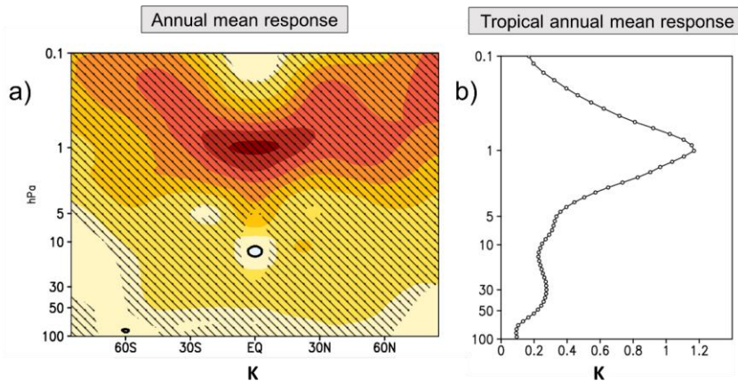
296 Figure 2: Long-term annual ensemble mean response based on MLR analysis of the zonal-mean temperature (in K) 297 to the solar cycle in the middle atmosphere as a function of height and latitude (hatched regions mark the 95% level 298 of significance) (a), and the annual mean tropical (25°S – 25°N) temperature response (in K). 299
