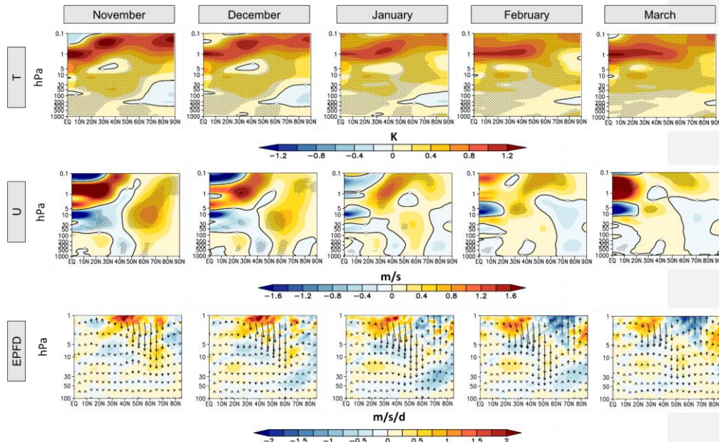
430 Figure 4: The ensemble mean long-term response (based on MLR) to the solar cycle of the zonal-mean temperature 431 (first row), zonal-mean zonal wind (second row) (hatched regions mark the 95% level of significance), and the EPF 432 (vectors) and the divergence of the EPF (EPFD, colors) in the NH during the boreal winter season. All results have 433 been scaled to 180 SSN.
